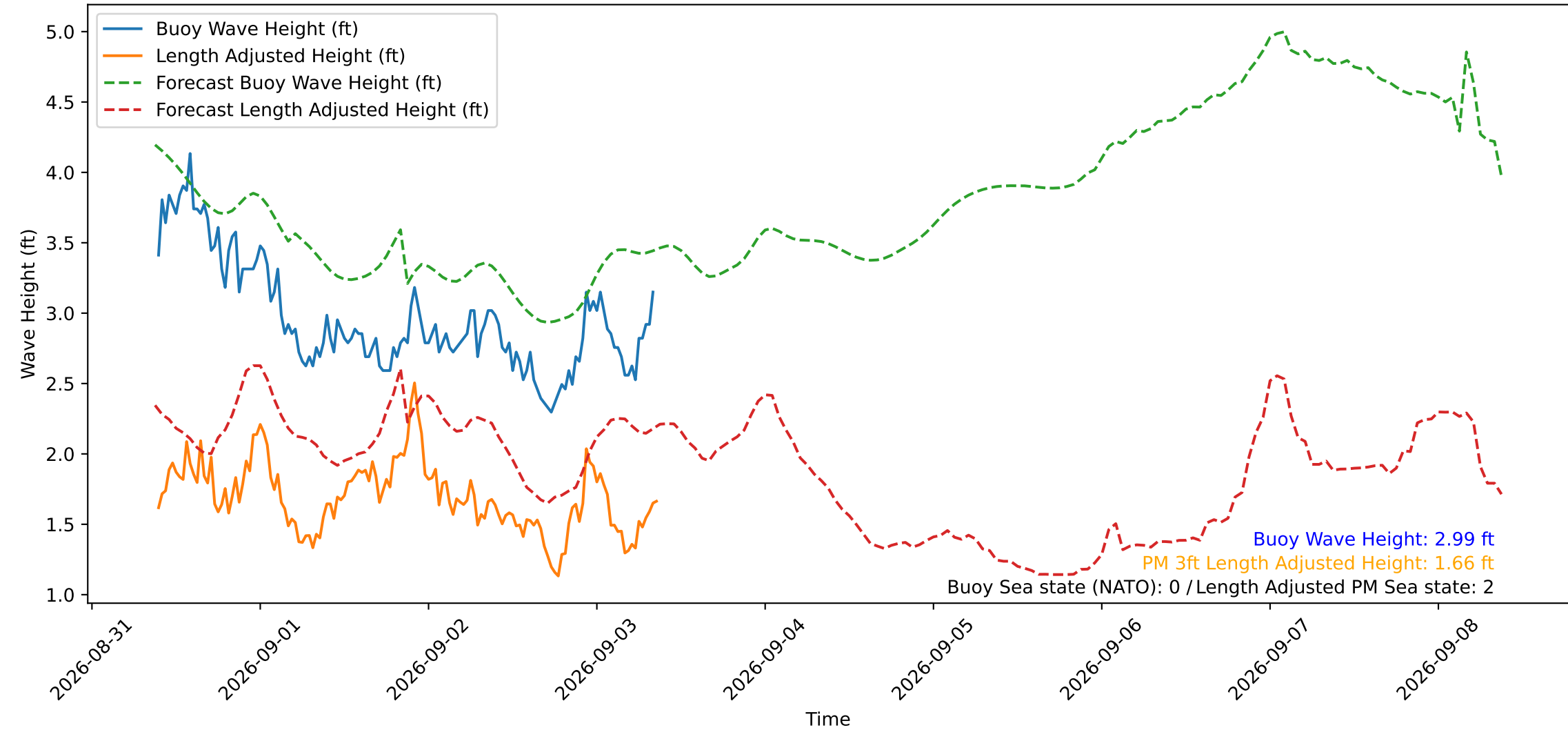
Wave Heights over Time for Red Beach at 2026-09-03 09:10:50
