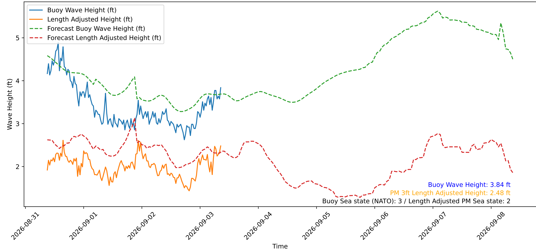
Wave Heights over Time for Oceanside Harbor at 2026-09-03 09:10:30
