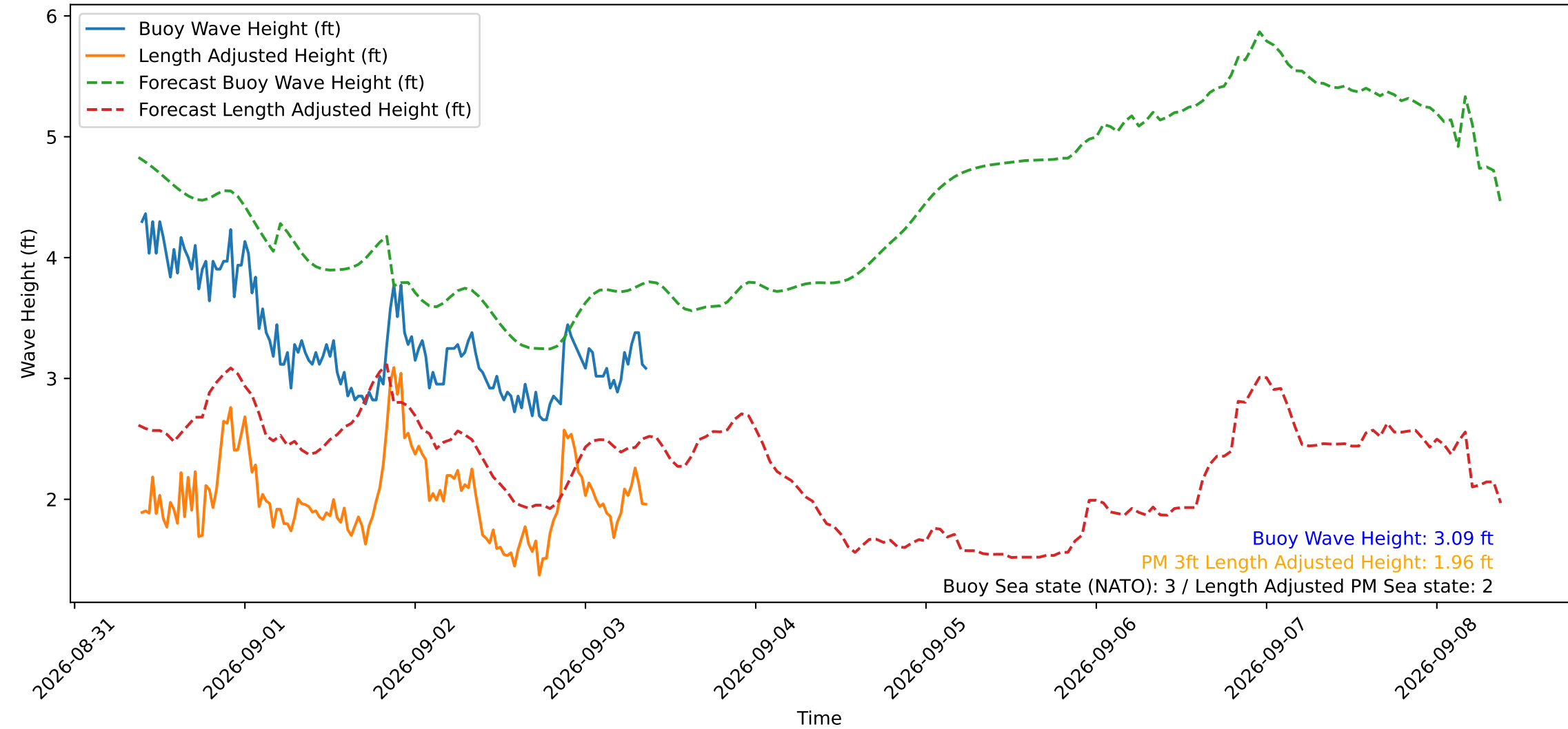
Wave Heights over Time for Green Beach at 2026-09-03 09:11:13
