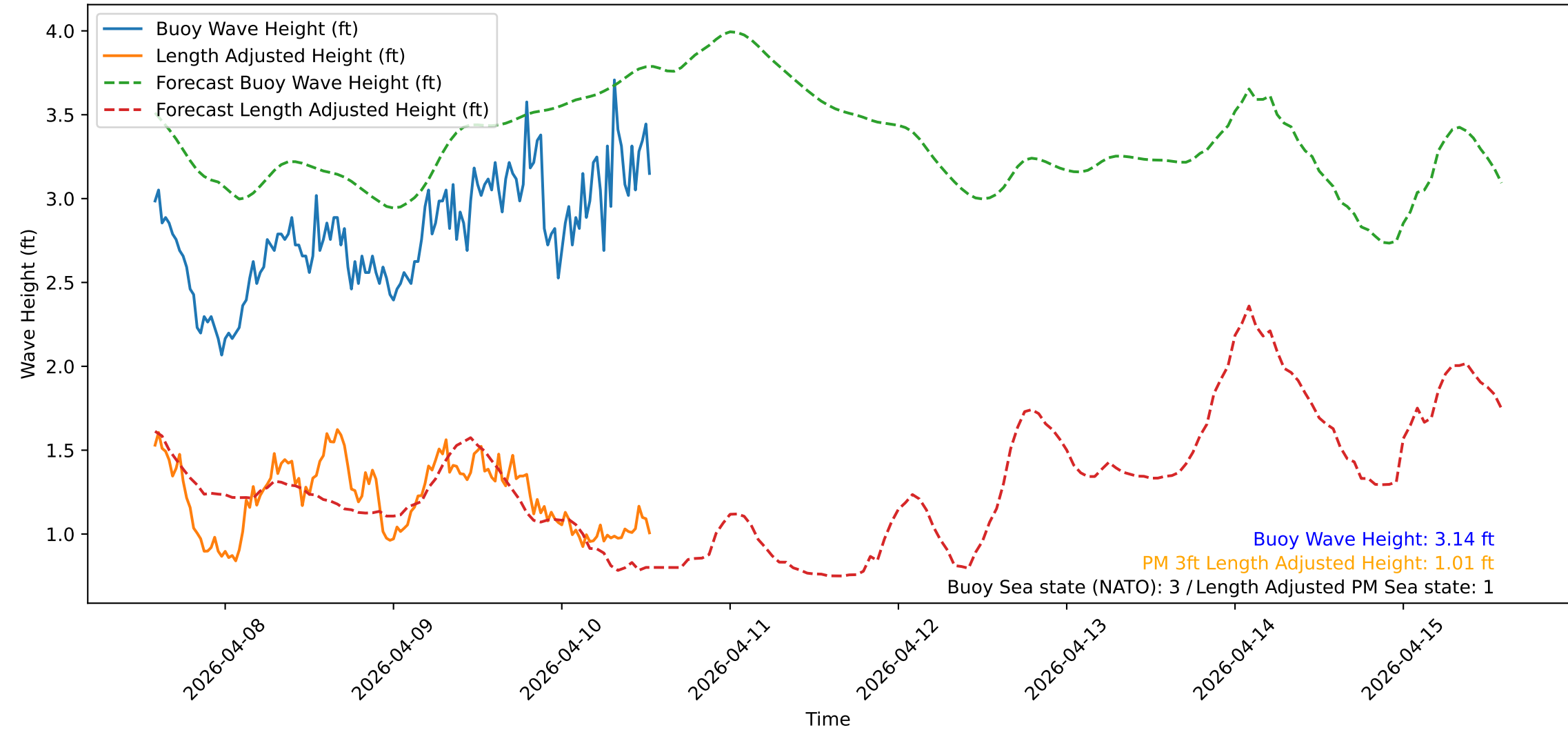
Wave Heights over Time for Red Beach at 2026-04-10 13:30:51
