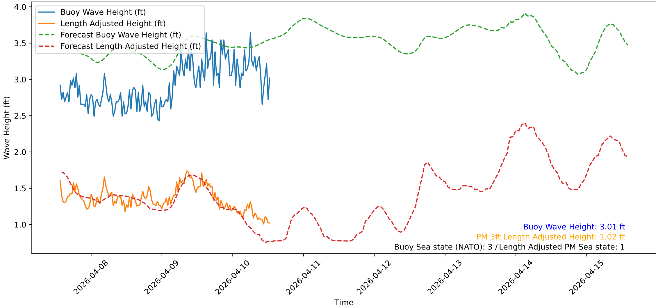
Wave Heights over Time for Oceanside Harbor at 2026-04-10 13:30:32
