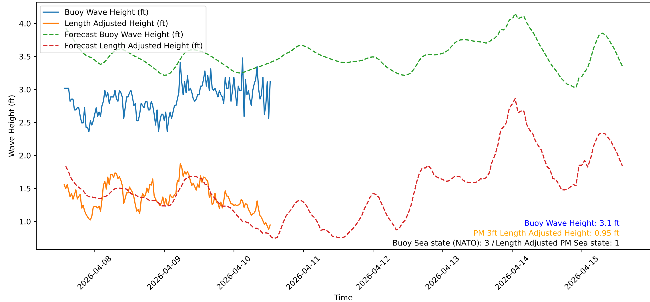
Wave Heights over Time for Green Beach at 2026-04-10 13:31:13
