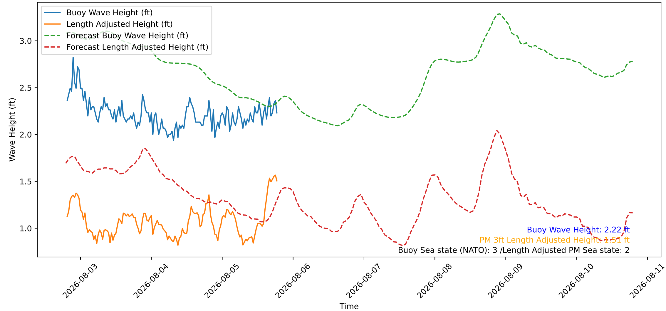
Wave Heights over Time for Green Beach at 2026-08-05 19:21:10
