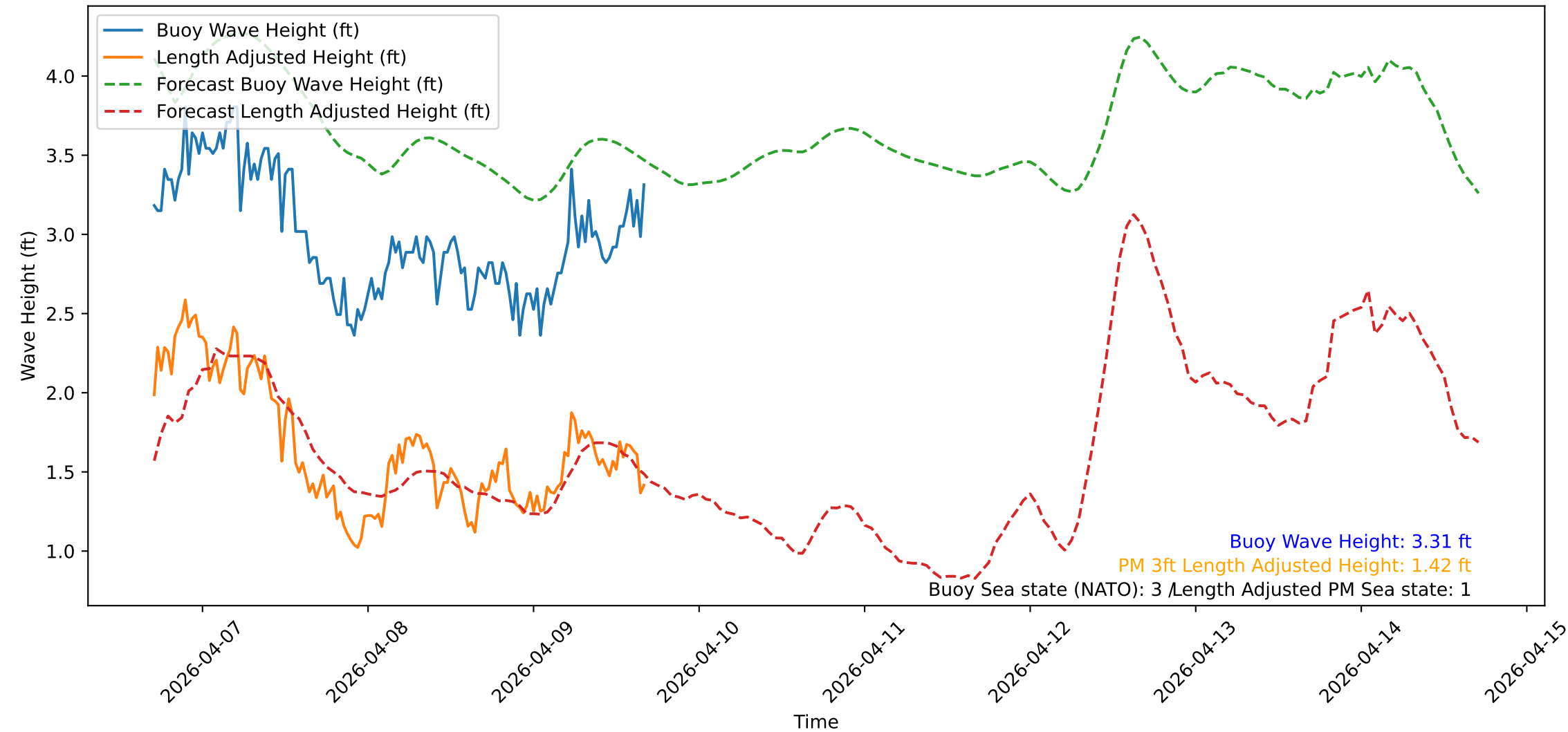
Wave Heights over Time for Green Beach at 2026-04-09 17:01:08
