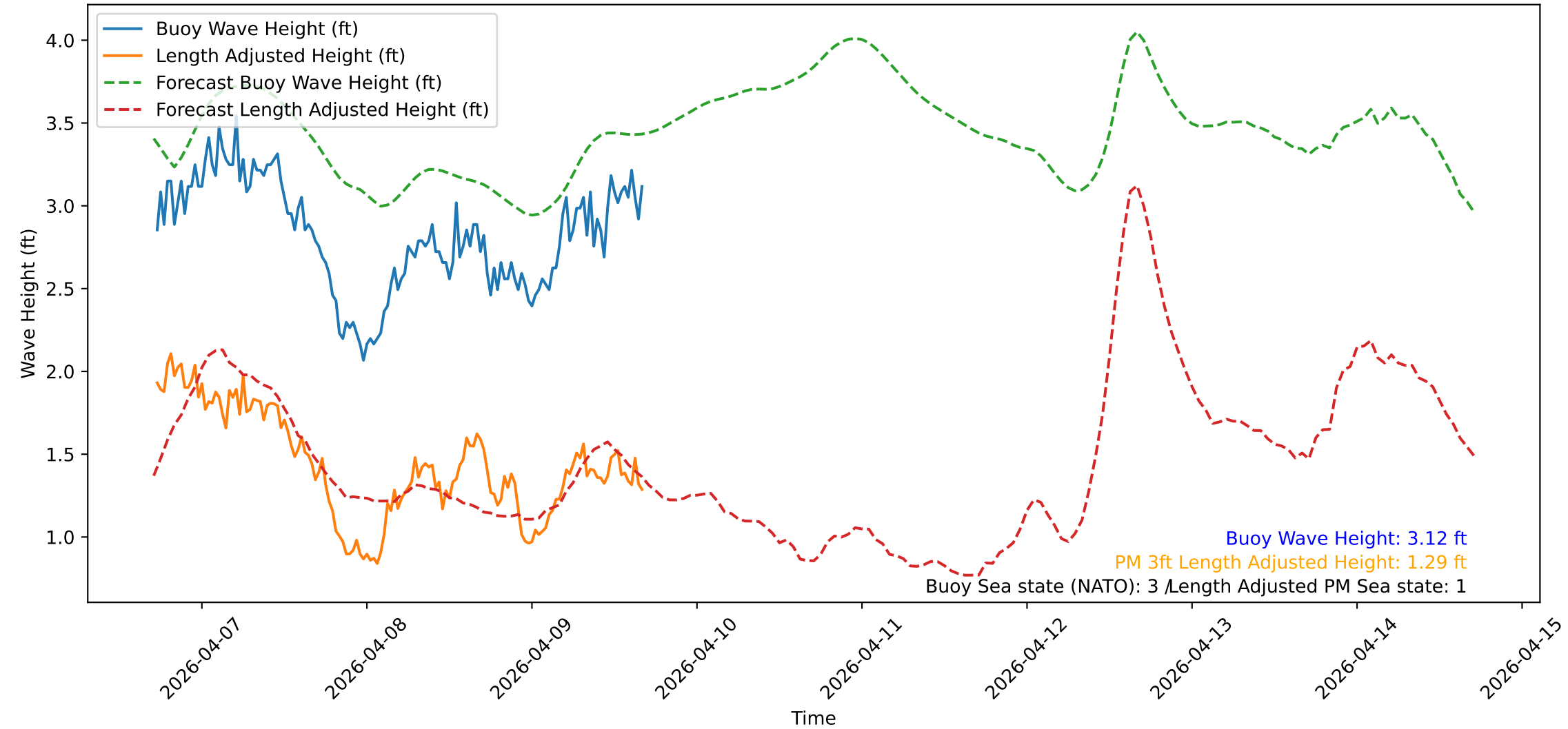
Wave Heights over Time for Red Beach at 2026-04-09 17:00:47
