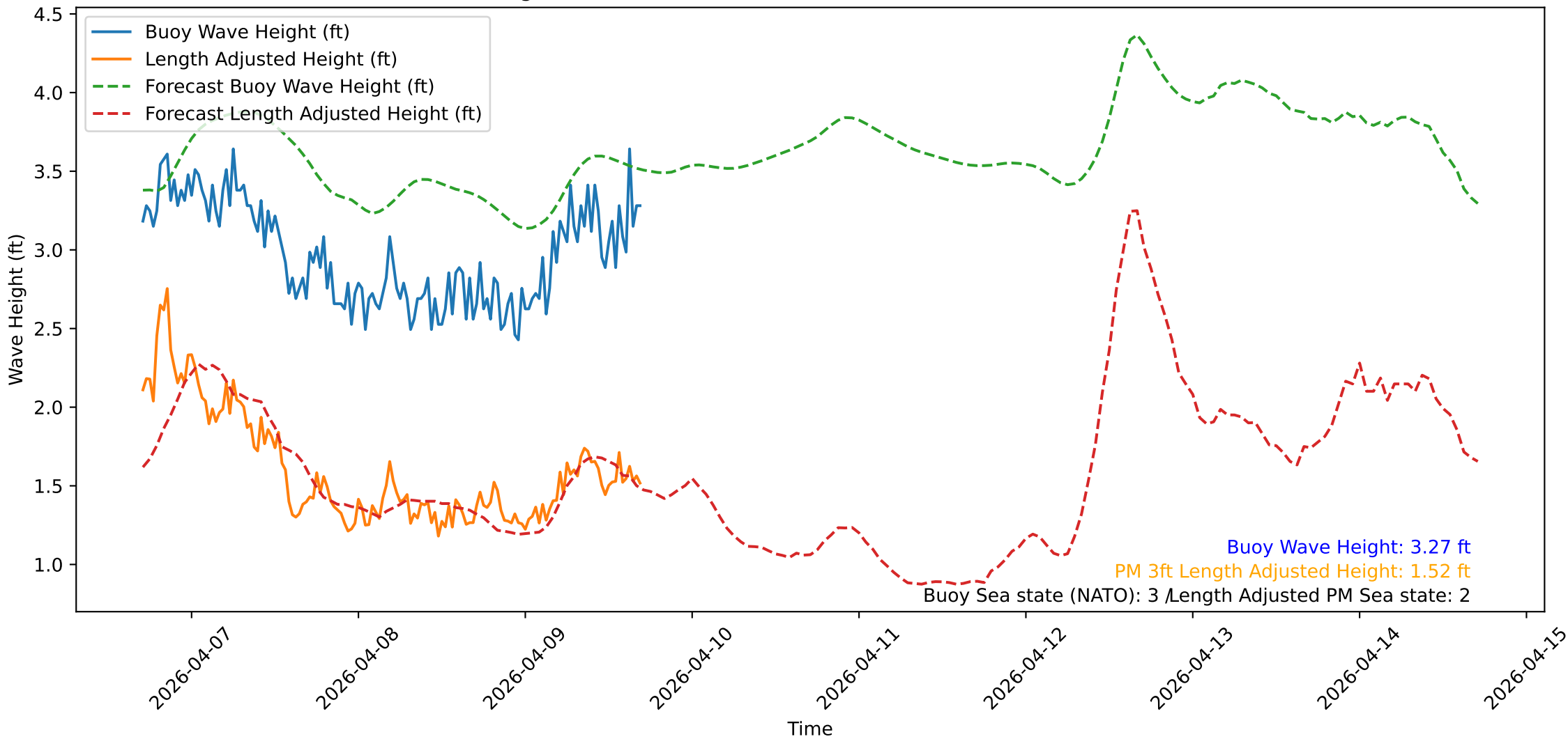
Wave Heights over Time for Oceanside Harbor at 2026-04-09 17:00:31
