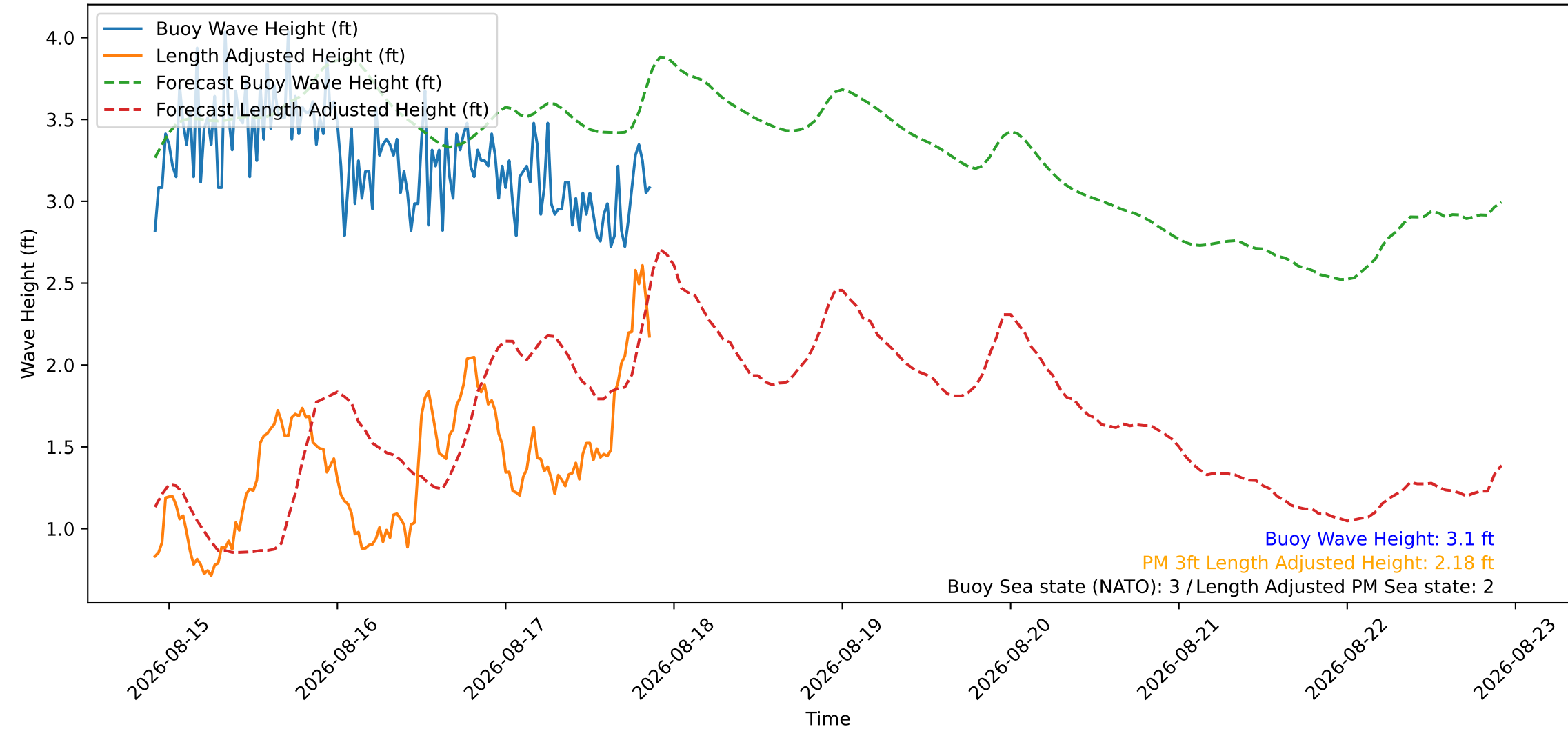
Wave Heights over Time for Red Beach at 2026-08-17 21:30:46
