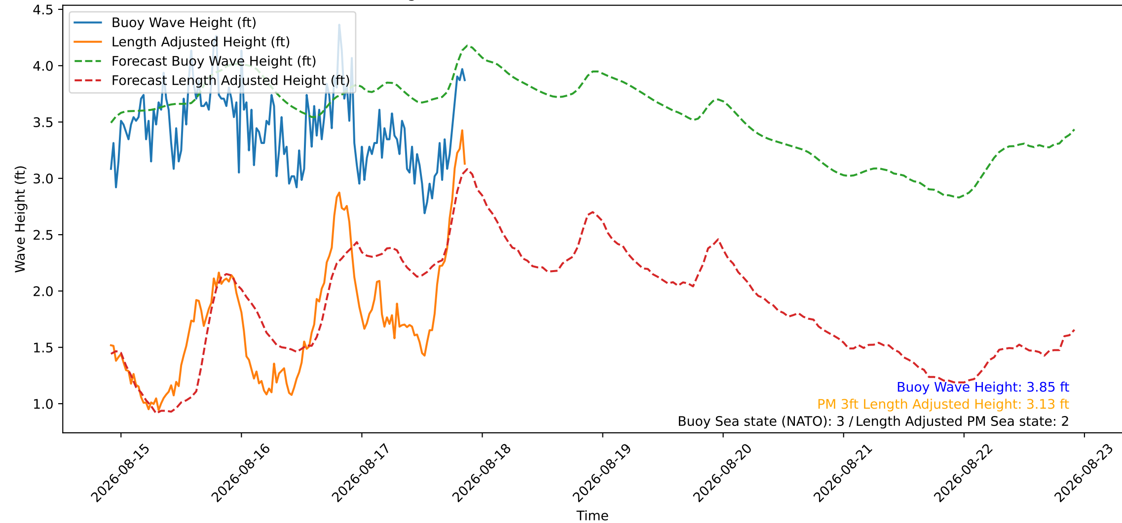
Wave Heights over Time for Green Beach at 2026-08-17 21:31:08
