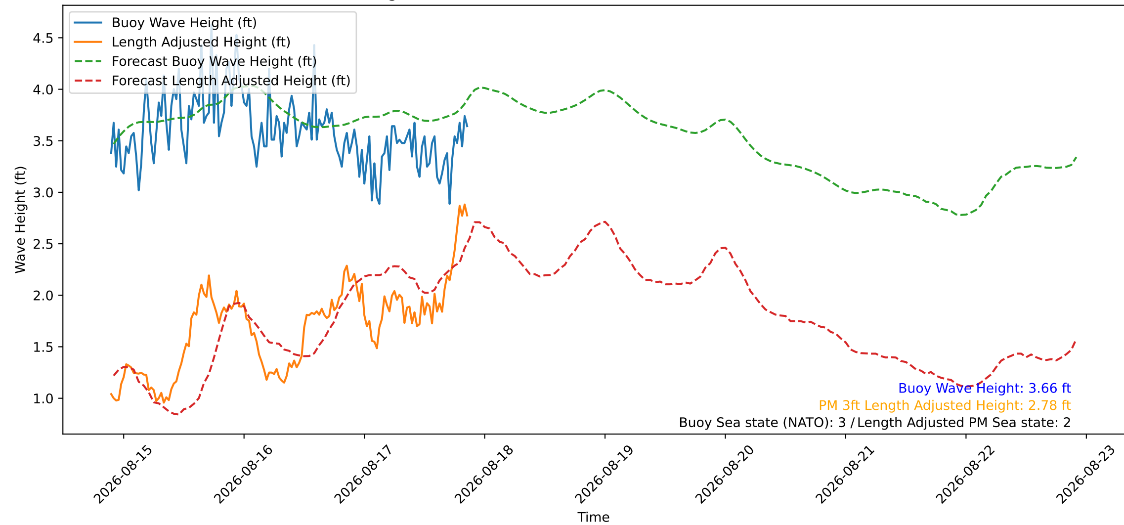
Wave Heights over Time for Oceanside Harbor at 2026-08-17 21:30:26
