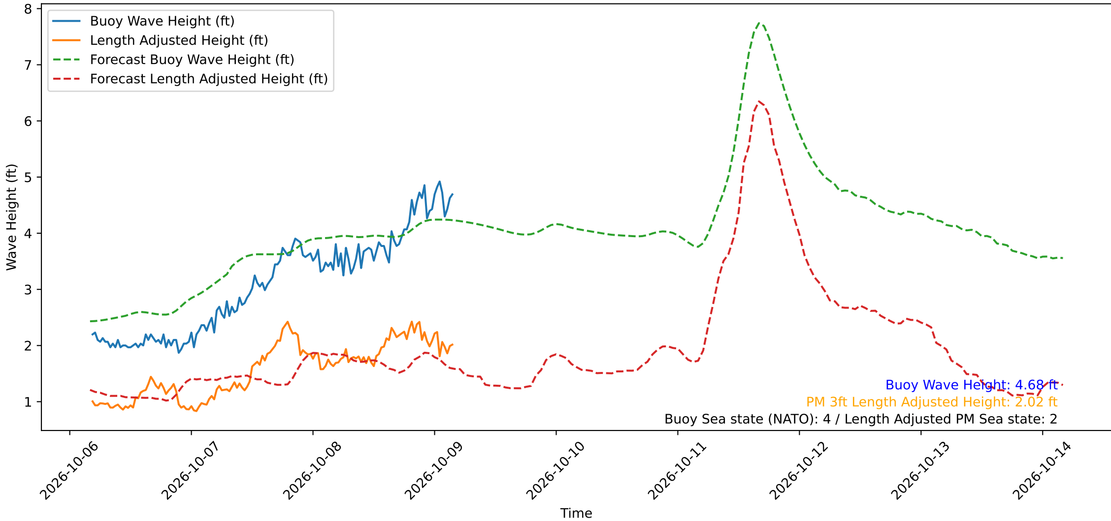
Wave Heights over Time for Red Beach at 2026-10-09 04:20:50
