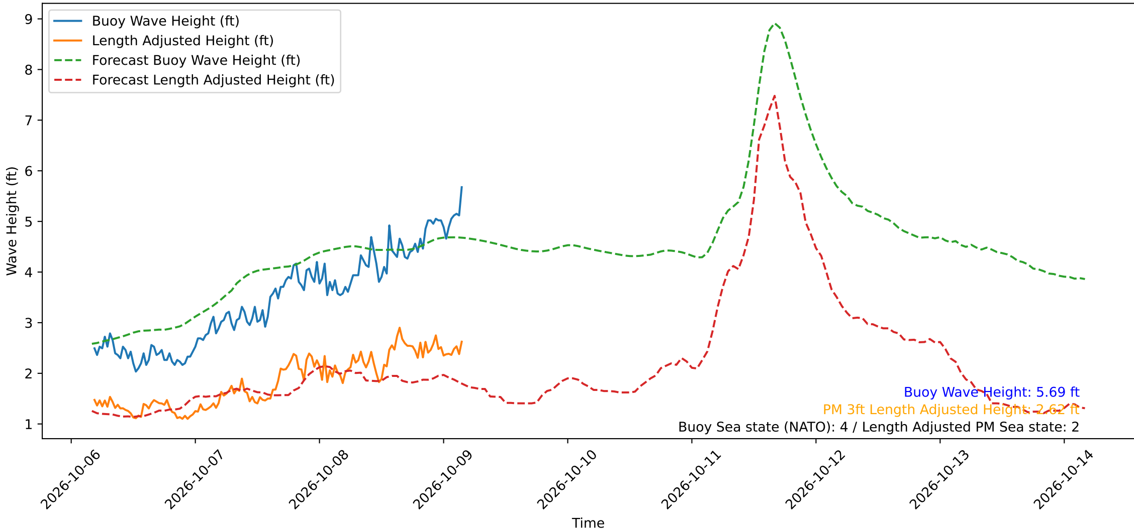
Wave Heights over Time for Oceanside Harbor at 2026-10-09 04:20:29
