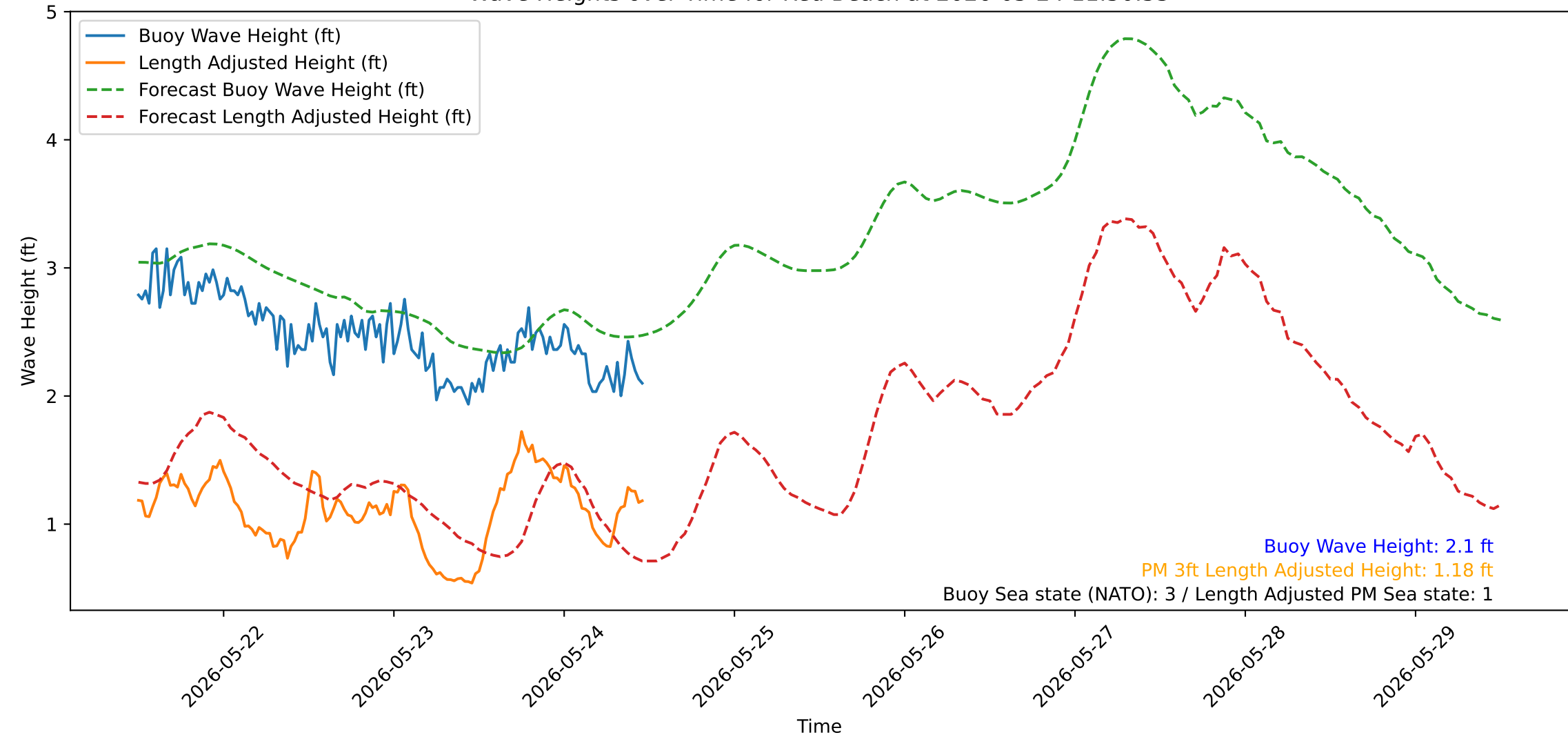
Wave Heights over Time for Red Beach at 2026-05-24 11:50:53
