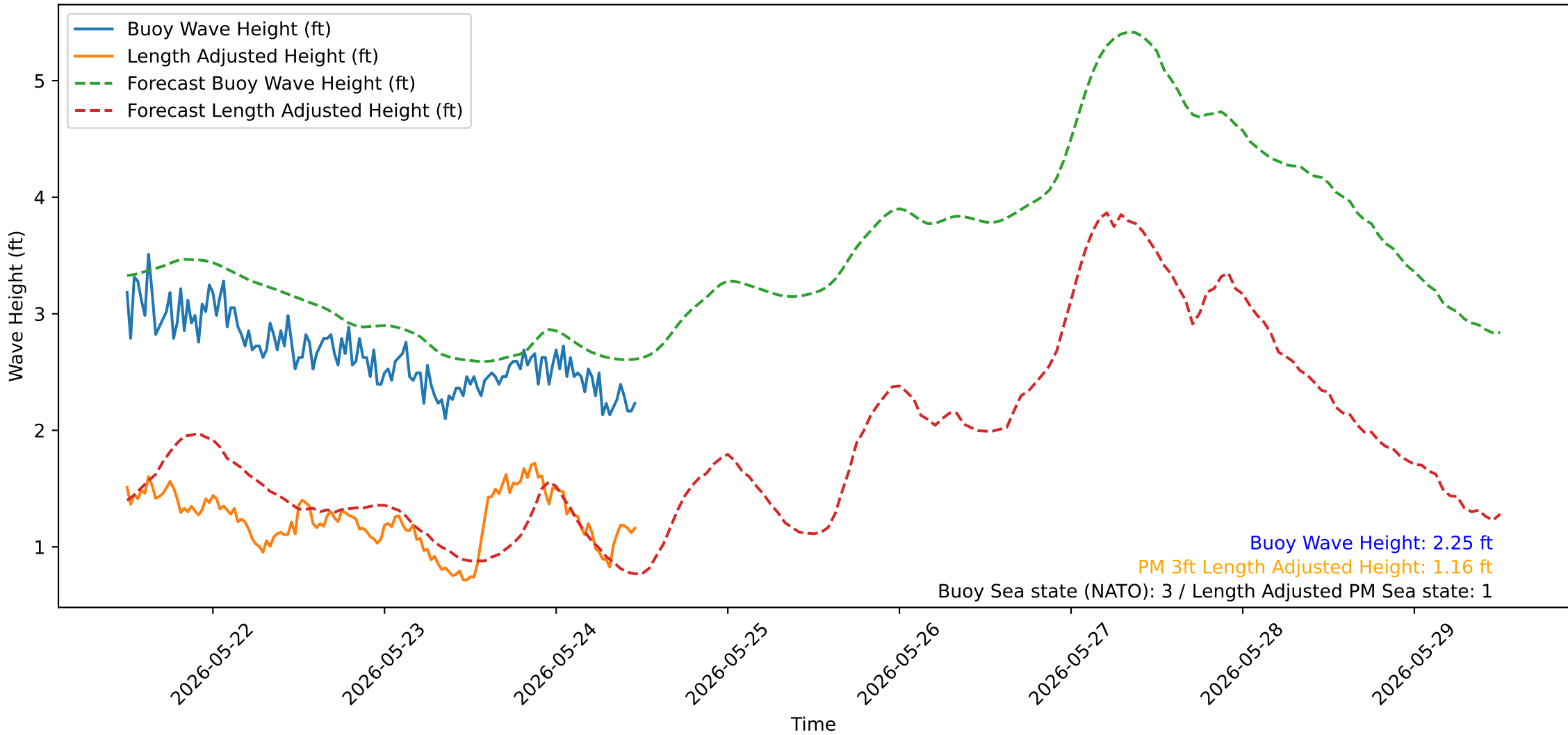
Wave Heights over Time for Oceanside Harbor at 2026-05-24 11:50:32
