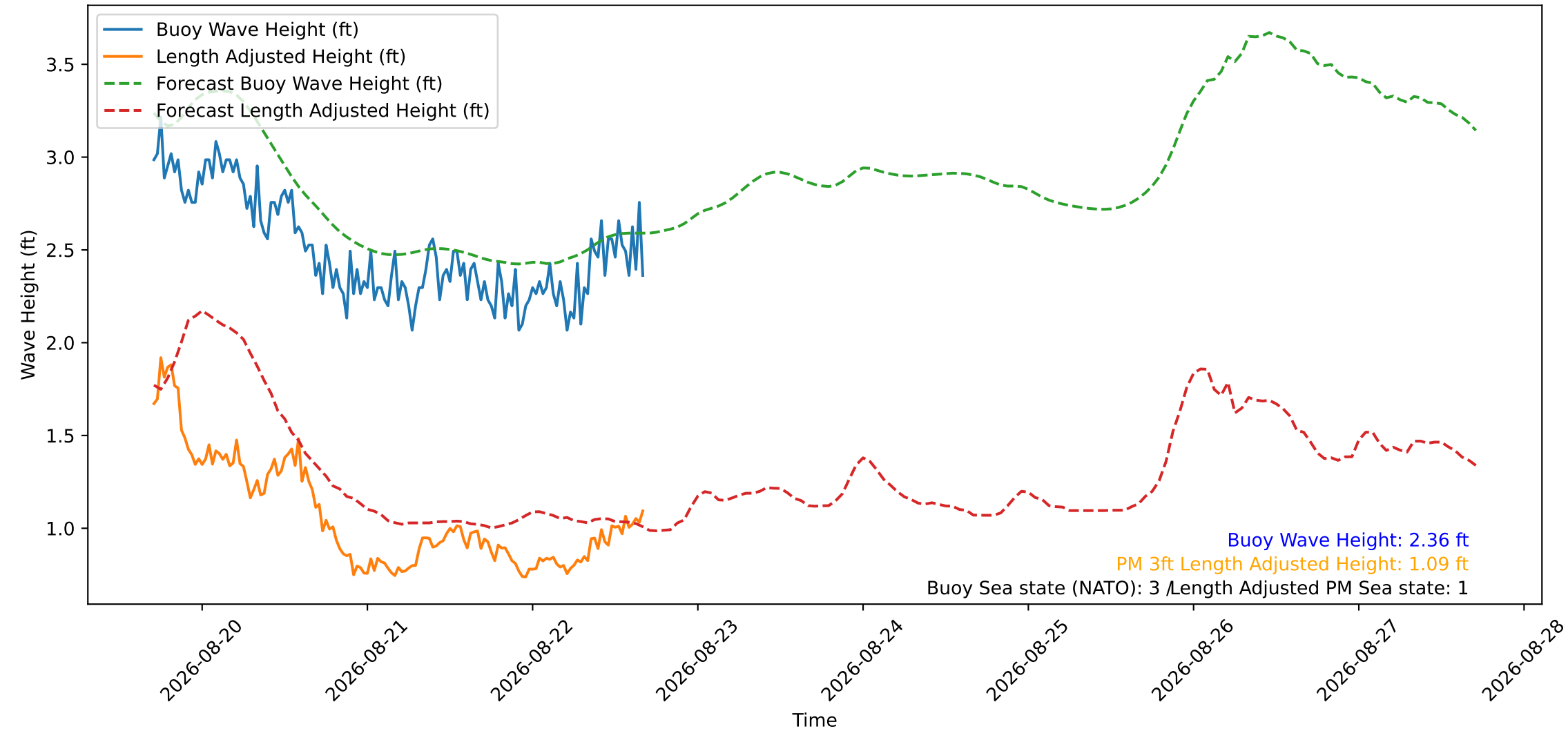
Wave Heights over Time for Red Beach at 2026-08-22 16:50:50
