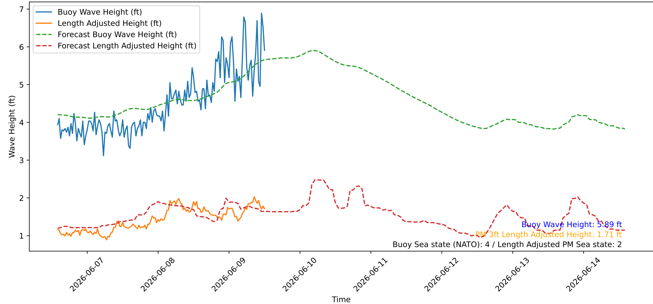
Wave Heights over Time for Green Beach at 2026-06-09 14:11:07
