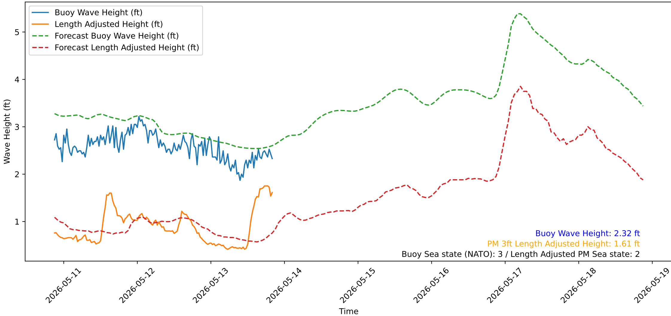
Wave Heights over Time for Red Beach at 2026-05-13 20:40:50
