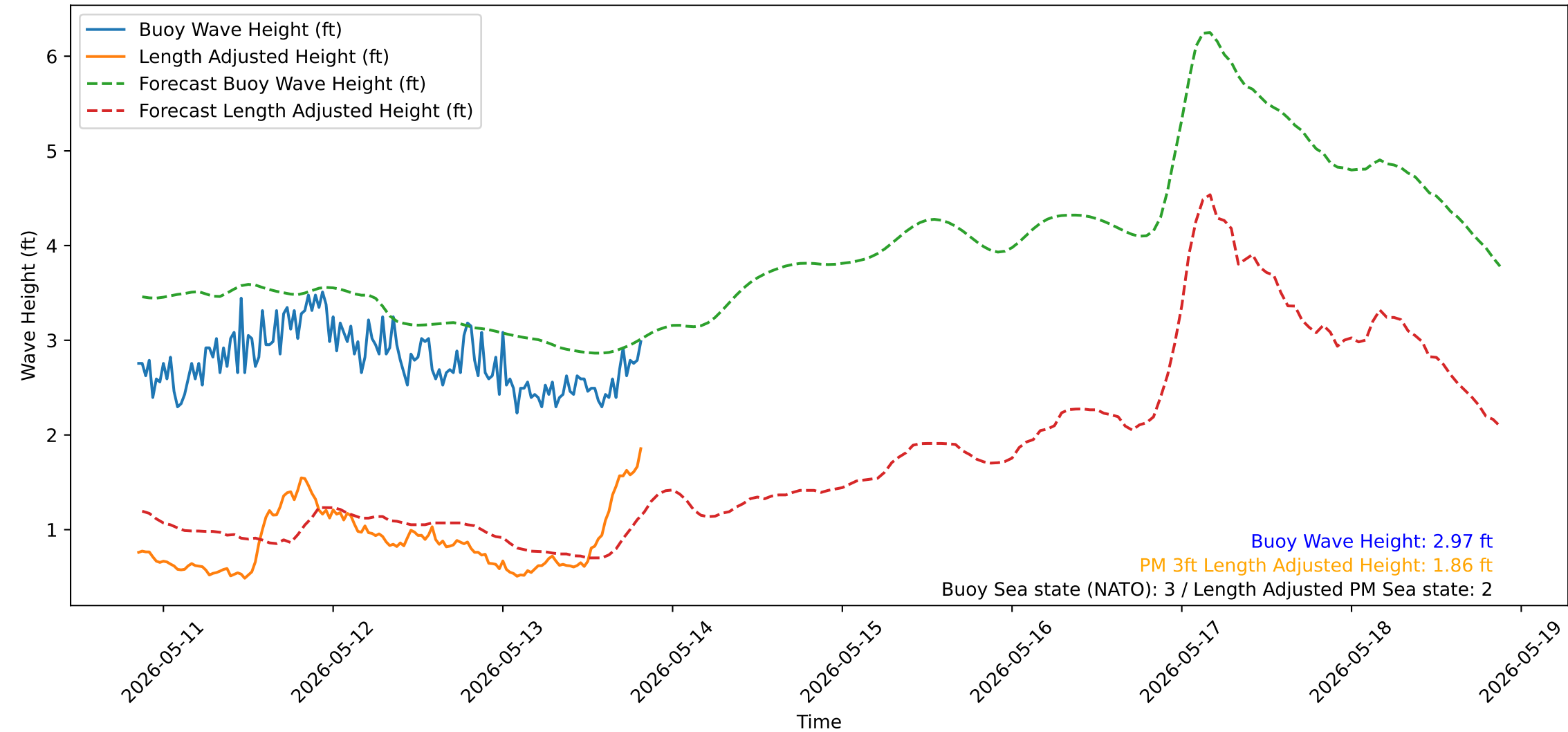
Wave Heights over Time for Green Beach at 2026-05-13 20:41:13
