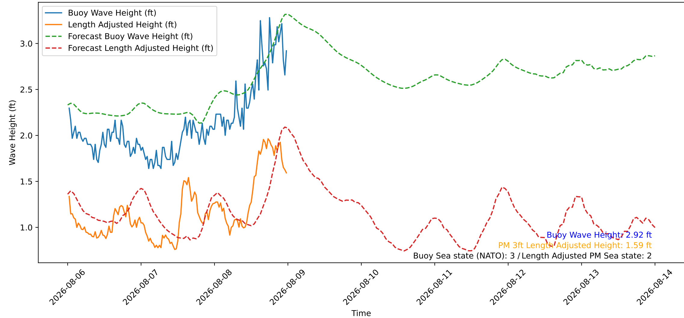
Wave Heights over Time for Oceanside Harbor at 2026-08-09 00:20:26
