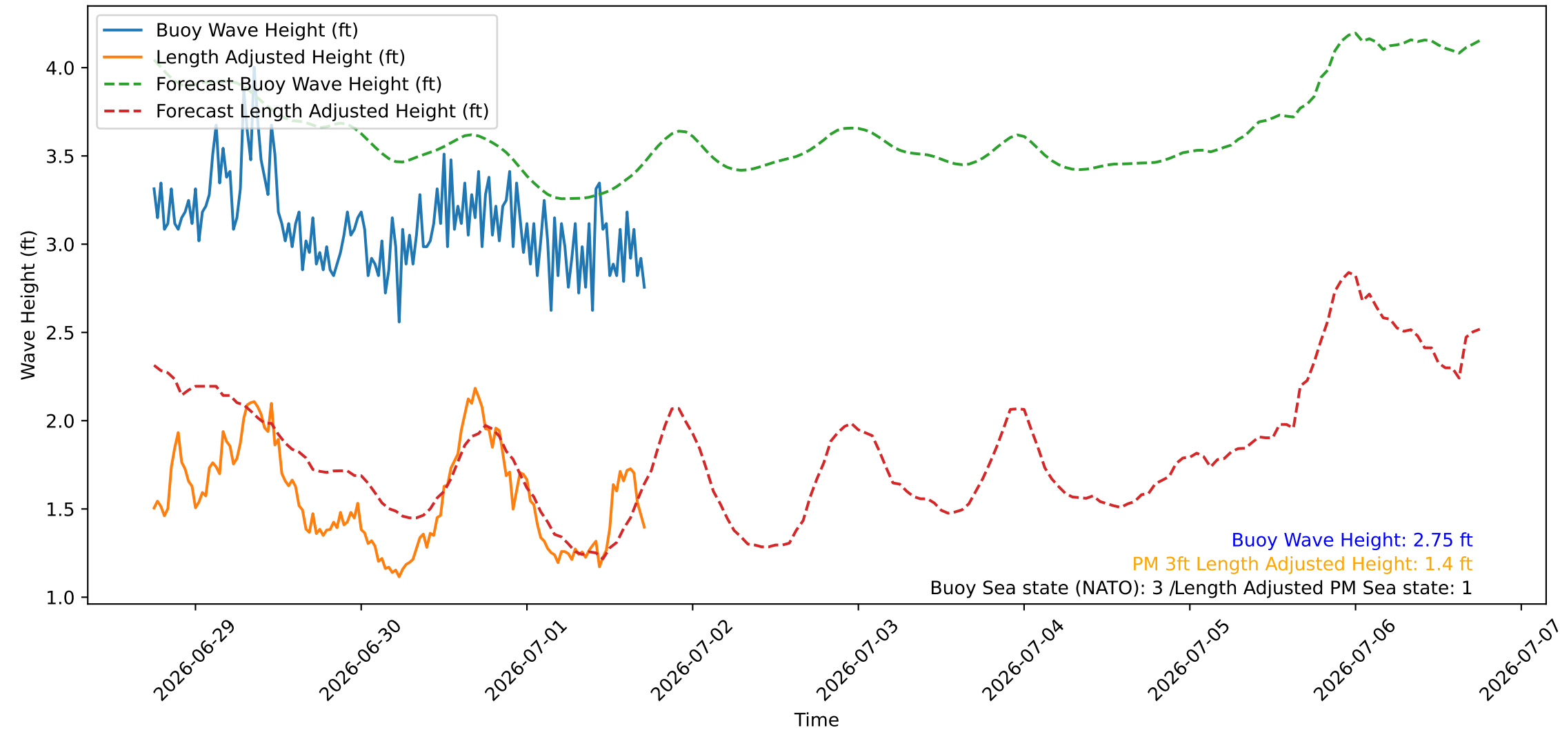
Wave Heights over Time for Oceanside Harbor at 2026-07-01 17:50:26
