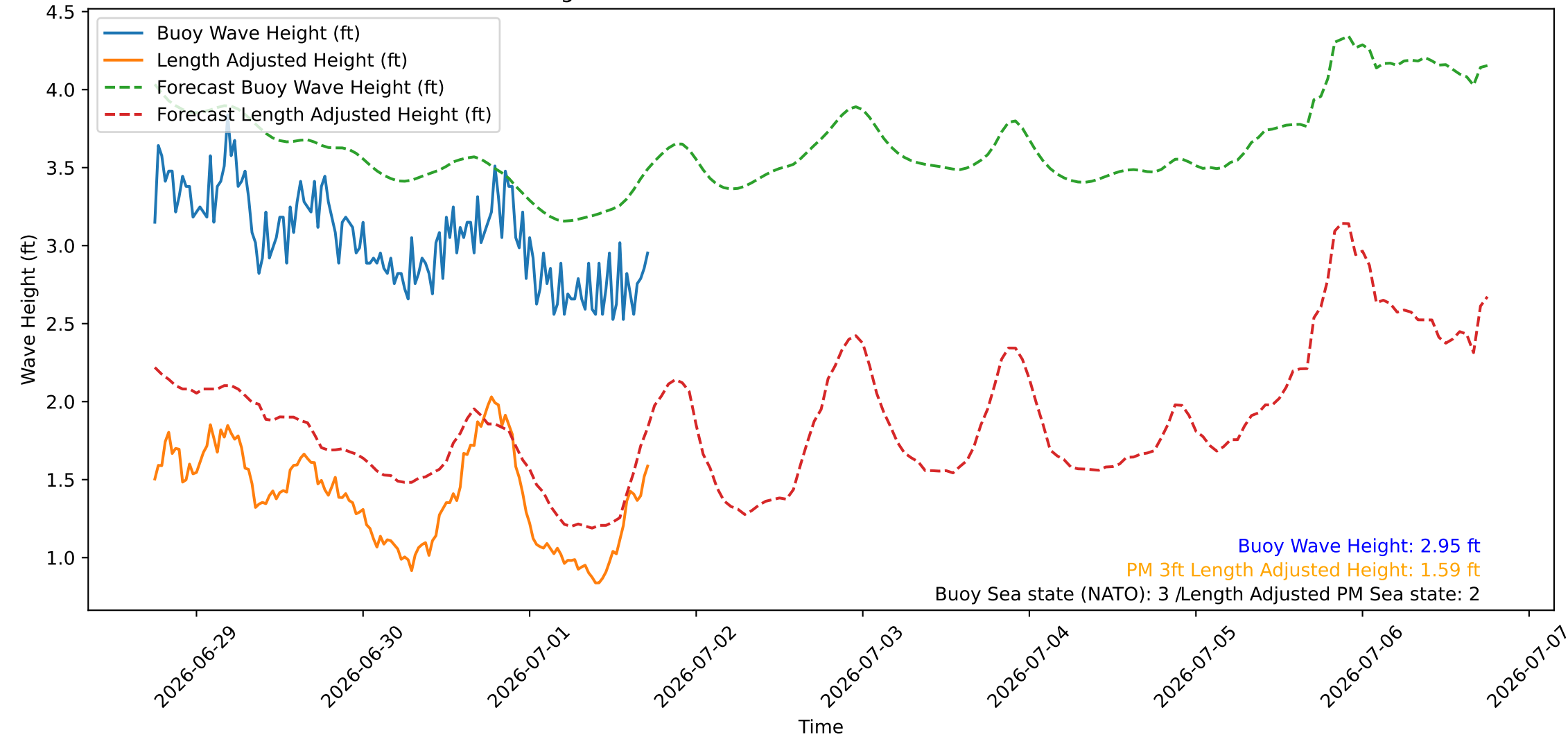
Wave Heights over Time for Green Beach at 2026-07-01 17:51:08
