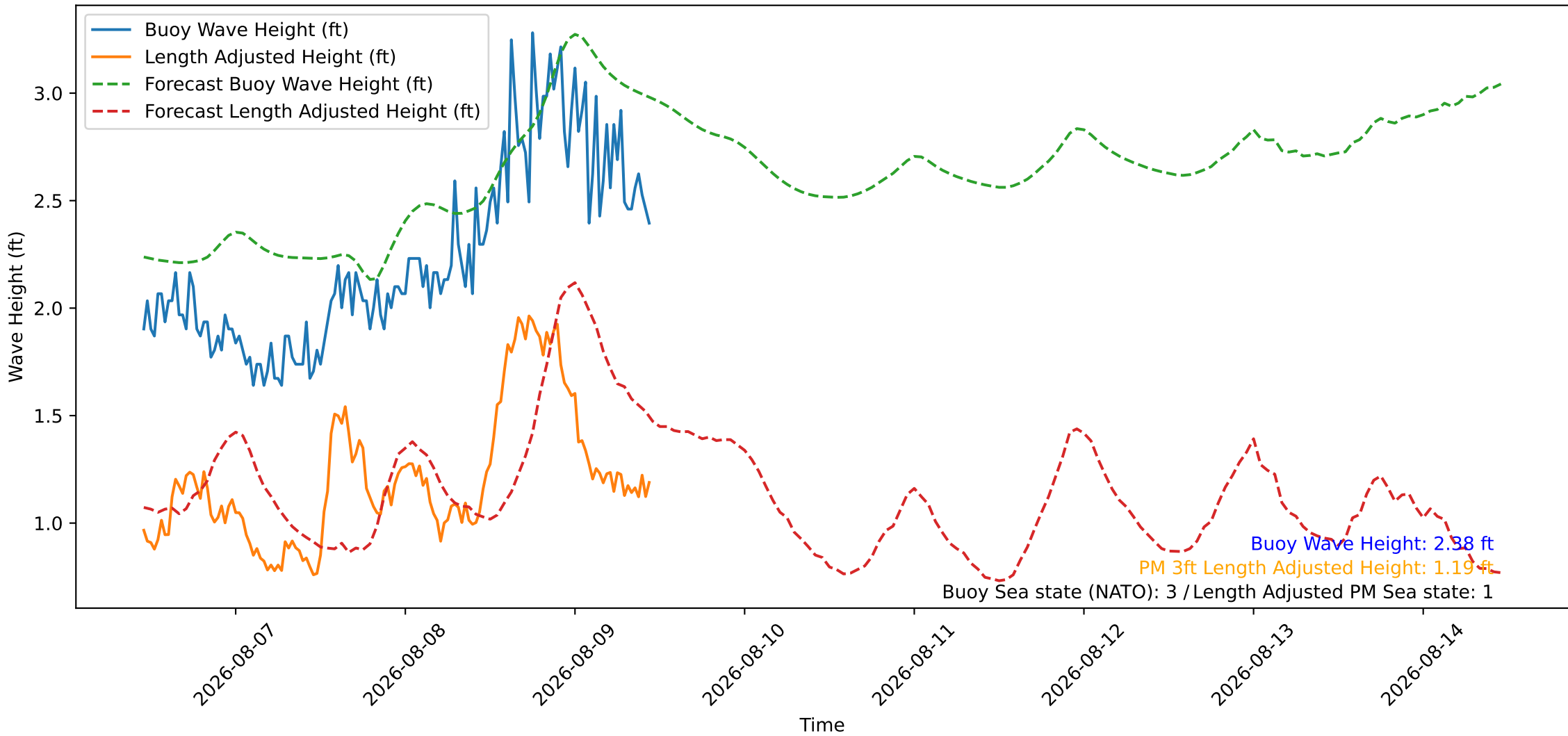
Wave Heights over Time for Oceanside Harbor at 2026-08-09 11:00:27
