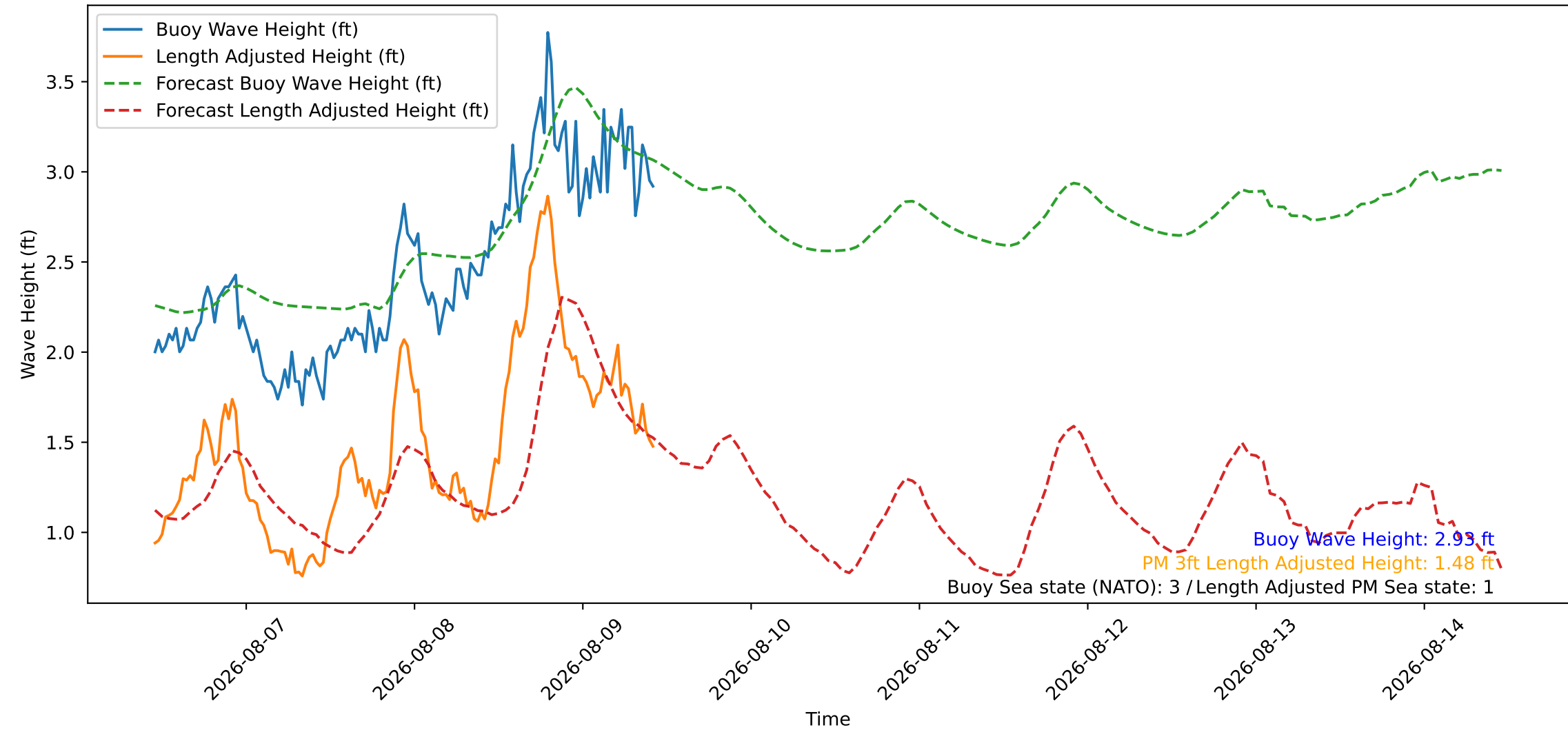
Wave Heights over Time for Green Beach at 2026-08-09 11:01:09
