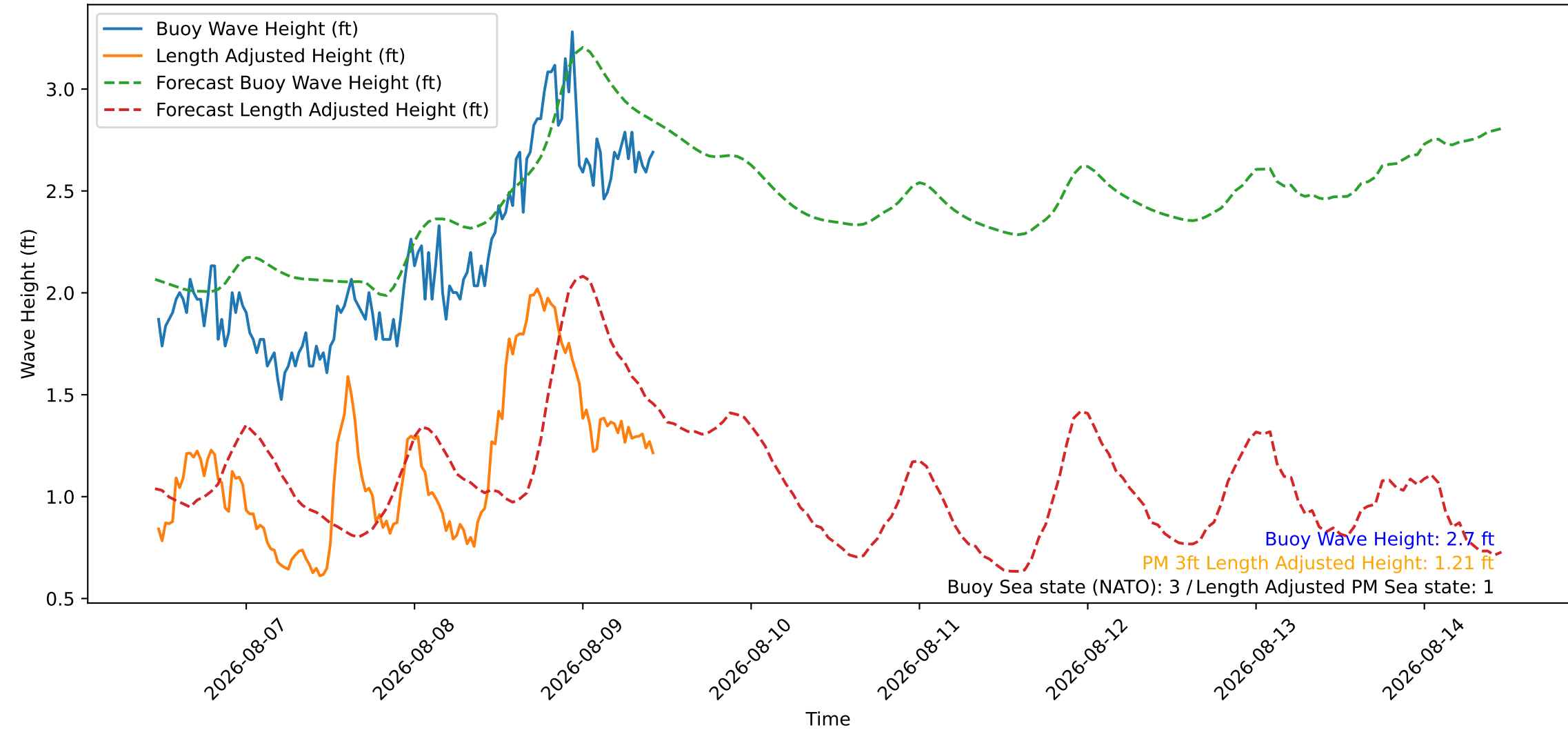
Wave Heights over Time for Red Beach at 2026-08-09 11:00:46
