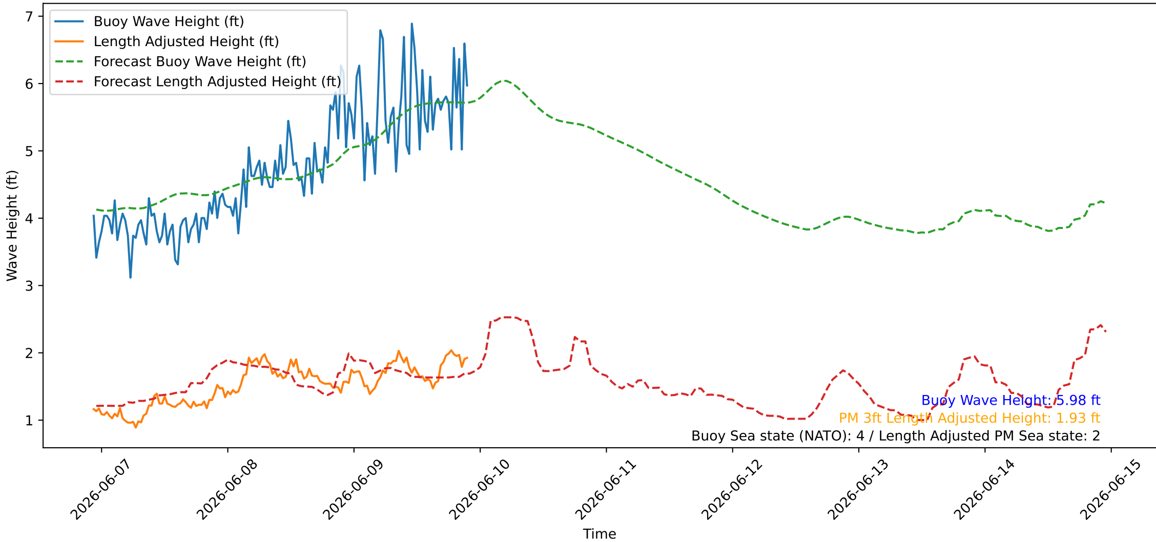
Wave Heights over Time for Green Beach at 2026-06-09 22:31:10
