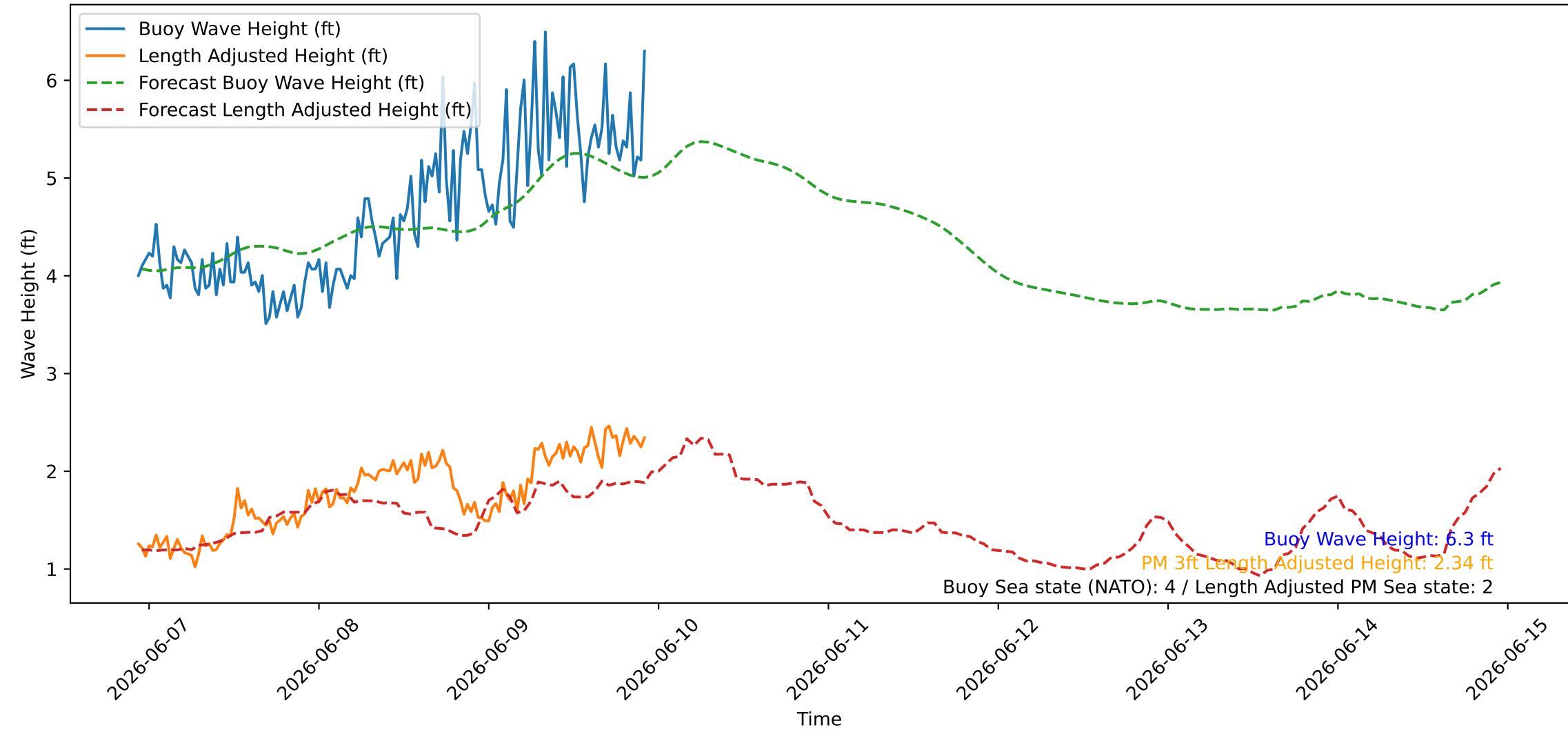
Wave Heights over Time for Oceanside Harbor at 2026-06-09 22:30:27
