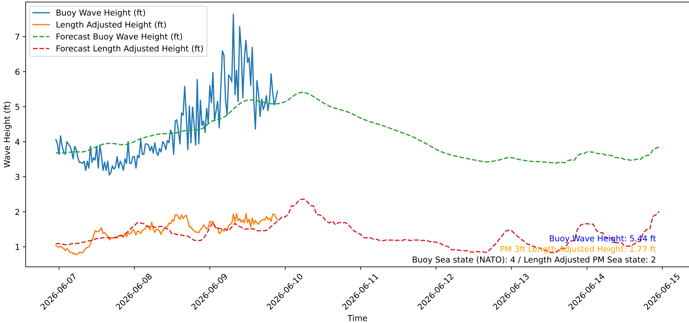
Wave Heights over Time for Red Beach at 2026-06-09 22:30:47
