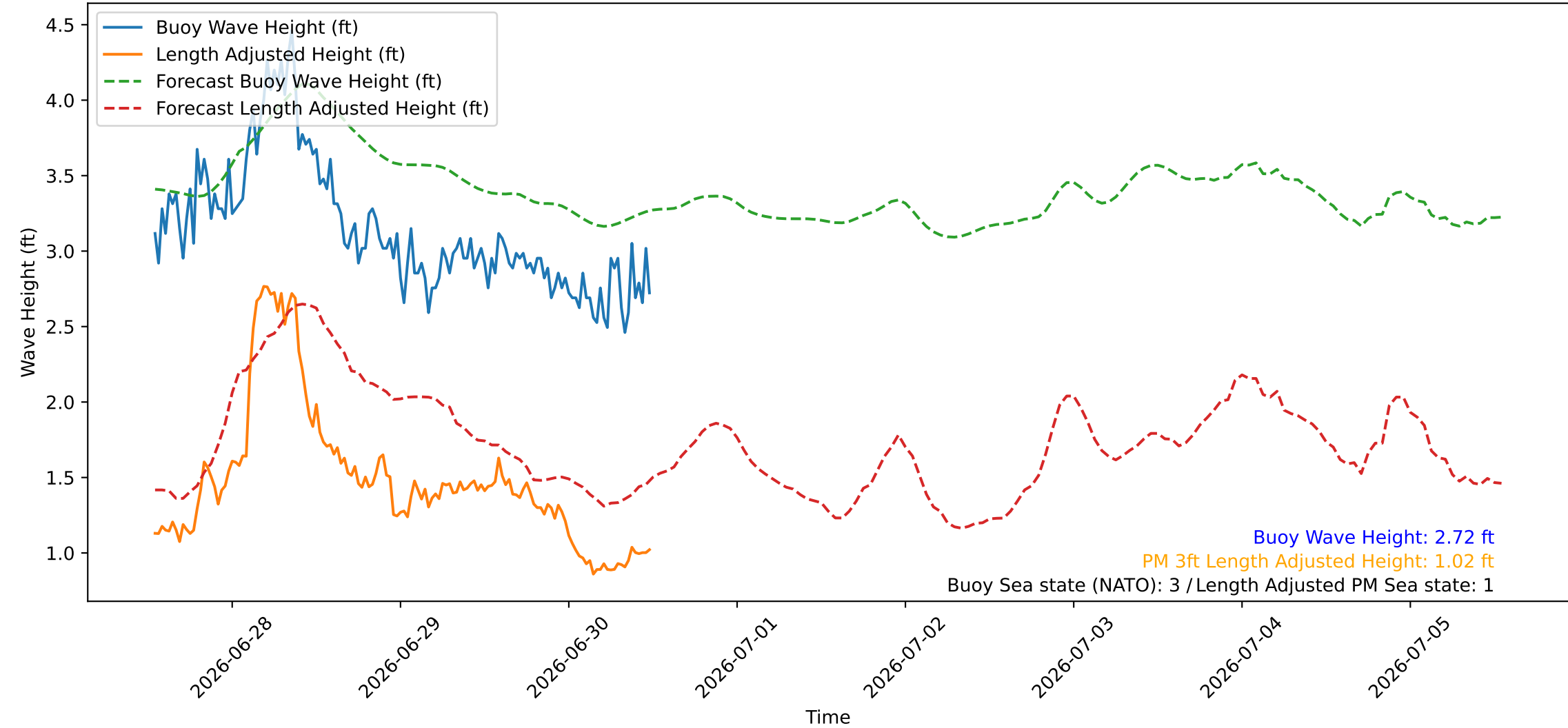
Wave Heights over Time for Red Beach at 2026-06-30 12:40:46
