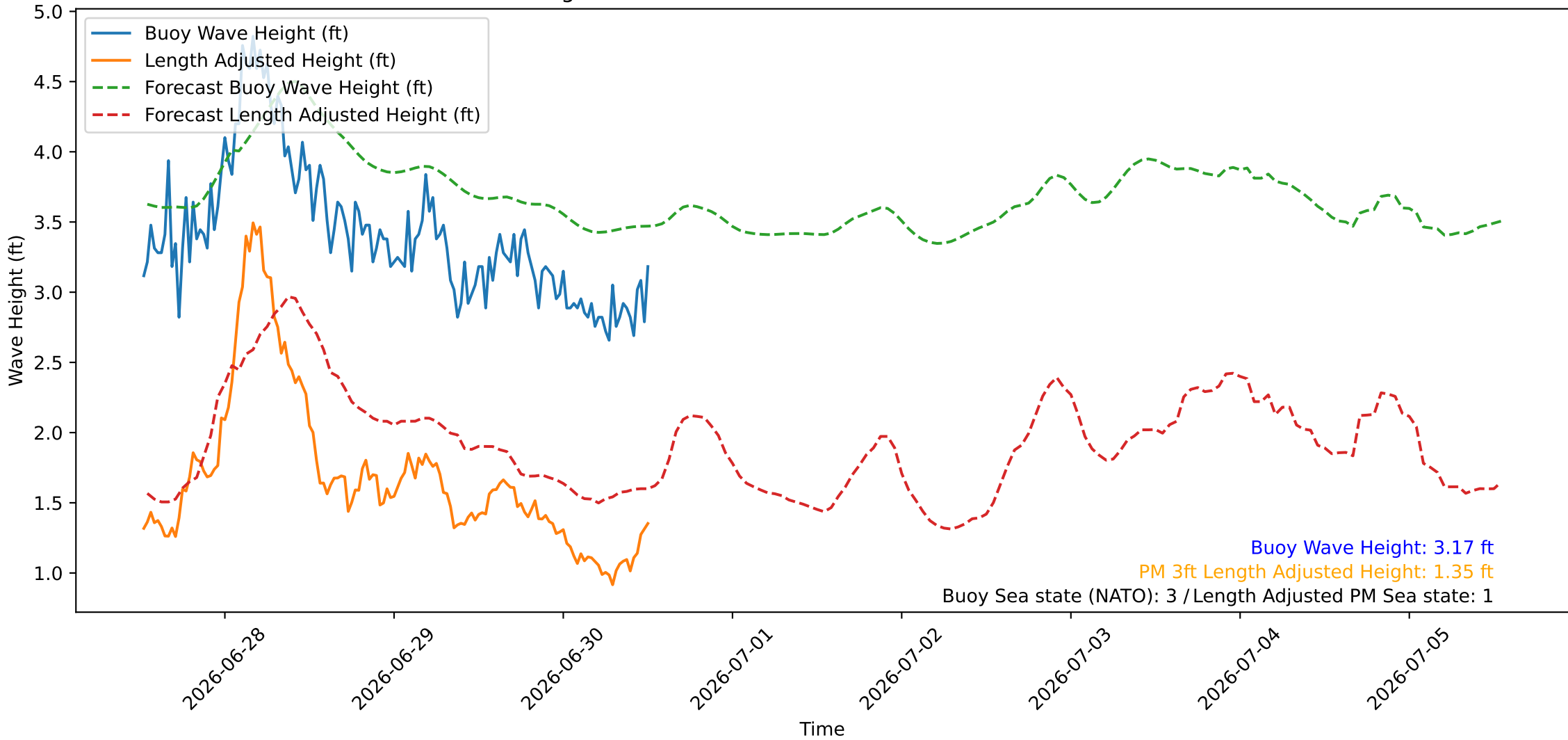
Wave Heights over Time for Green Beach at 2026-06-30 12:41:08
