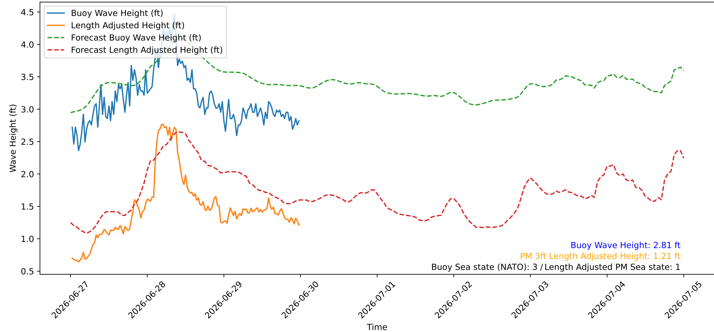
Wave Heights over Time for Red Beach at 2026-06-30 00:10:45
