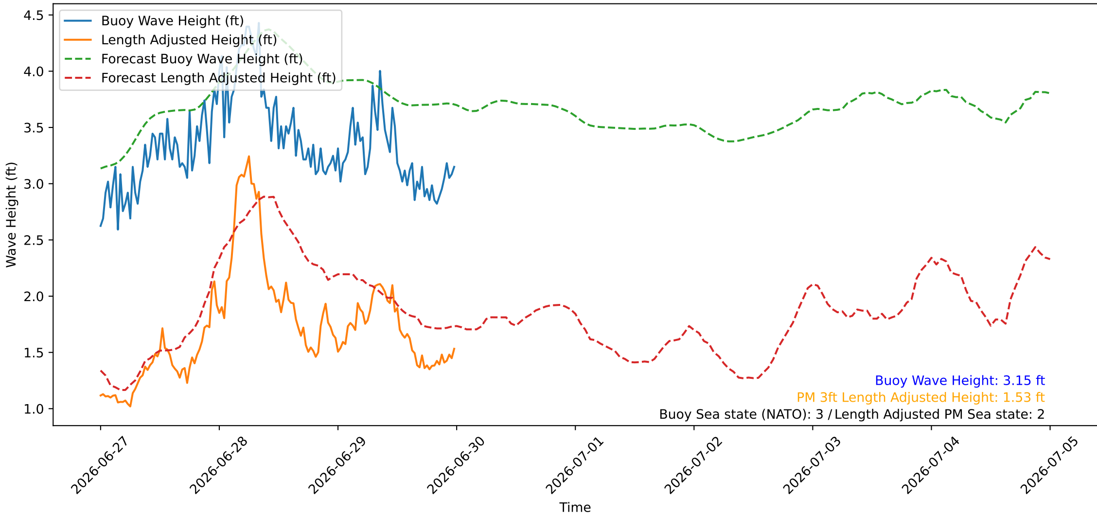
Wave Heights over Time for Oceanside Harbor at 2026-06-30 00:10:26
