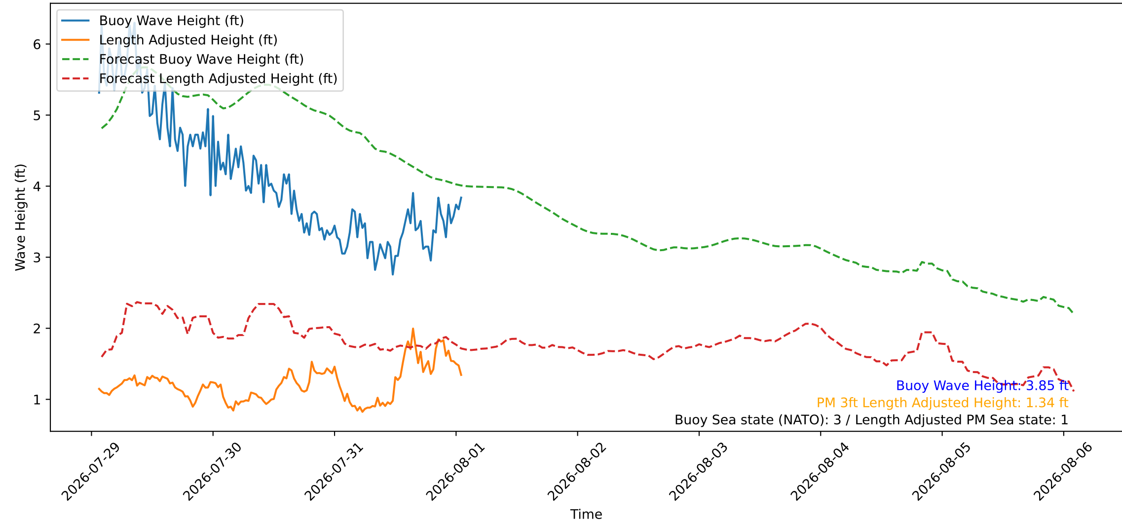
Wave Heights over Time for Green Beach at 2026-08-01 01:41:09
