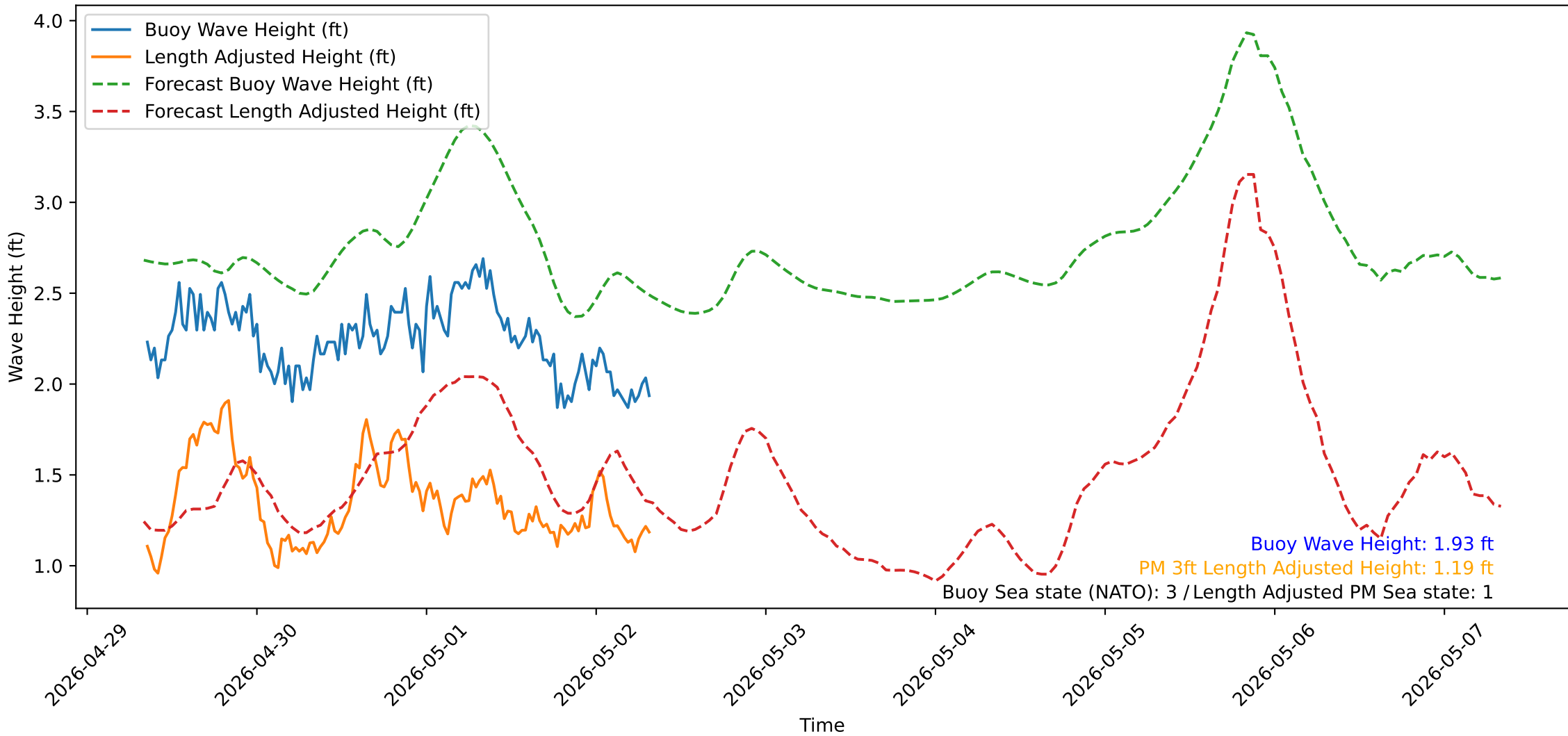
Wave Heights over Time for Oceanside Harbor at 2026-05-02 08:20:31
