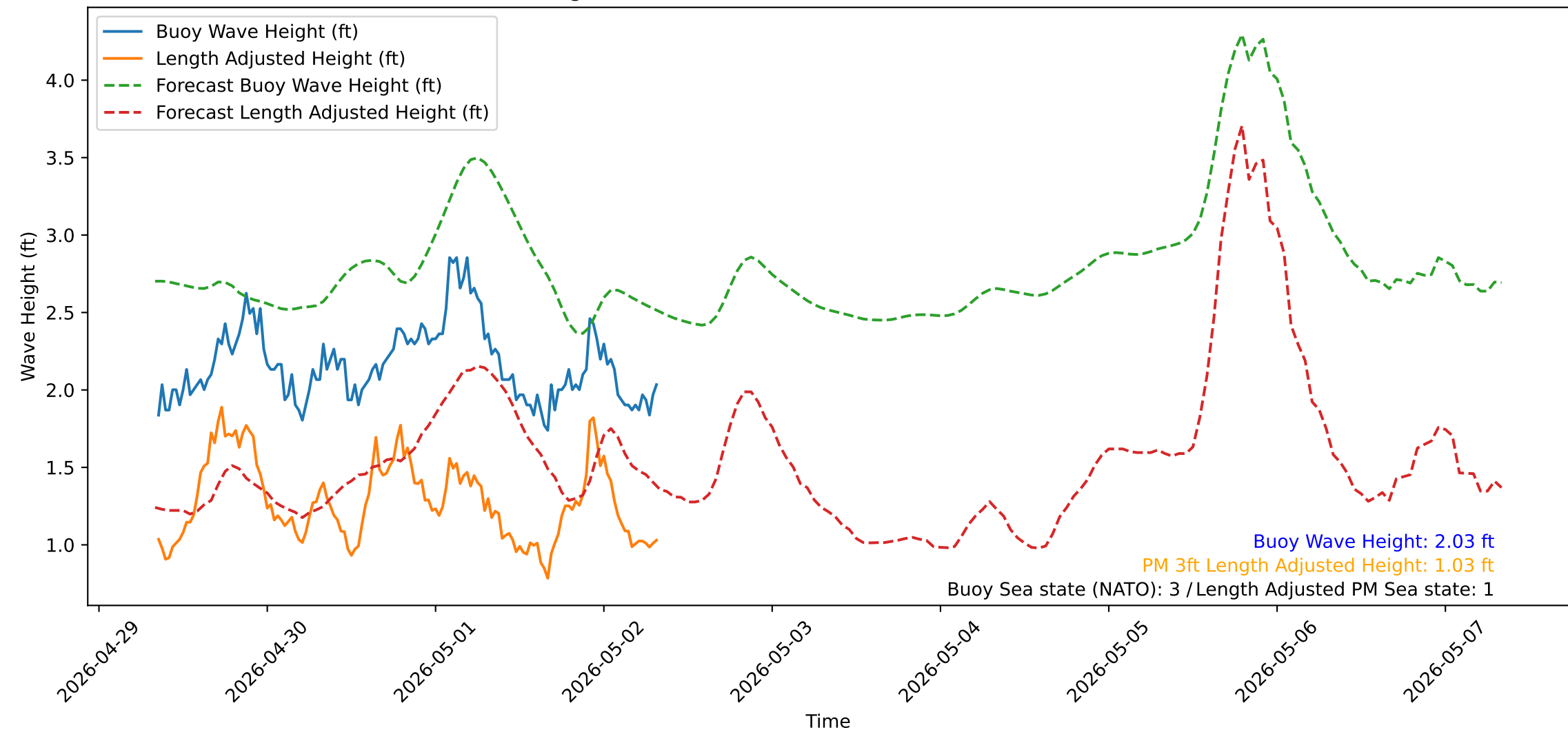
Wave Heights over Time for Green Beach at 2026-05-02 08:21:14
