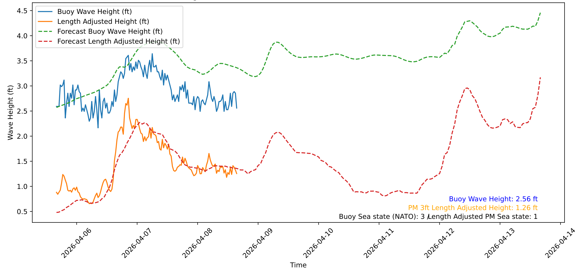
Wave Heights over Time for Oceanside Harbor at 2026-04-08 16:00:32
