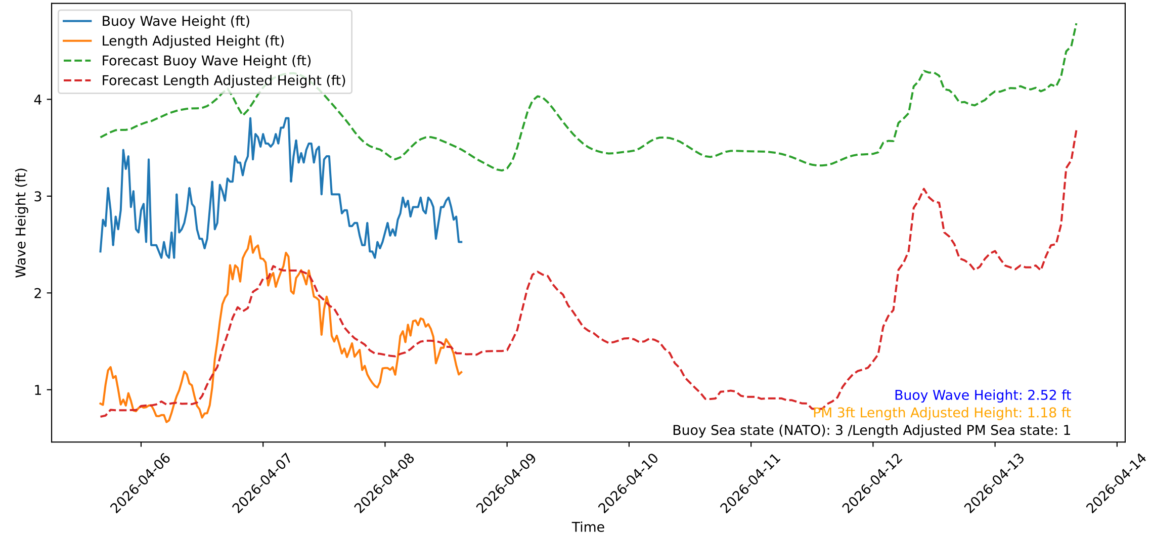
Wave Heights over Time for Green Beach at 2026-04-08 16:01:10
