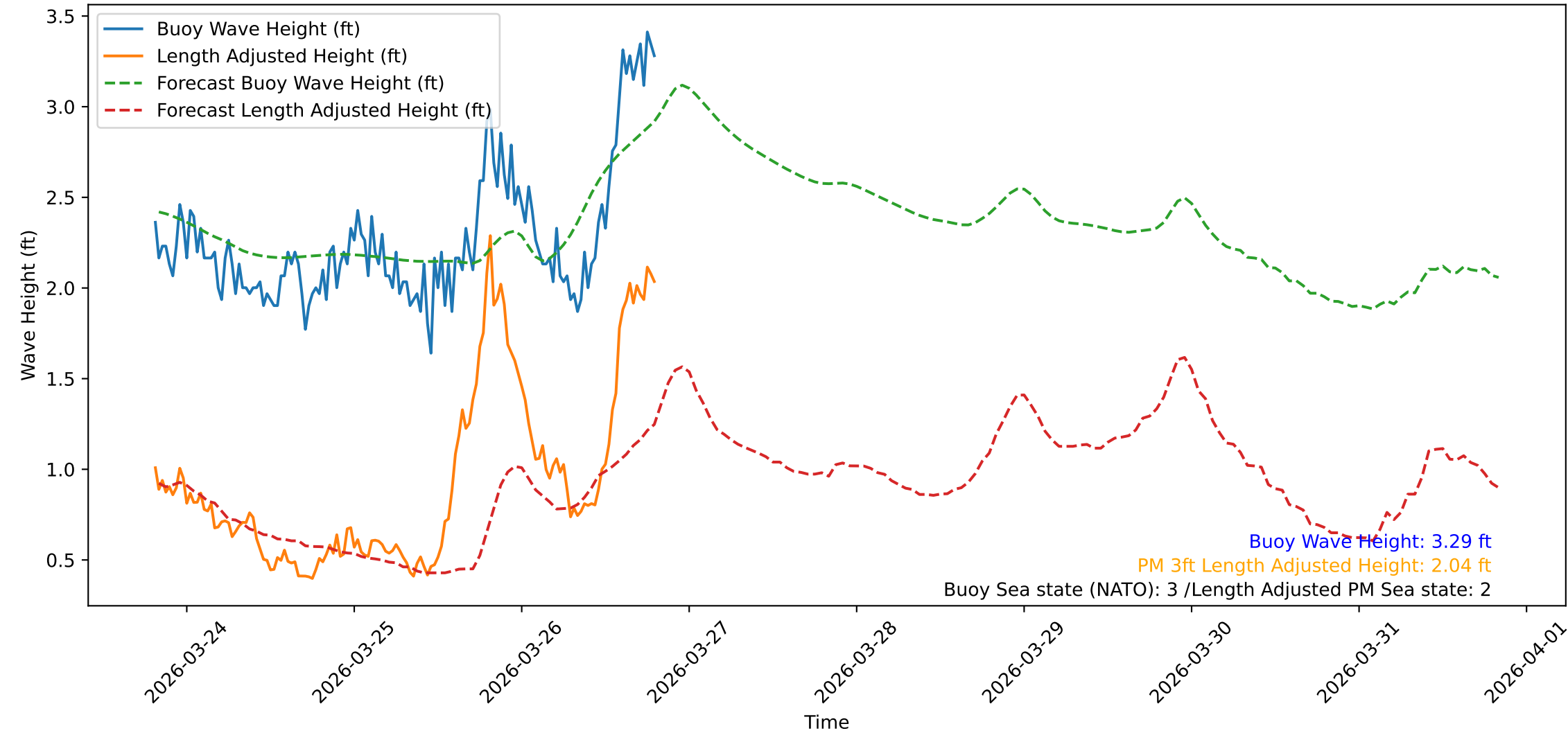
Wave Heights over Time for Green Beach at 2026-03-26 19:41:10
