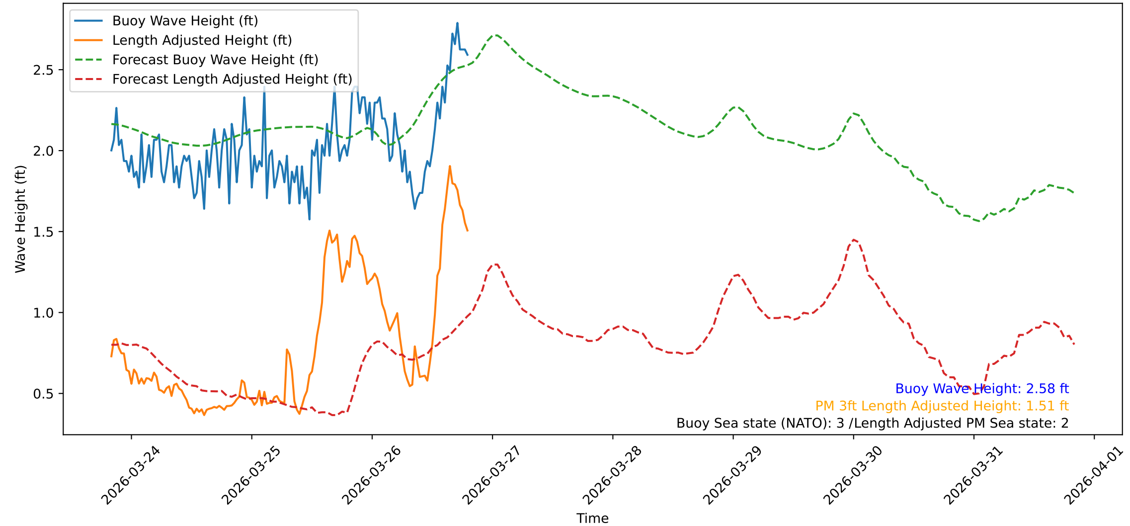
Wave Heights over Time for Red Beach at 2026-03-26 19:40:47
