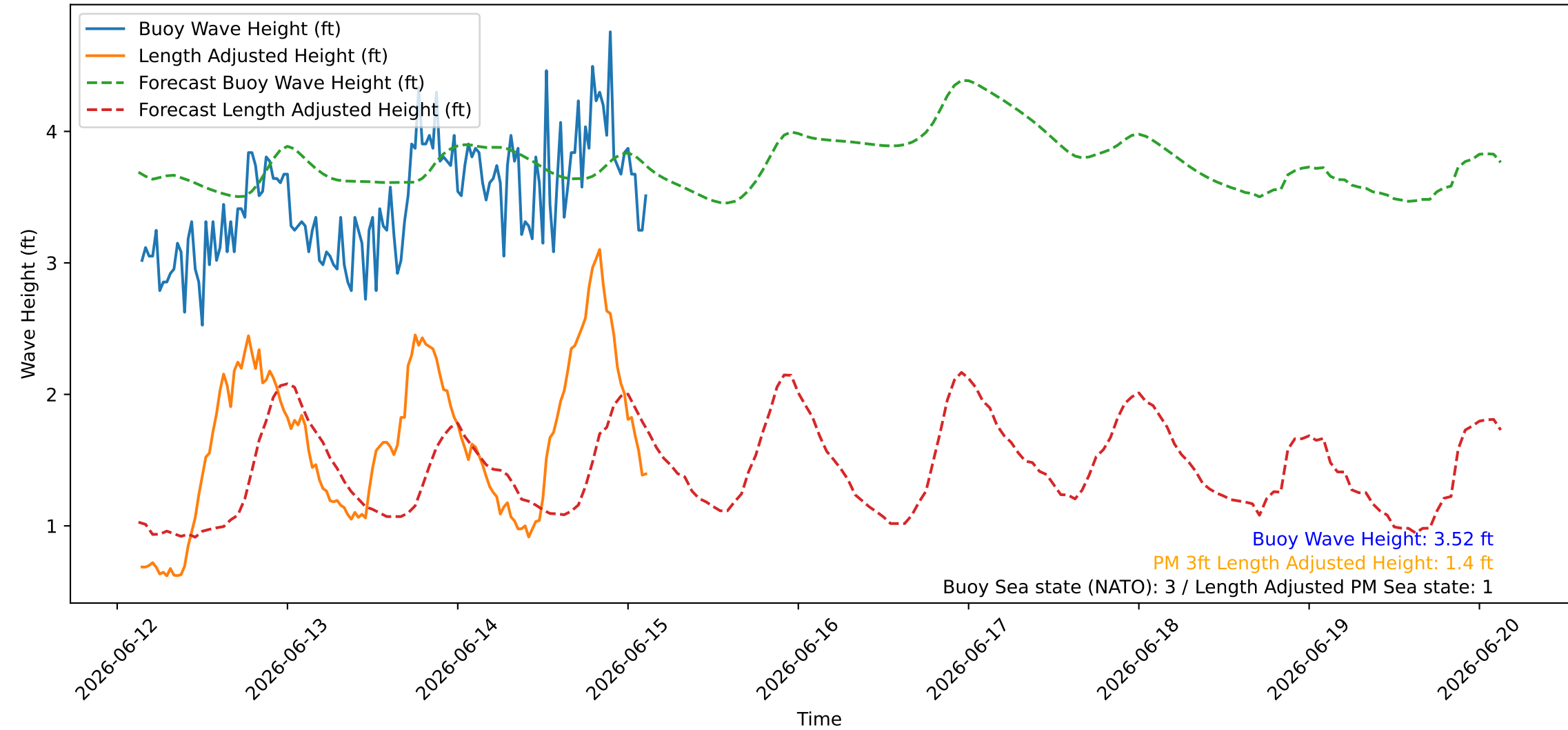
Wave Heights over Time for Red Beach at 2026-06-15 03:20:46
