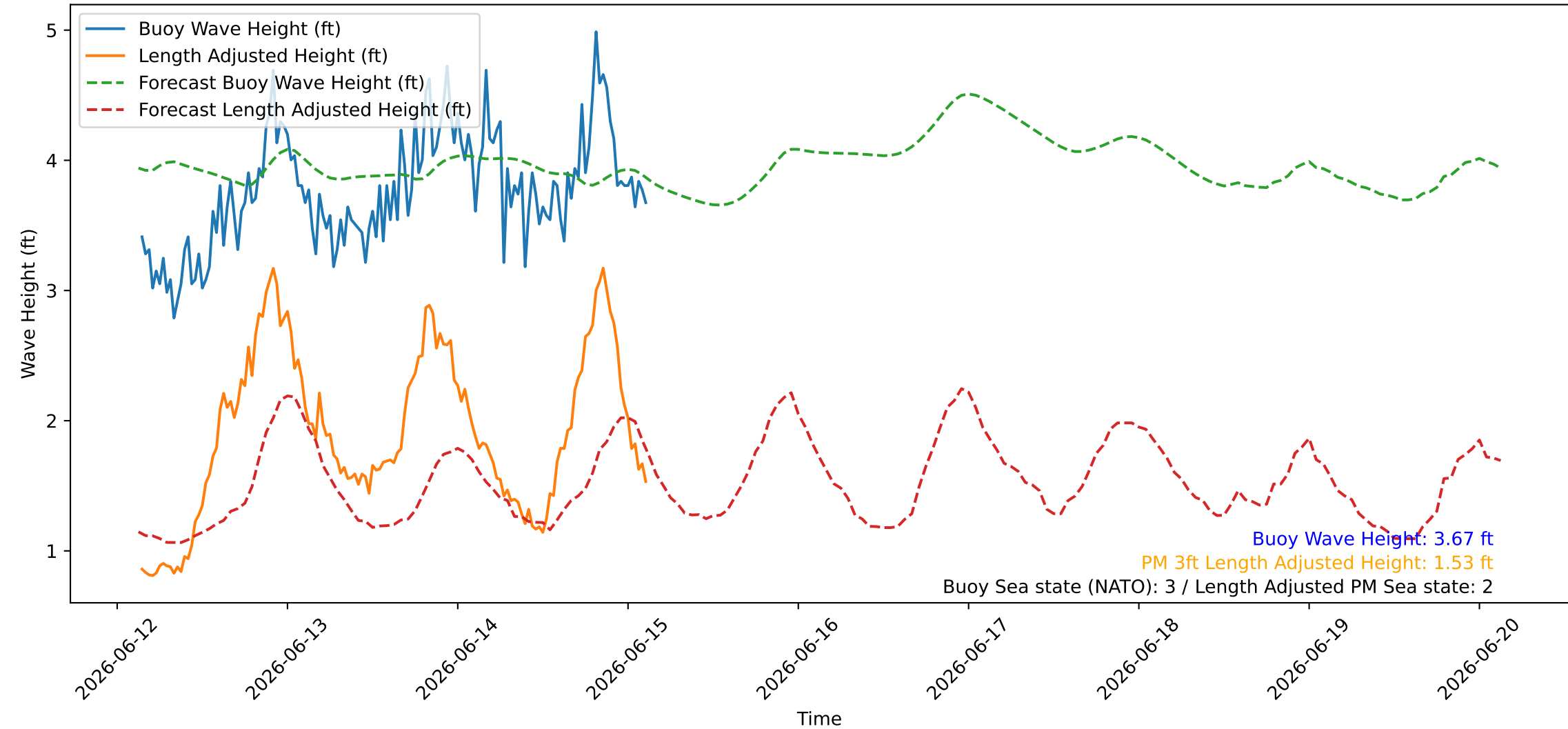
Wave Heights over Time for Oceanside Harbor at 2026-06-15 03:20:25
