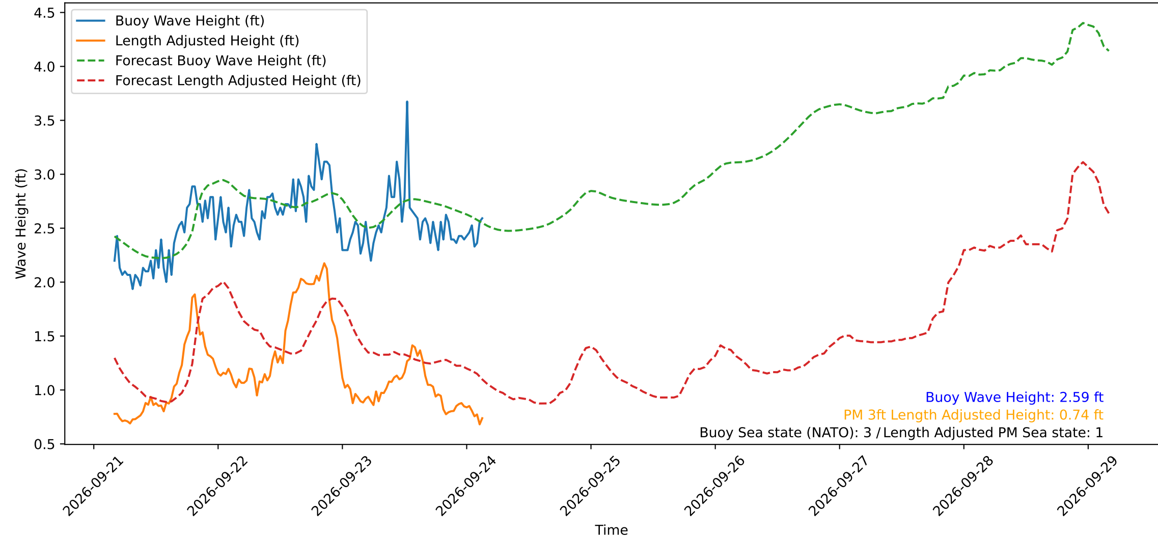
Wave Heights over Time for Red Beach at 2026-09-24 03:50:51
