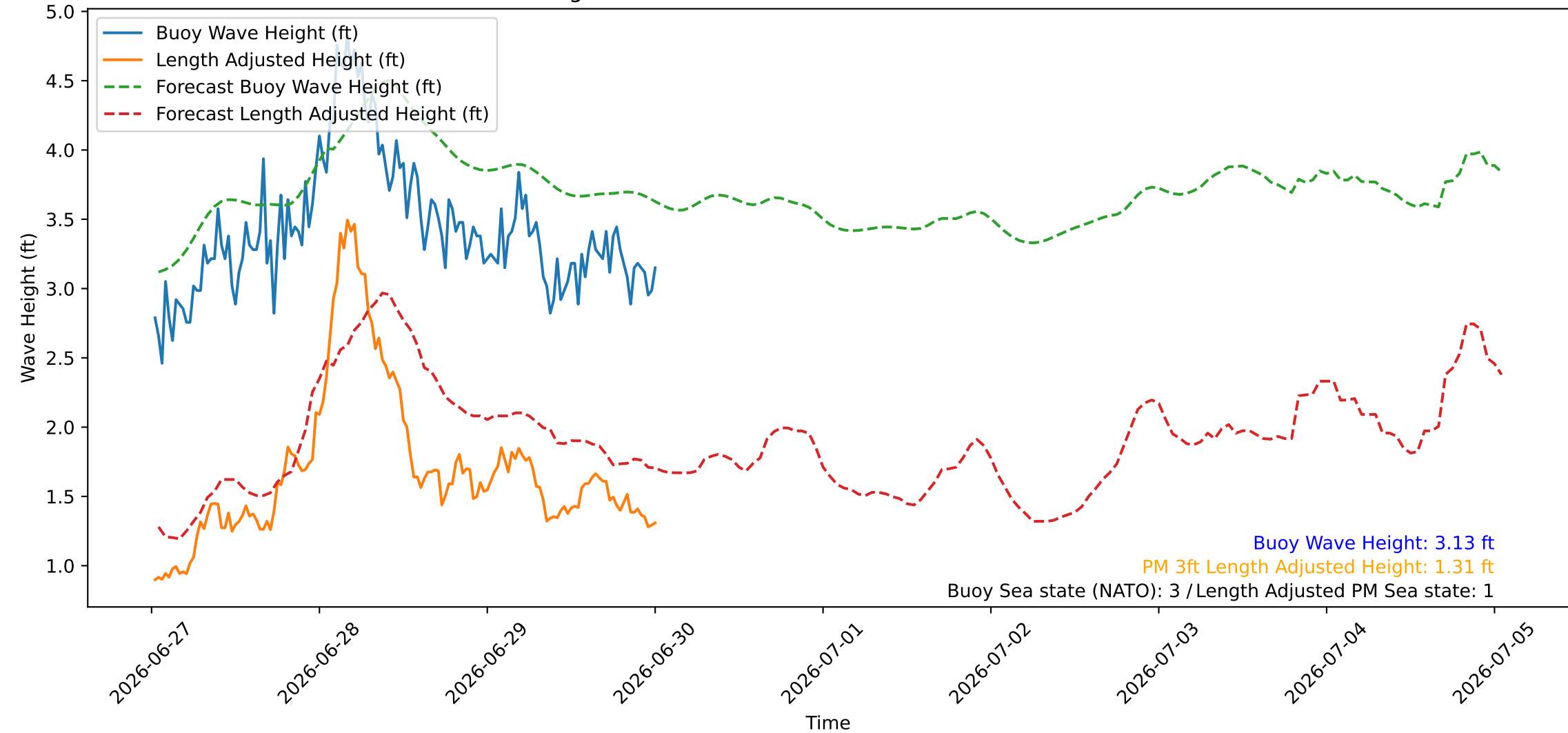
Wave Heights over Time for Green Beach at 2026-06-30 00:41:08
