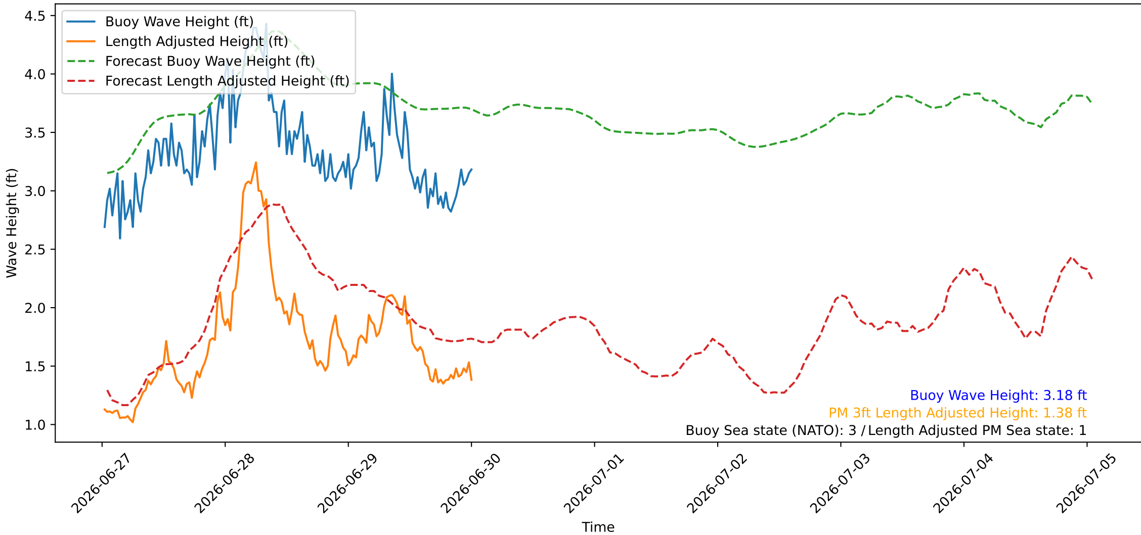
Wave Heights over Time for Oceanside Harbor at 2026-06-30 00:40:26
