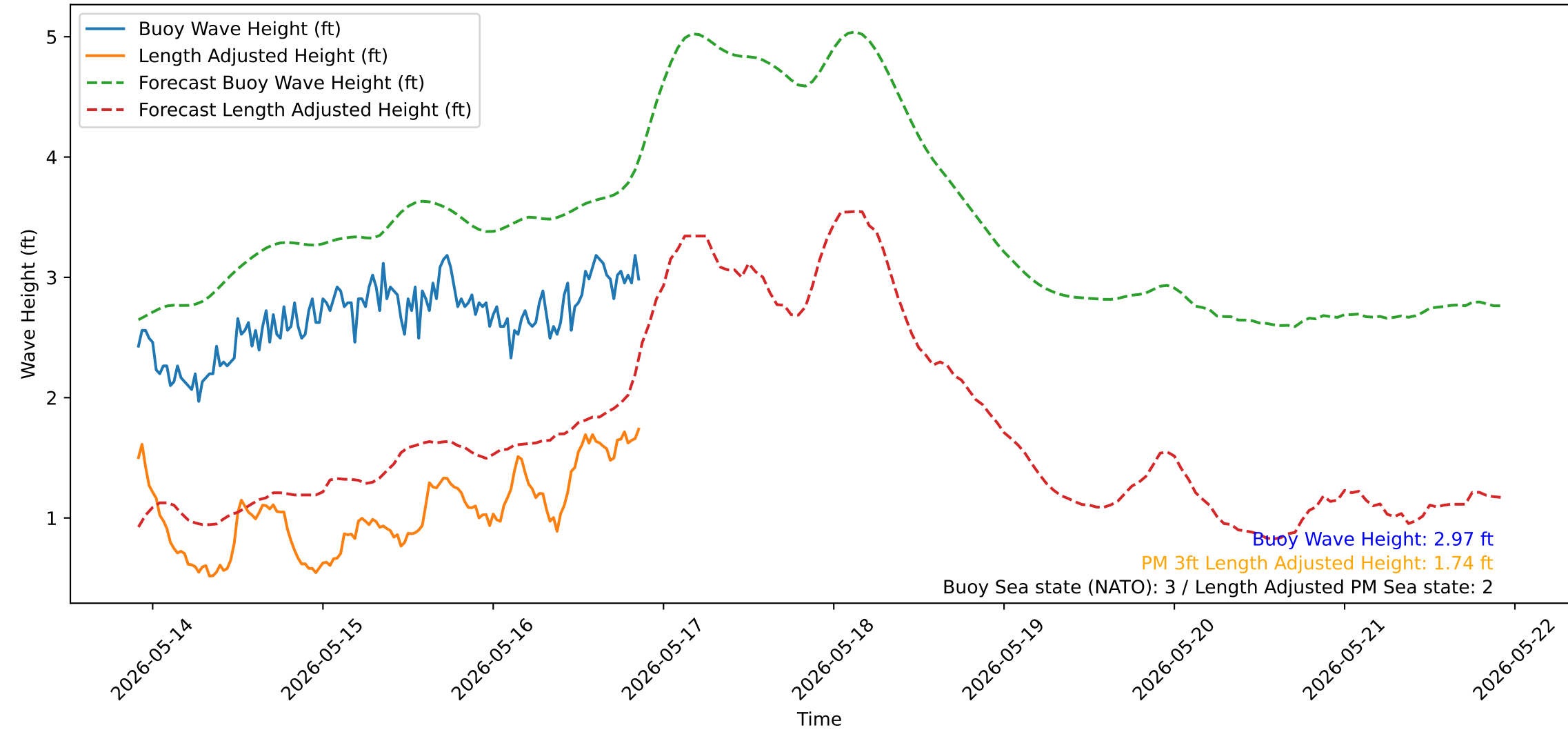
Wave Heights over Time for Red Beach at 2026-05-16 21:40:51
