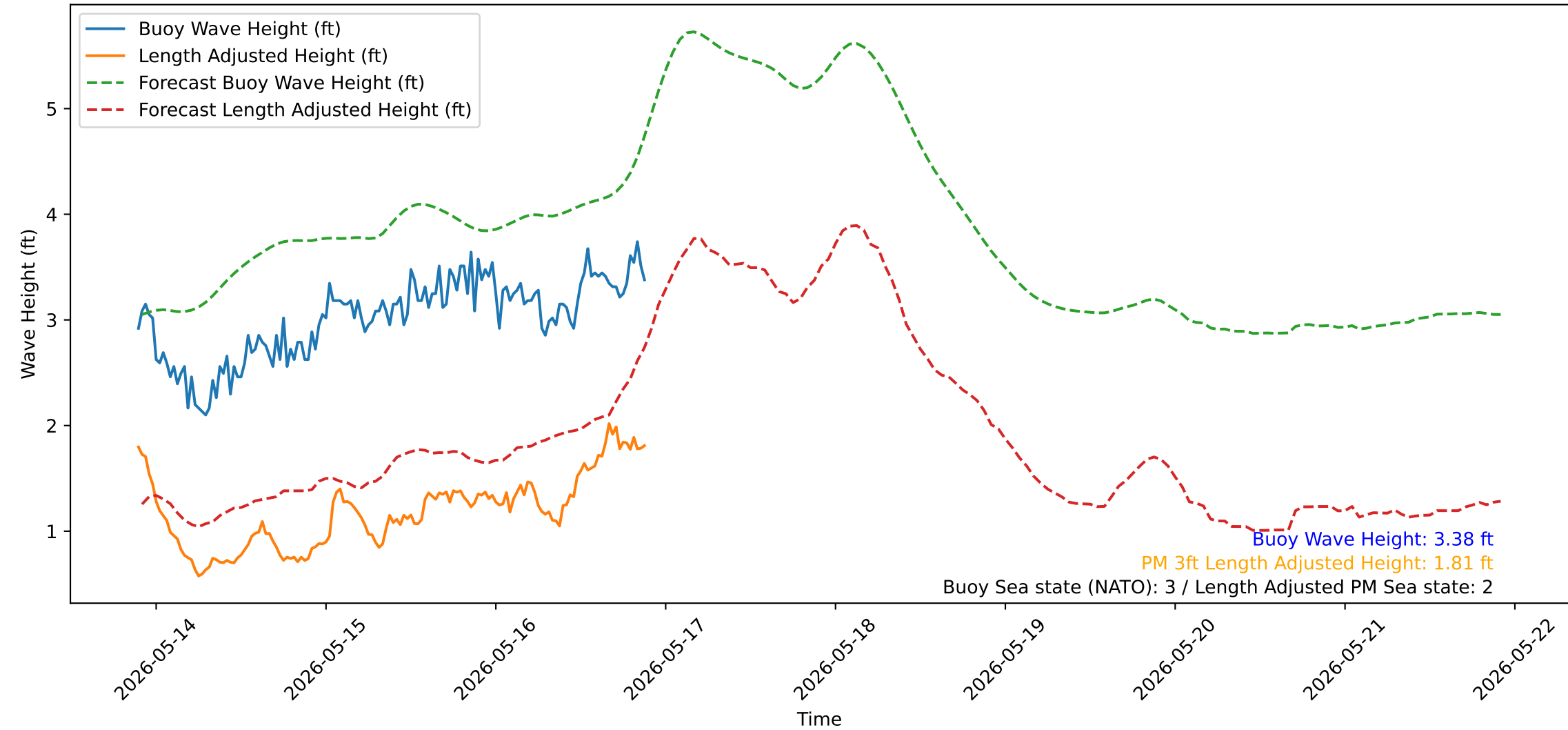
Wave Heights over Time for Green Beach at 2026-05-16 21:41:13
