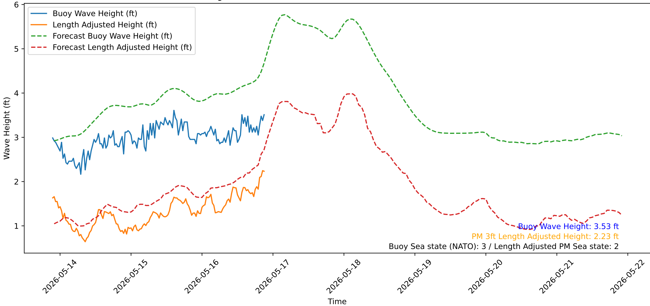
Wave Heights over Time for Oceanside Harbor at 2026-05-16 21:40:31
