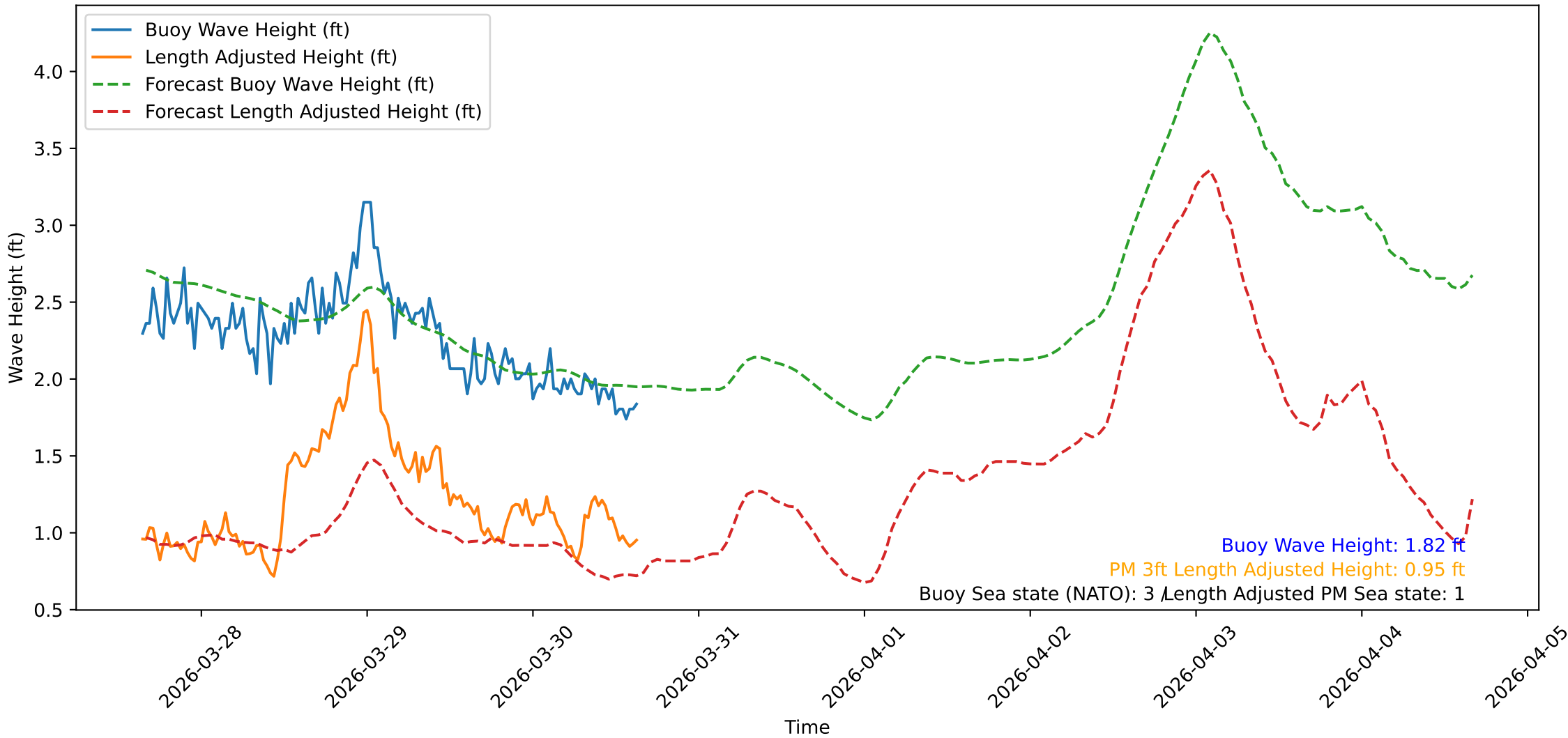
Wave Heights over Time for Oceanside Harbor at 2026-03-30 15:40:31
