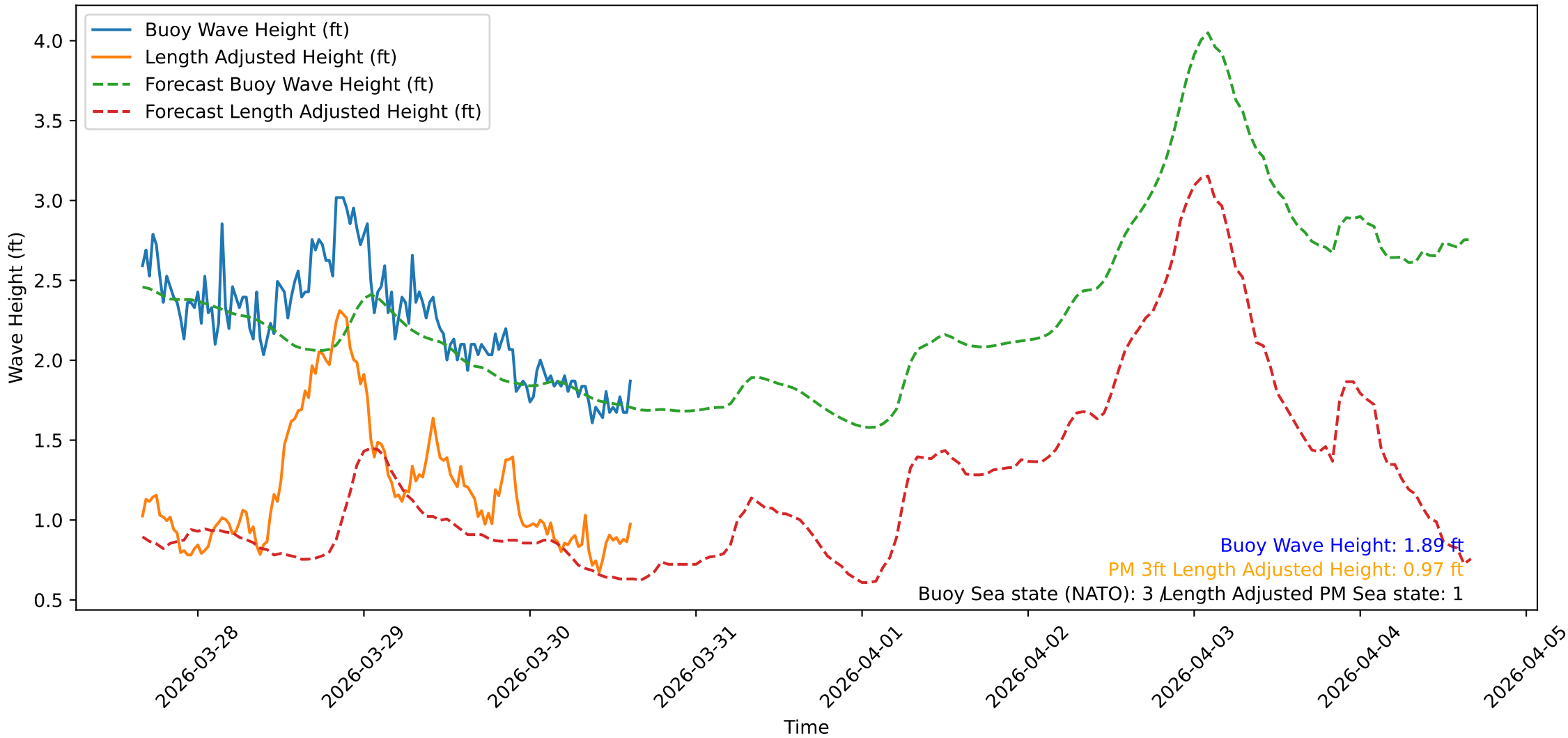
Wave Heights over Time for Red Beach at 2026-03-30 15:40:47
