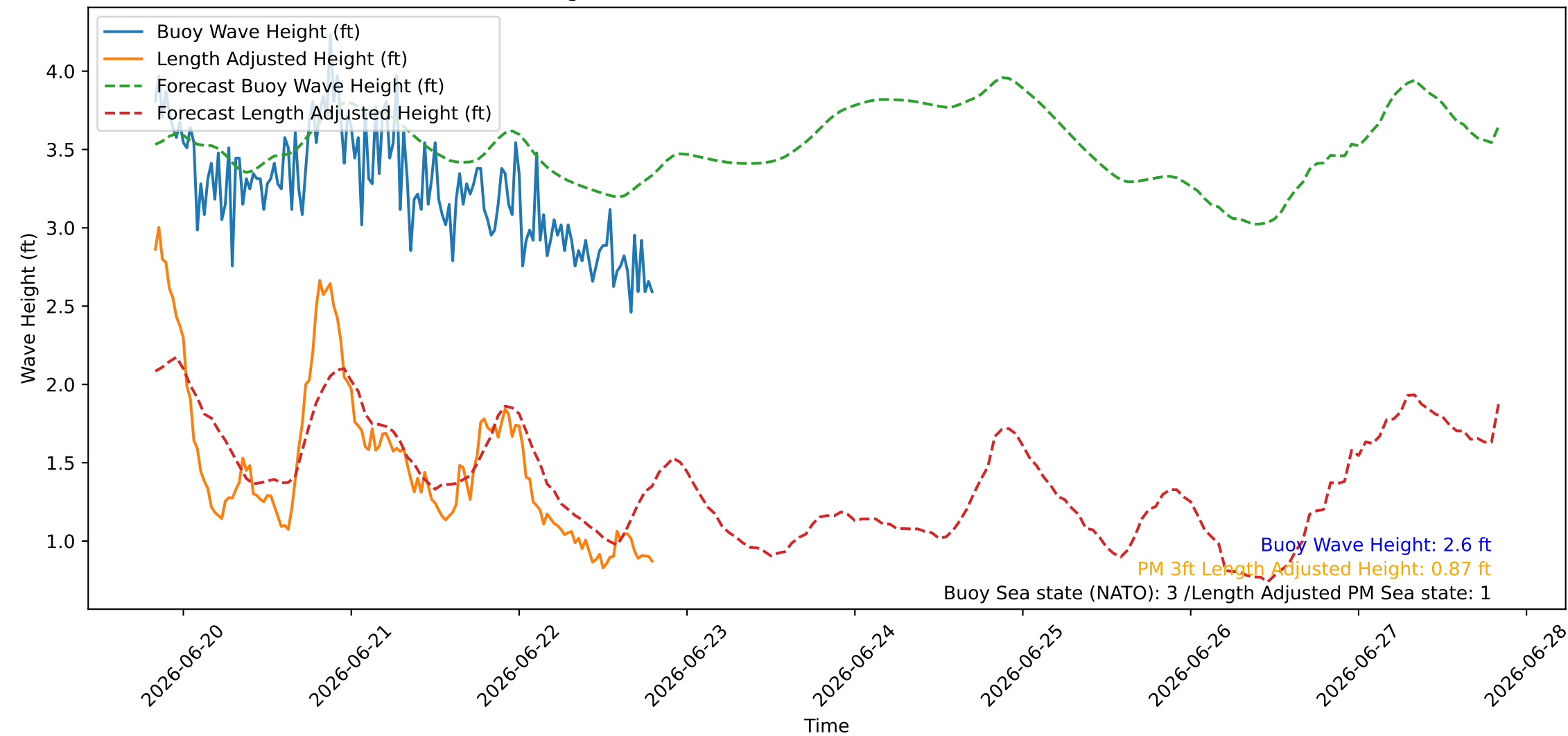
Wave Heights over Time for Green Beach at 2026-06-22 20:01:08
