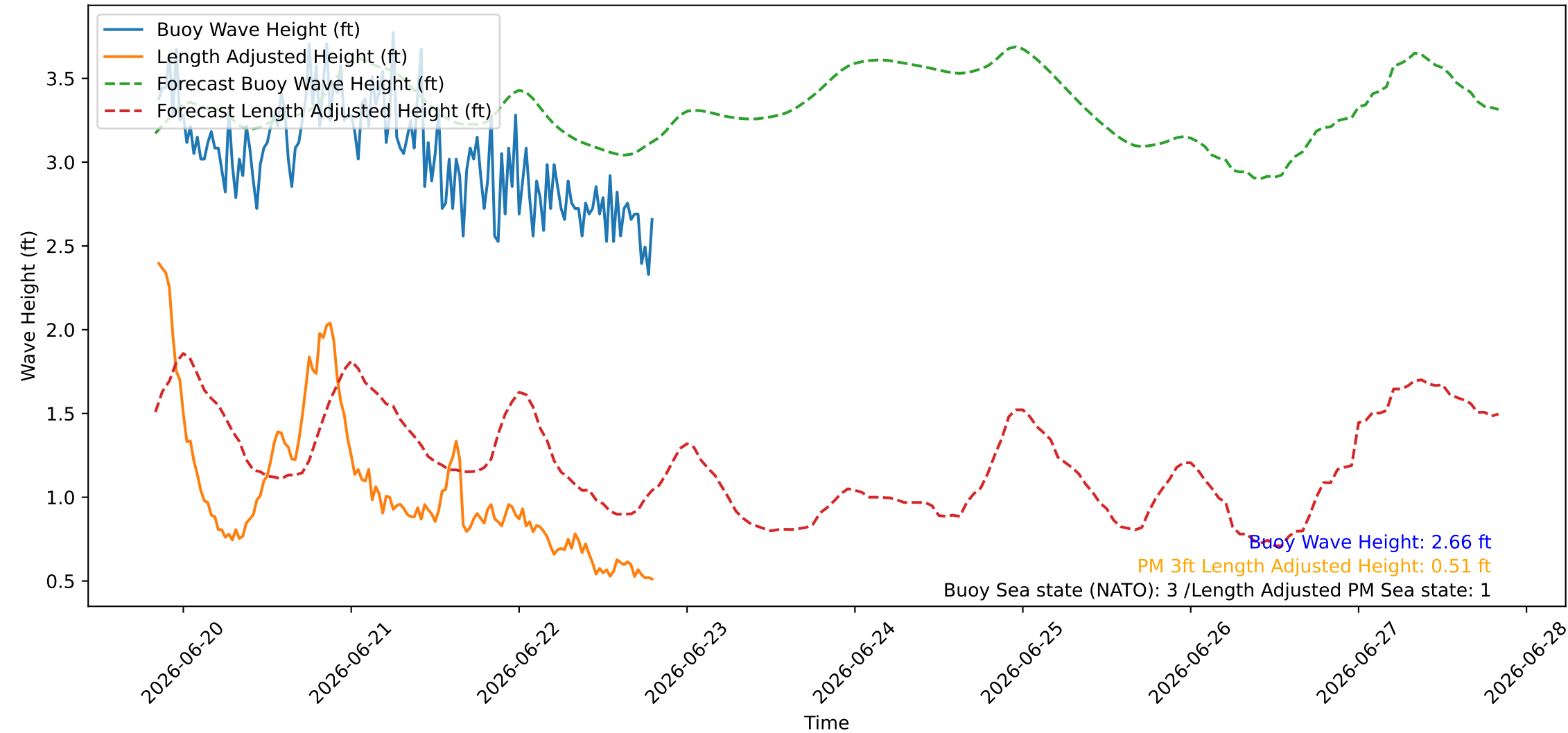
Wave Heights over Time for Red Beach at 2026-06-22 20:00:45
