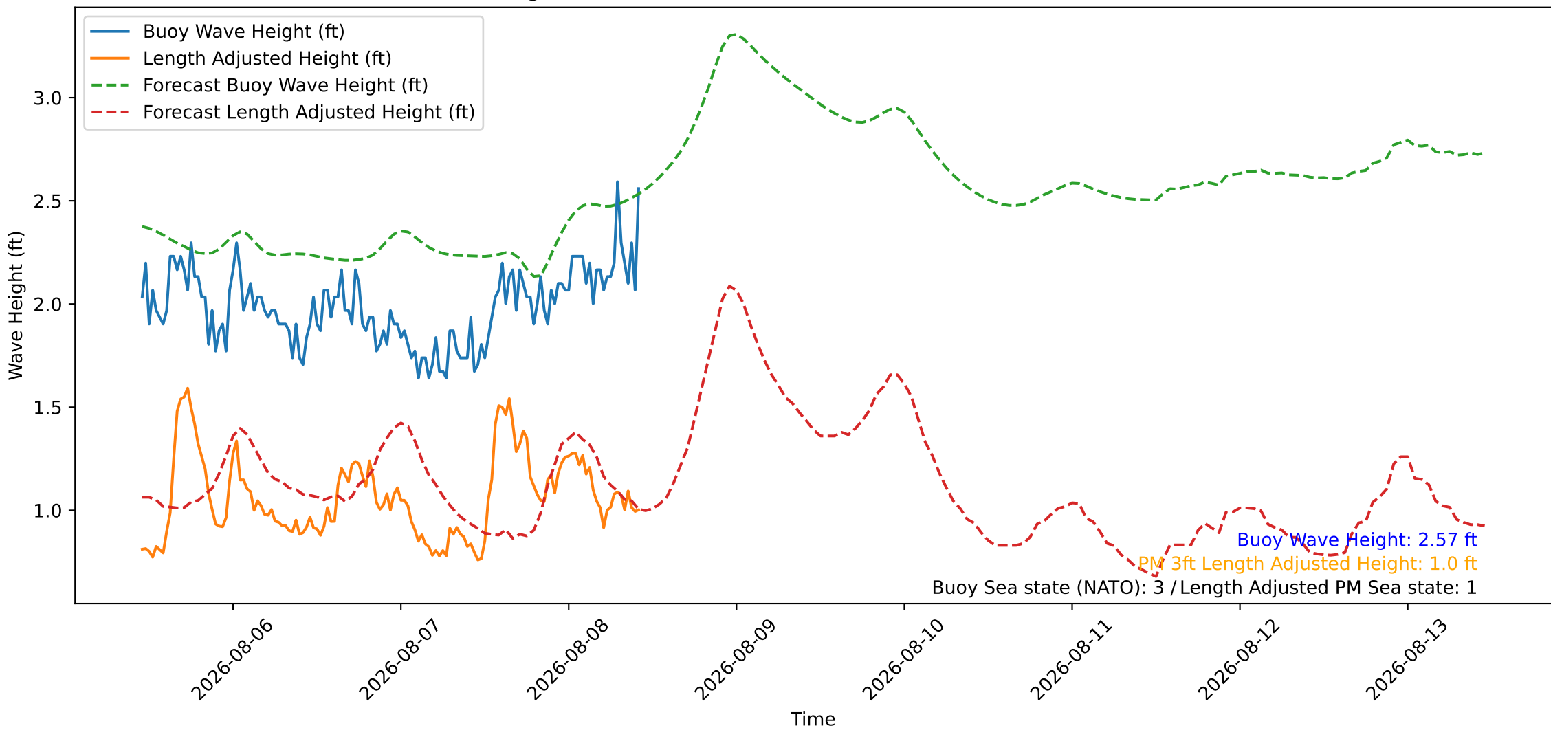
Wave Heights over Time for Oceanside Harbor at 2026-08-08 11:00:26
