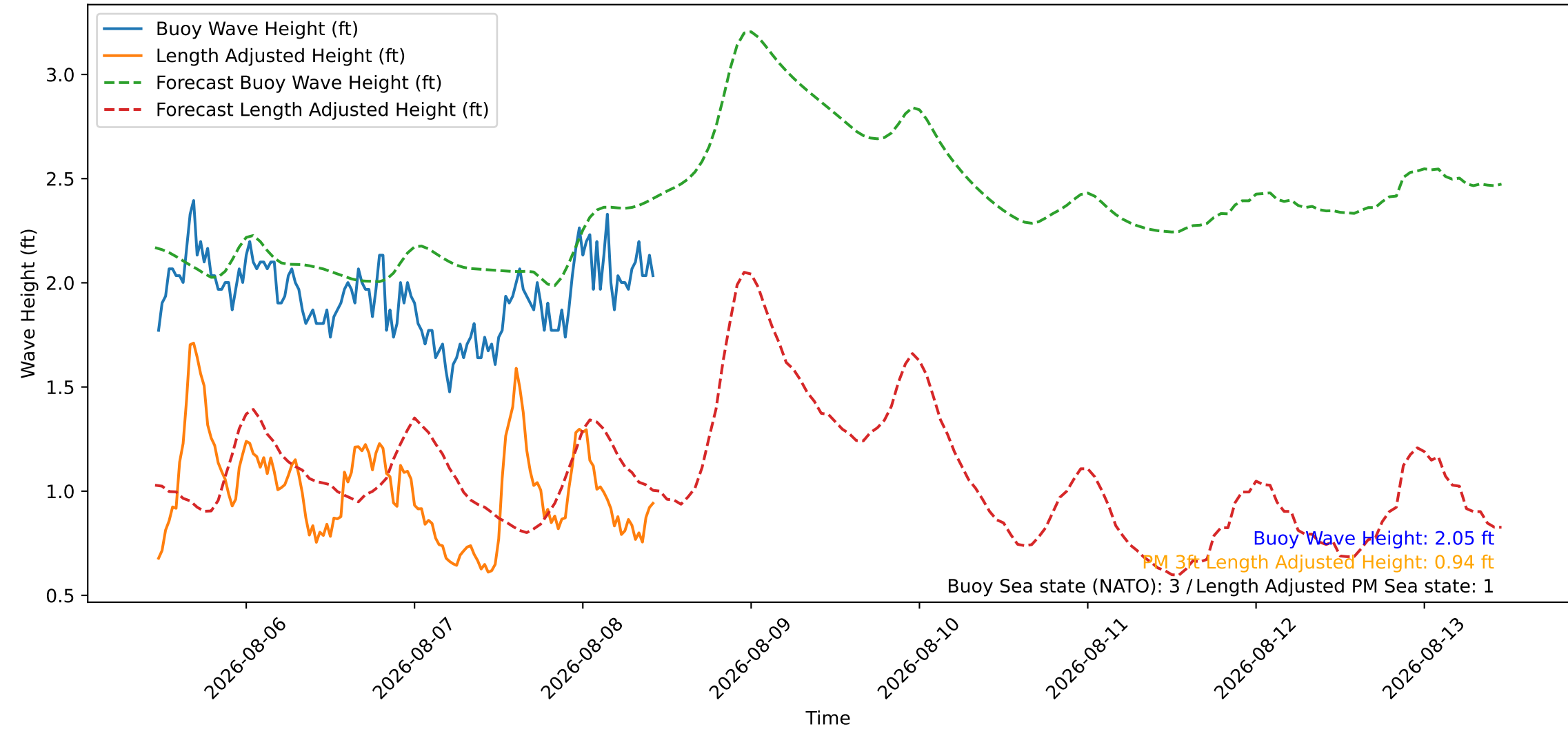
Wave Heights over Time for Red Beach at 2026-08-08 11:00:45
