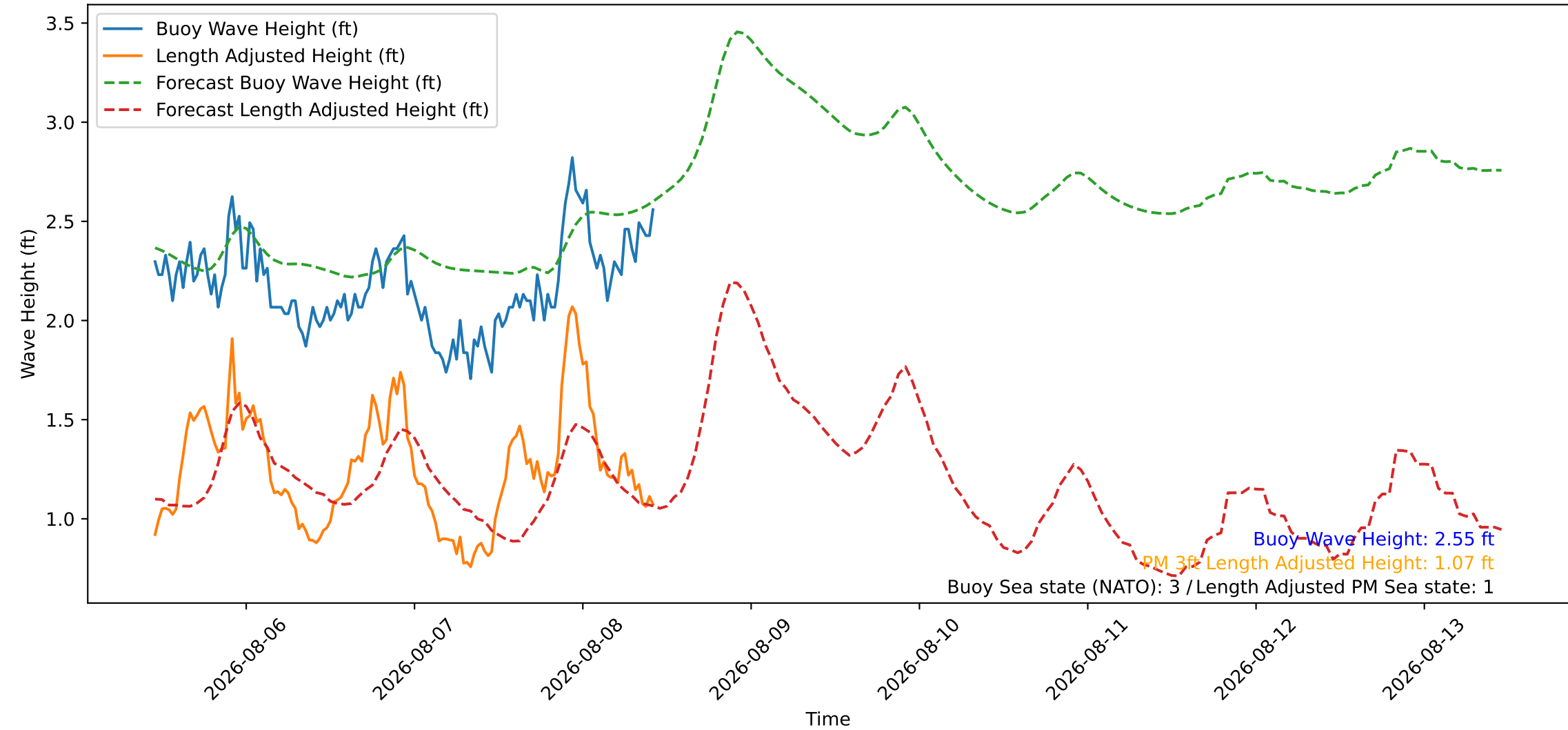
Wave Heights over Time for Green Beach at 2026-08-08 11:01:08
