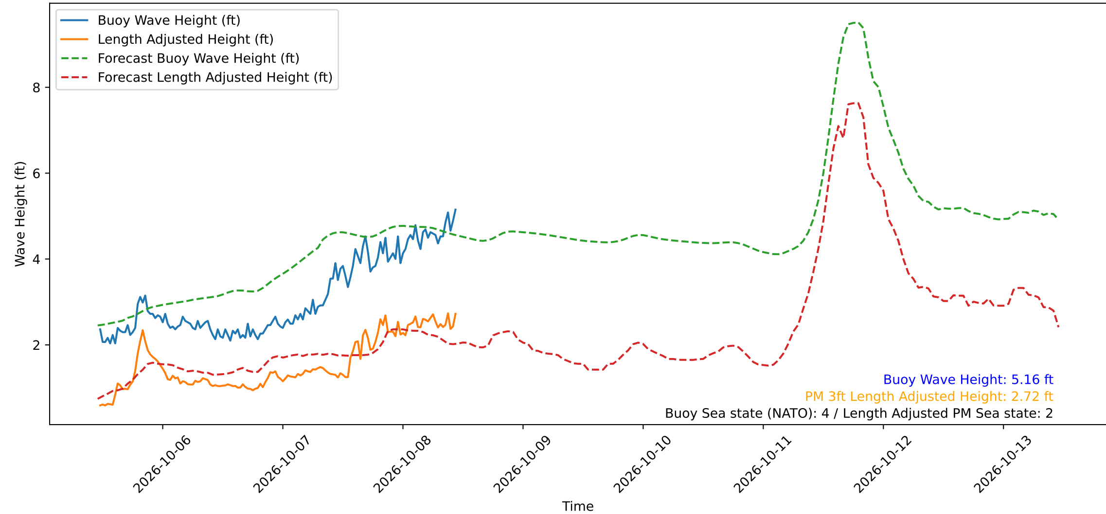
Wave Heights over Time for Green Beach at 2026-10-08 11:11:13
