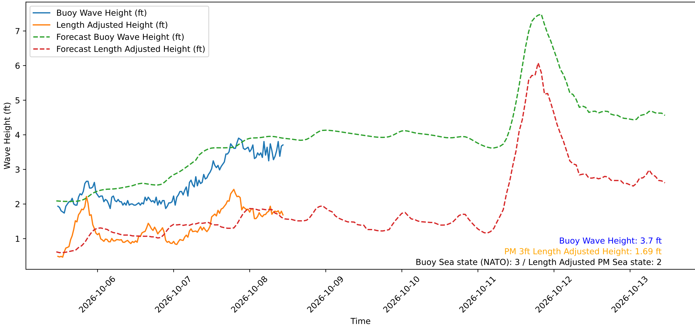
Wave Heights over Time for Red Beach at 2026-10-08 11:10:50
