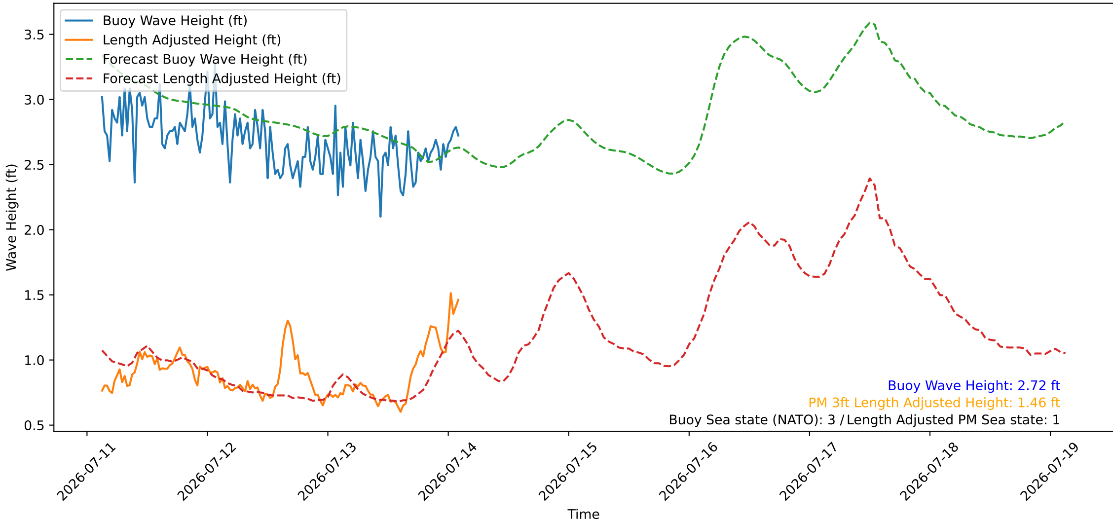
Wave Heights over Time for Oceanside Harbor at 2026-07-14 02:50:26
