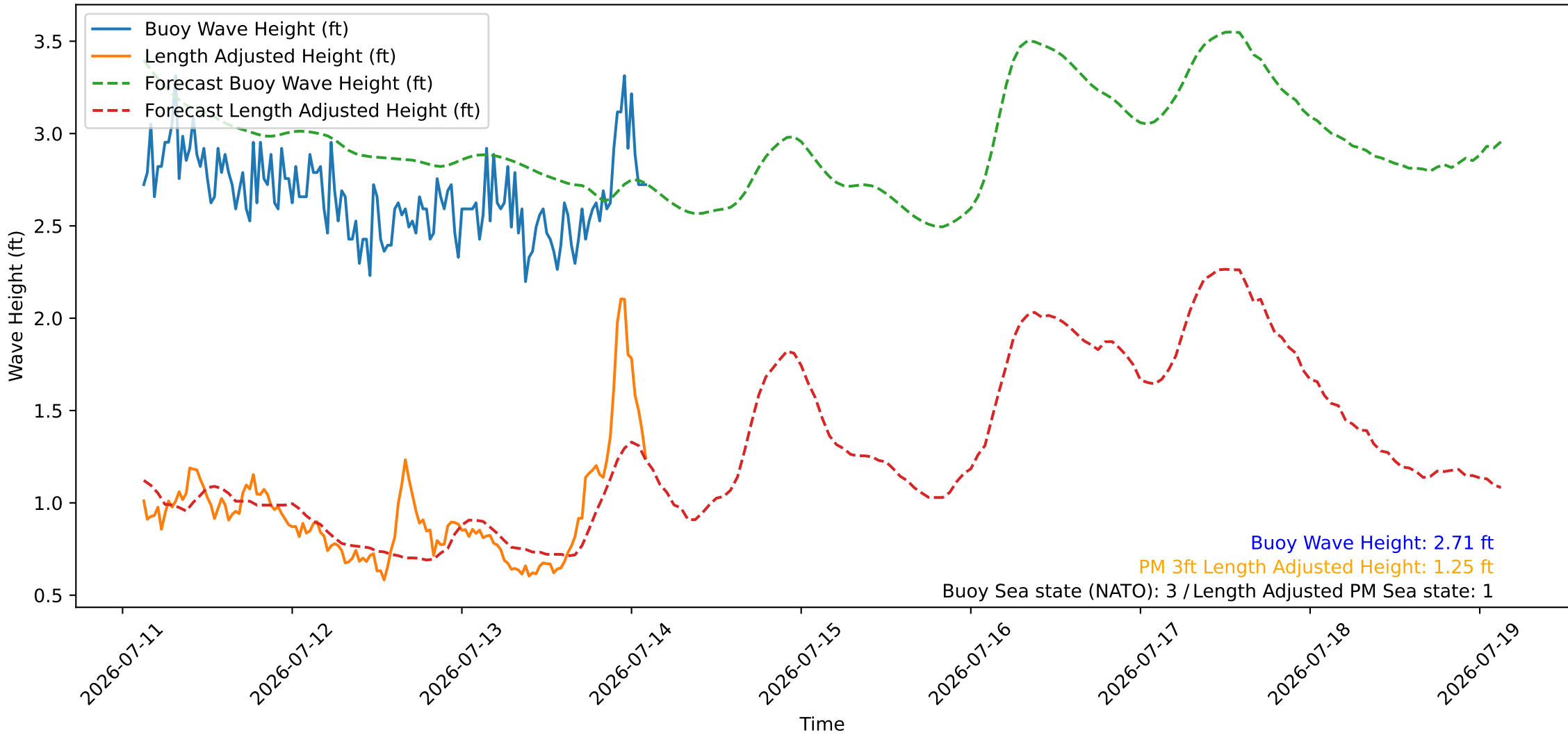
Wave Heights over Time for Green Beach at 2026-07-14 02:51:09
