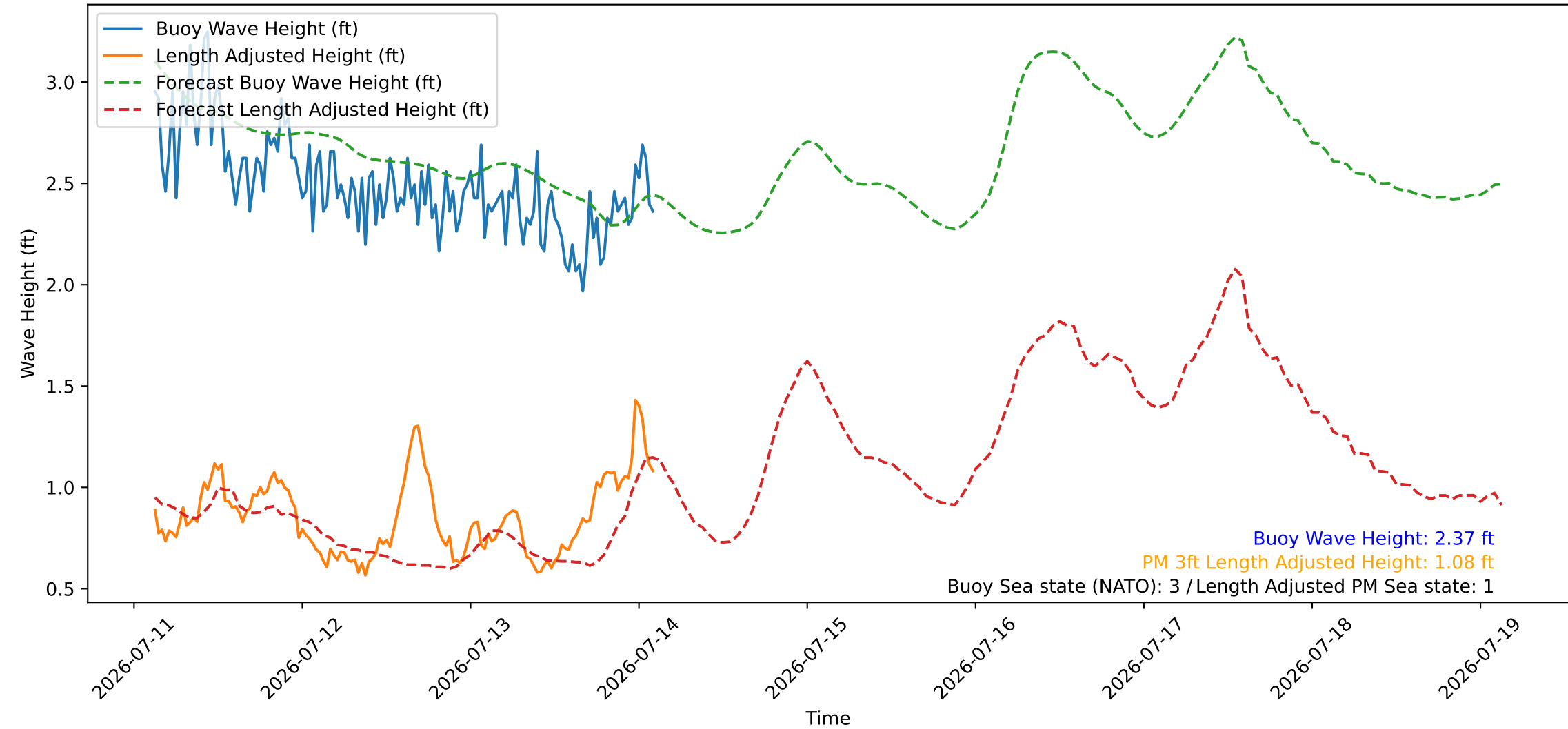
Wave Heights over Time for Red Beach at 2026-07-14 02:50:47
