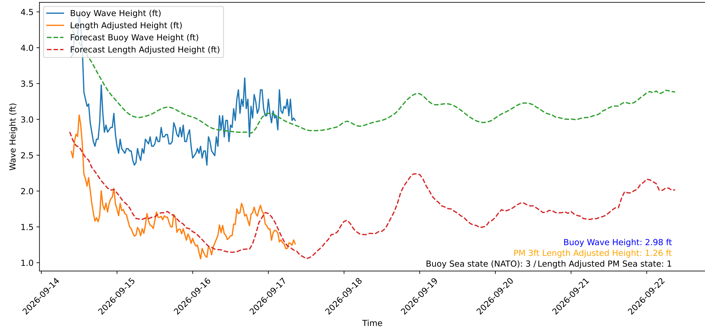
Wave Heights over Time for Oceanside Harbor at 2026-09-17 09:20:29
