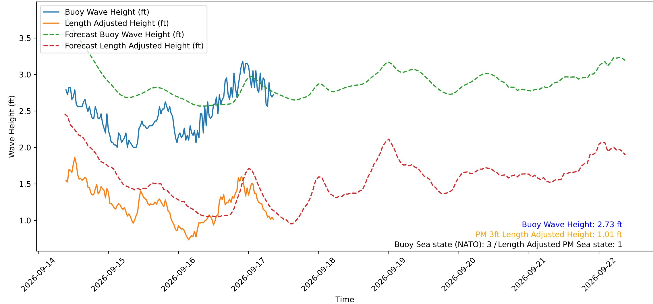
Wave Heights over Time for Red Beach at 2026-09-17 09:20:50
