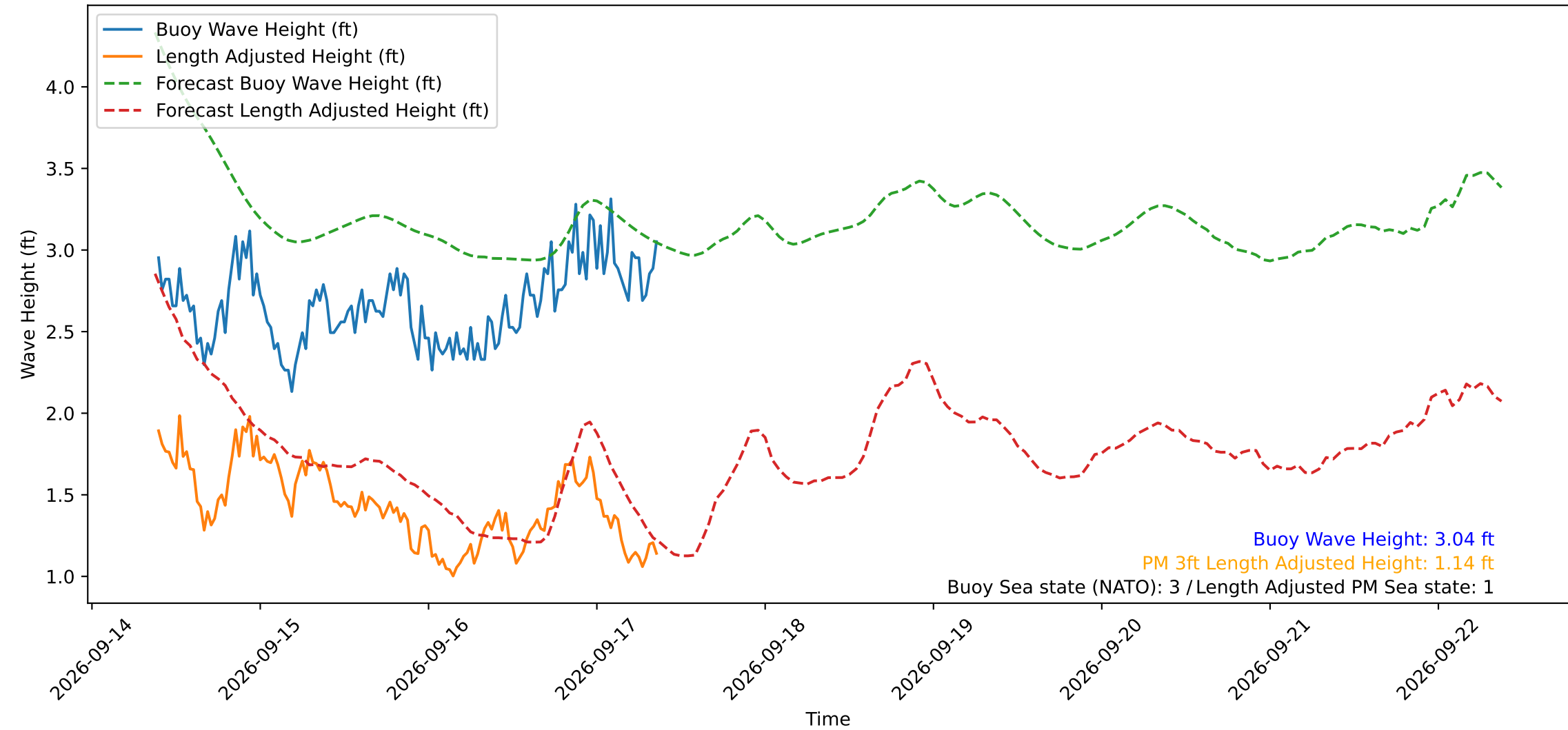
Wave Heights over Time for Green Beach at 2026-09-17 09:21:14
