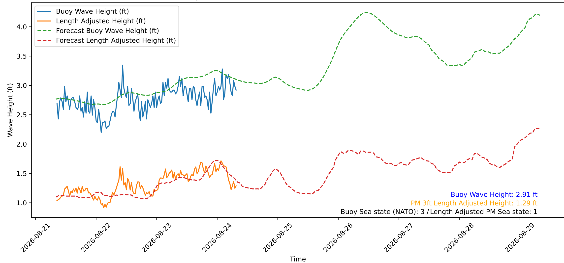
Wave Heights over Time for Oceanside Harbor at 2026-08-24 08:20:39
