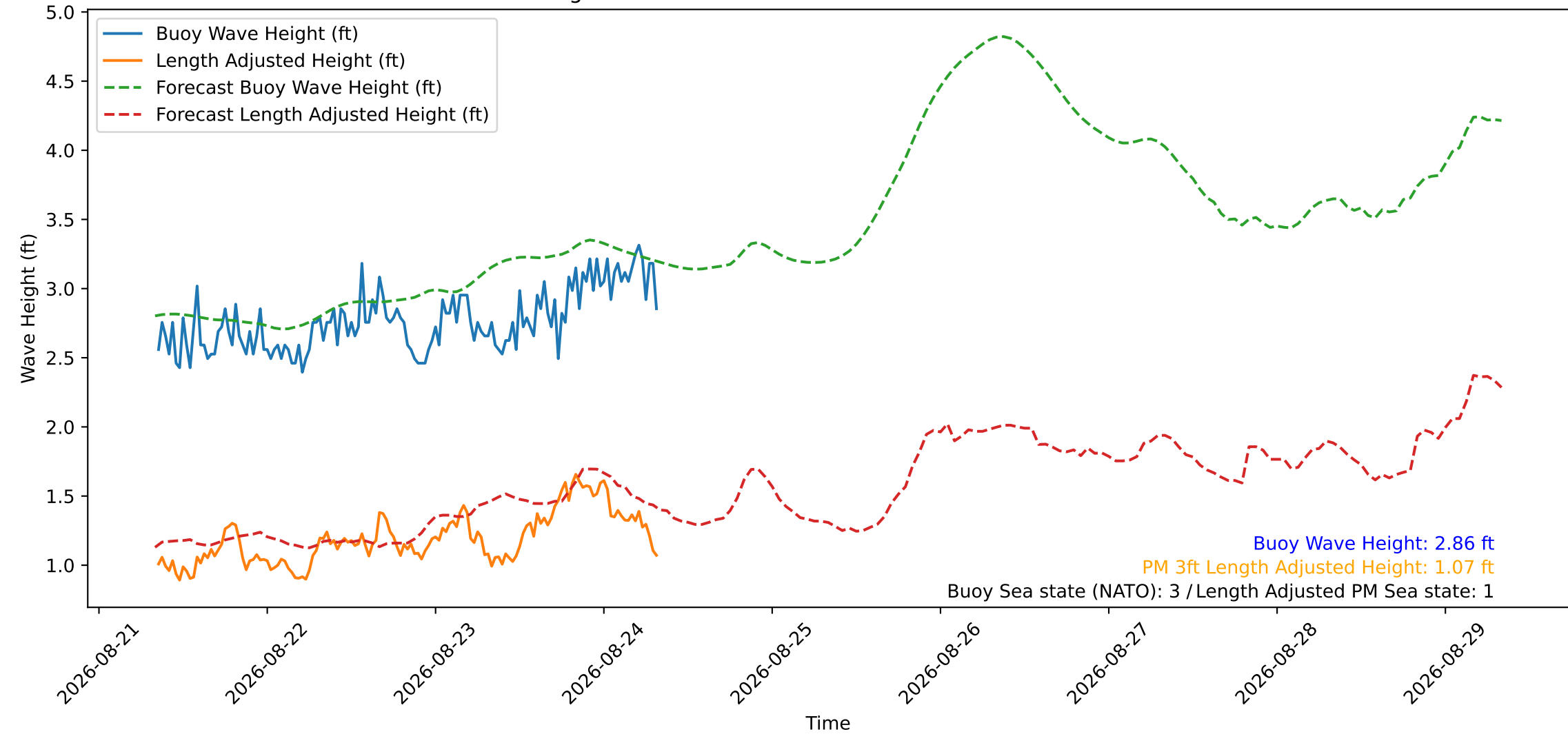
Wave Heights over Time for Green Beach at 2026-08-24 08:21:24
