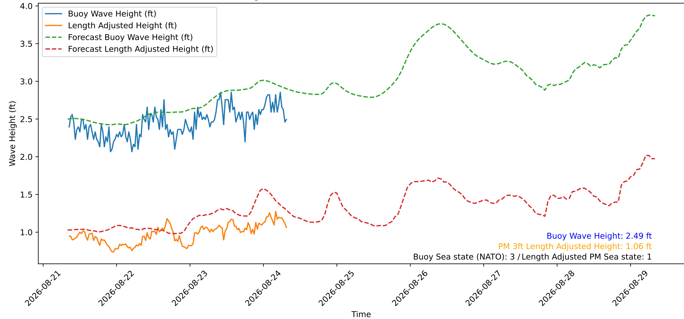
Wave Heights over Time for Red Beach at 2026-08-24 08:21:00
