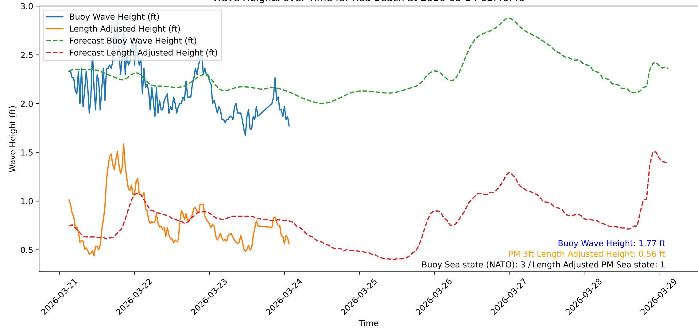
Wave Heights over Time for Red Beach at 2026-03-24 02:40:48
