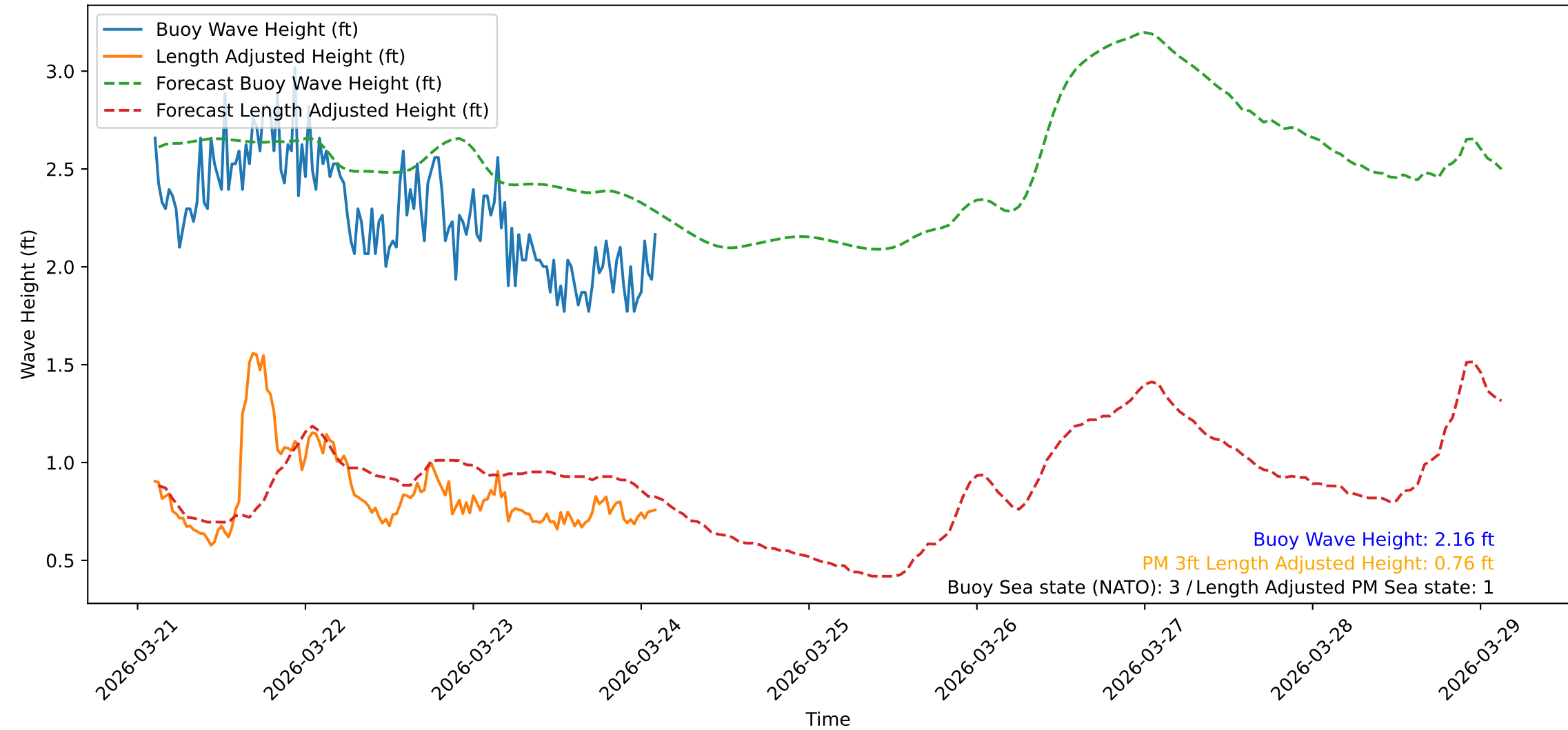
Wave Heights over Time for Oceanside Harbor at 2026-03-24 02:40:32
