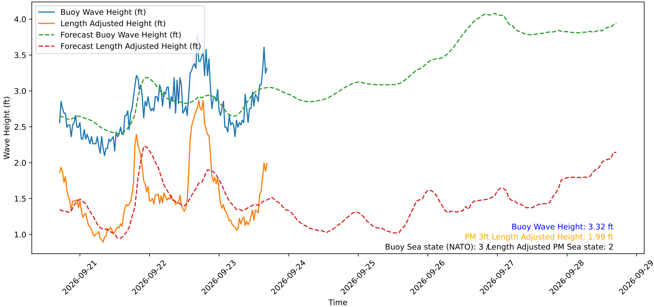
Wave Heights over Time for Oceanside Harbor at 2026-09-23 17:10:30
