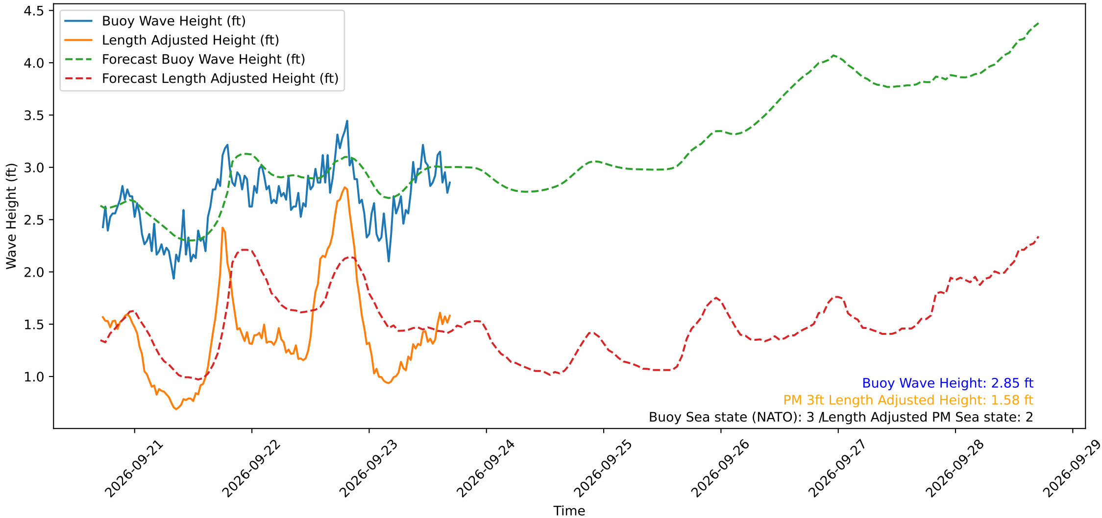
Wave Heights over Time for Green Beach at 2026-09-23 17:11:12
