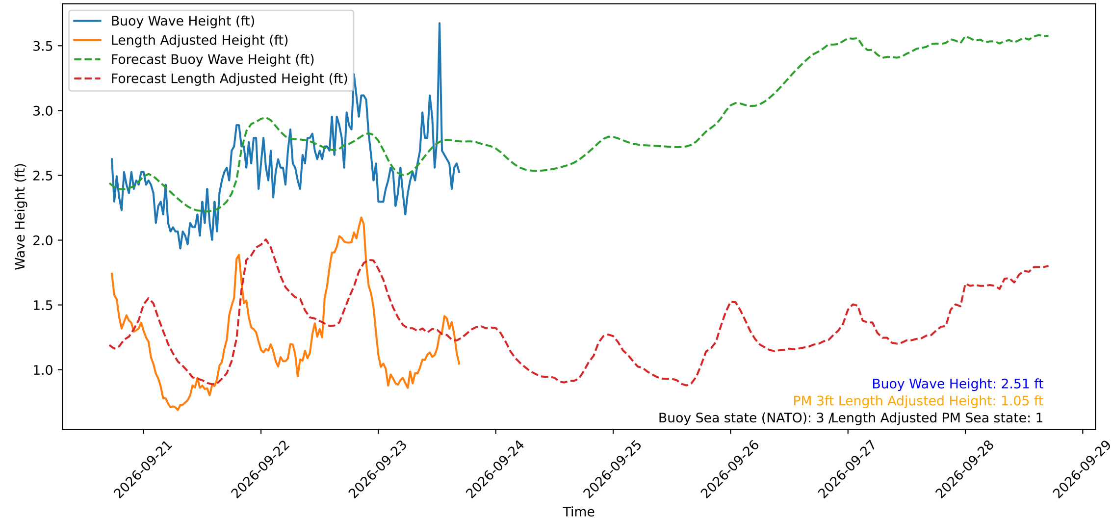
Wave Heights over Time for Red Beach at 2026-09-23 17:10:50
