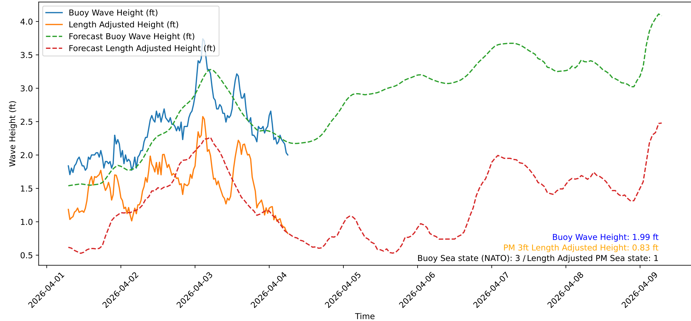
Wave Heights over Time for Red Beach at 2026-04-04 06:50:47
