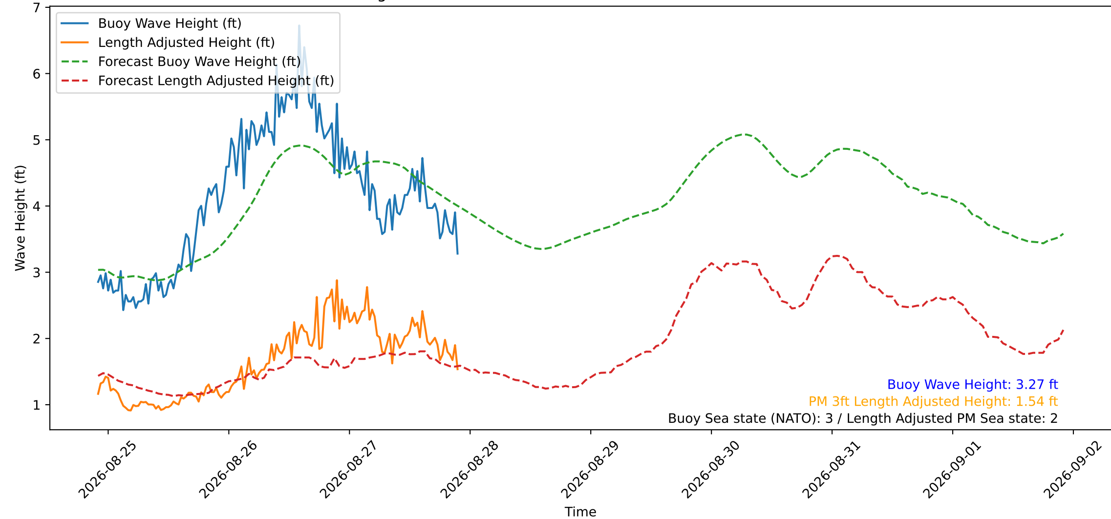
Wave Heights over Time for Oceanside Harbor at 2026-08-27 22:10:29
