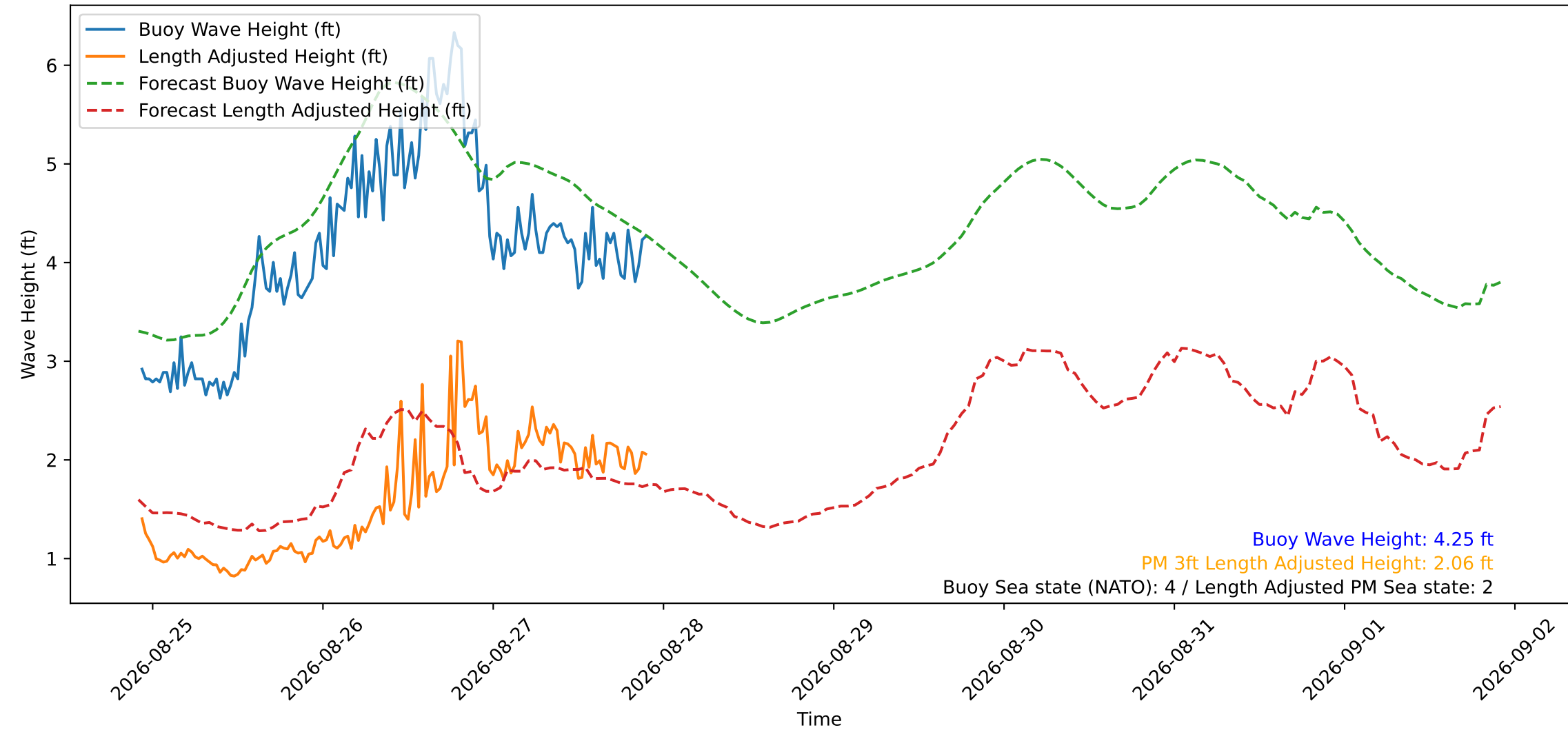
Wave Heights over Time for Green Beach at 2026-08-27 22:11:13
