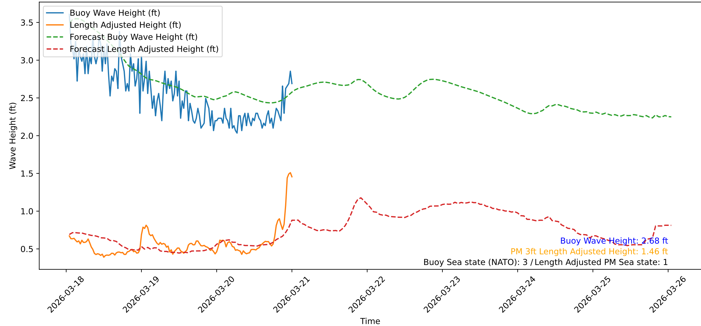
Wave Heights over Time for Green Beach at 2026-03-21 00:51:10
