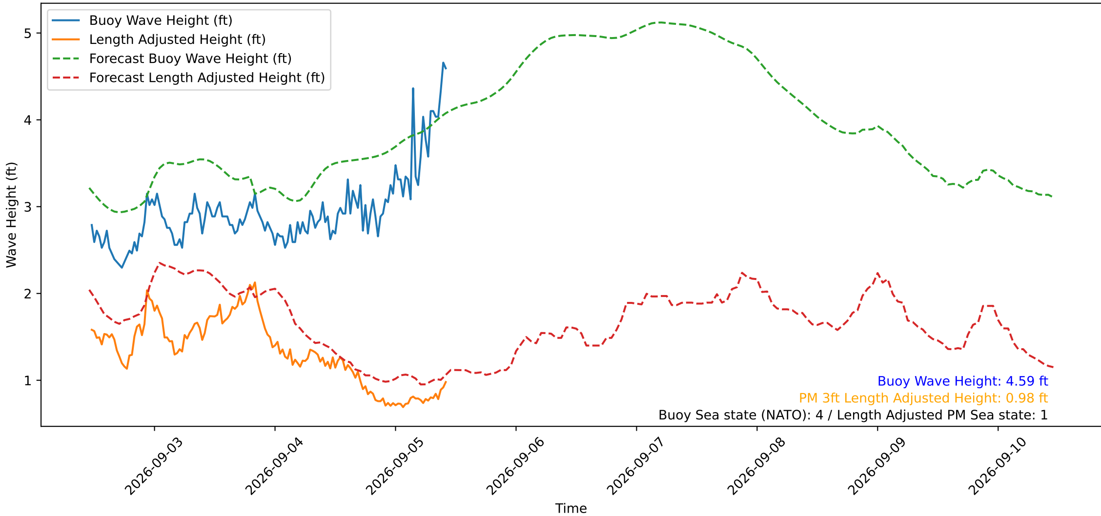
Wave Heights over Time for Red Beach at 2026-09-05 11:00:50
