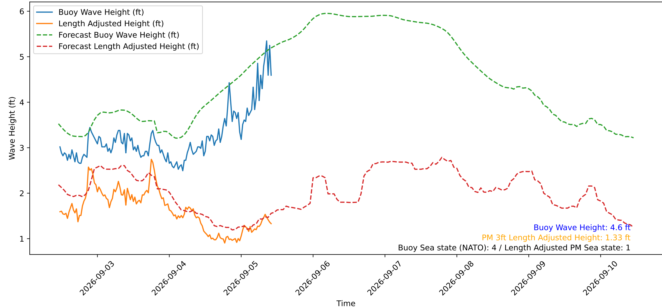
Wave Heights over Time for Green Beach at 2026-09-05 11:01:13
