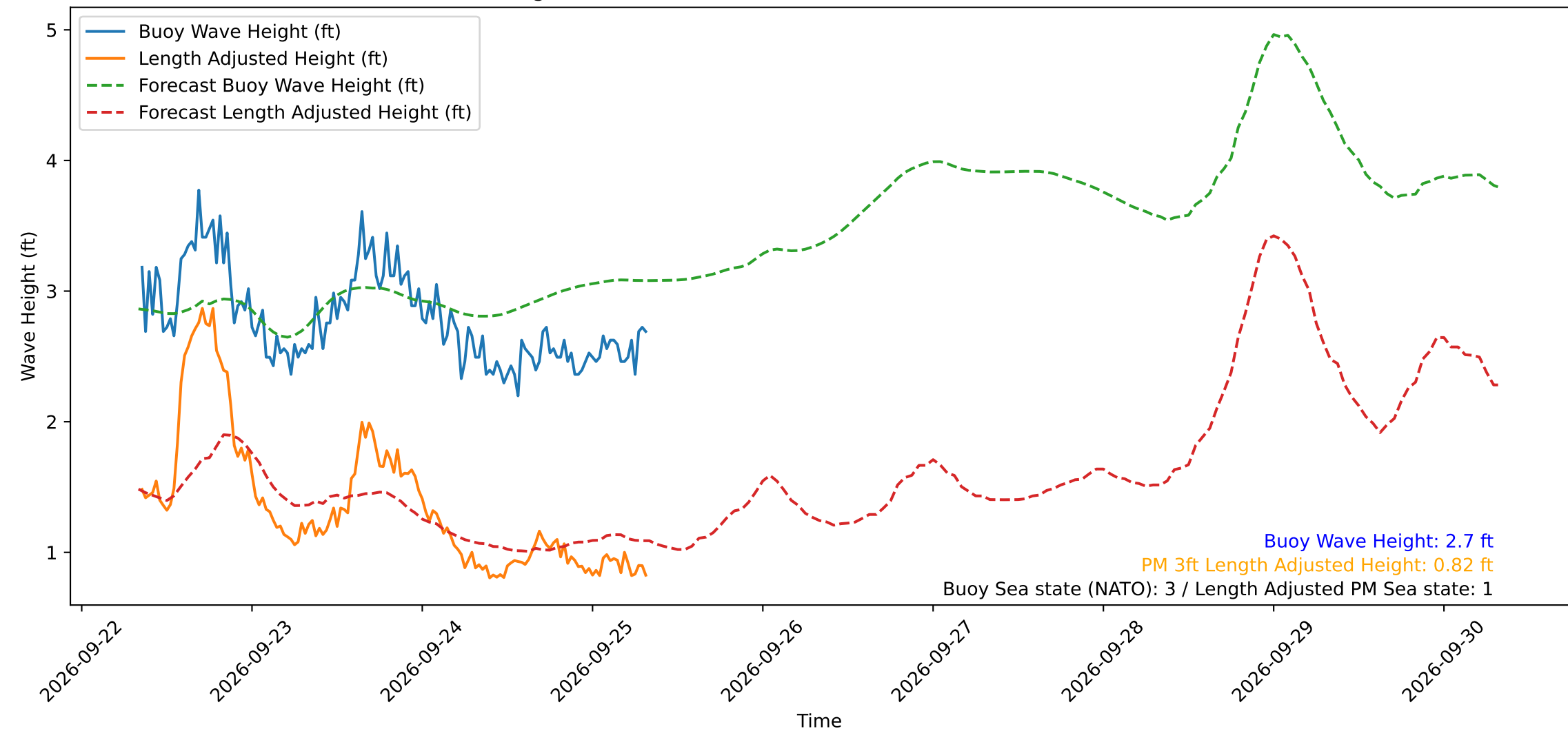
Wave Heights over Time for Oceanside Harbor at 2026-09-25 08:20:29
