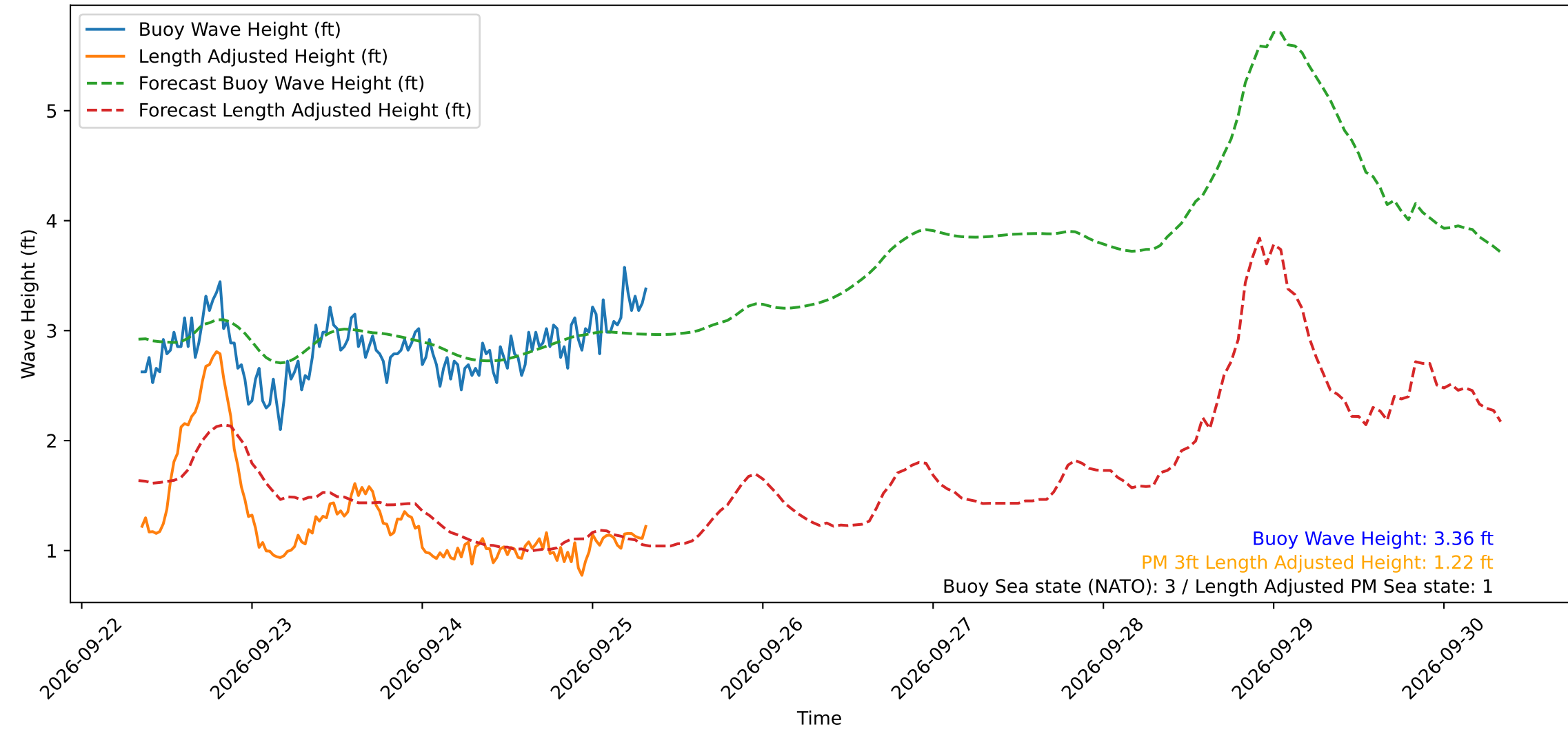
Wave Heights over Time for Green Beach at 2026-09-25 08:21:13
