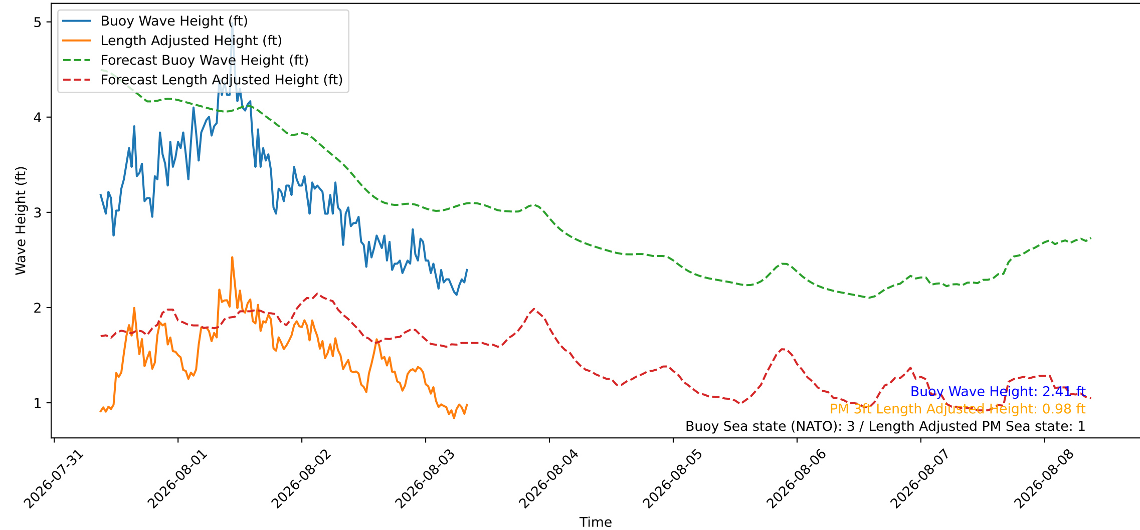
Wave Heights over Time for Green Beach at 2026-08-03 08:51:10
