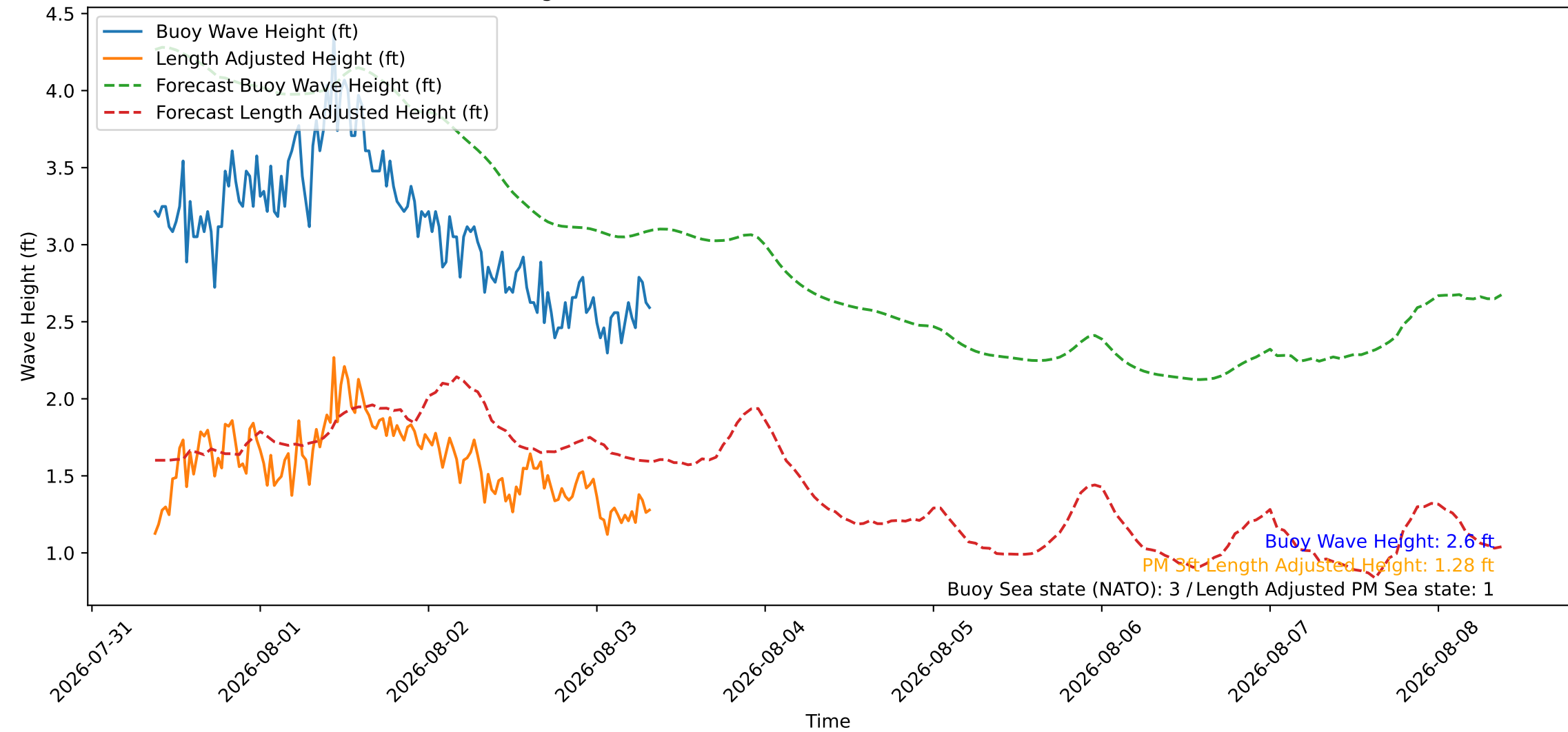
Wave Heights over Time for Oceanside Harbor at 2026-08-03 08:50:27
