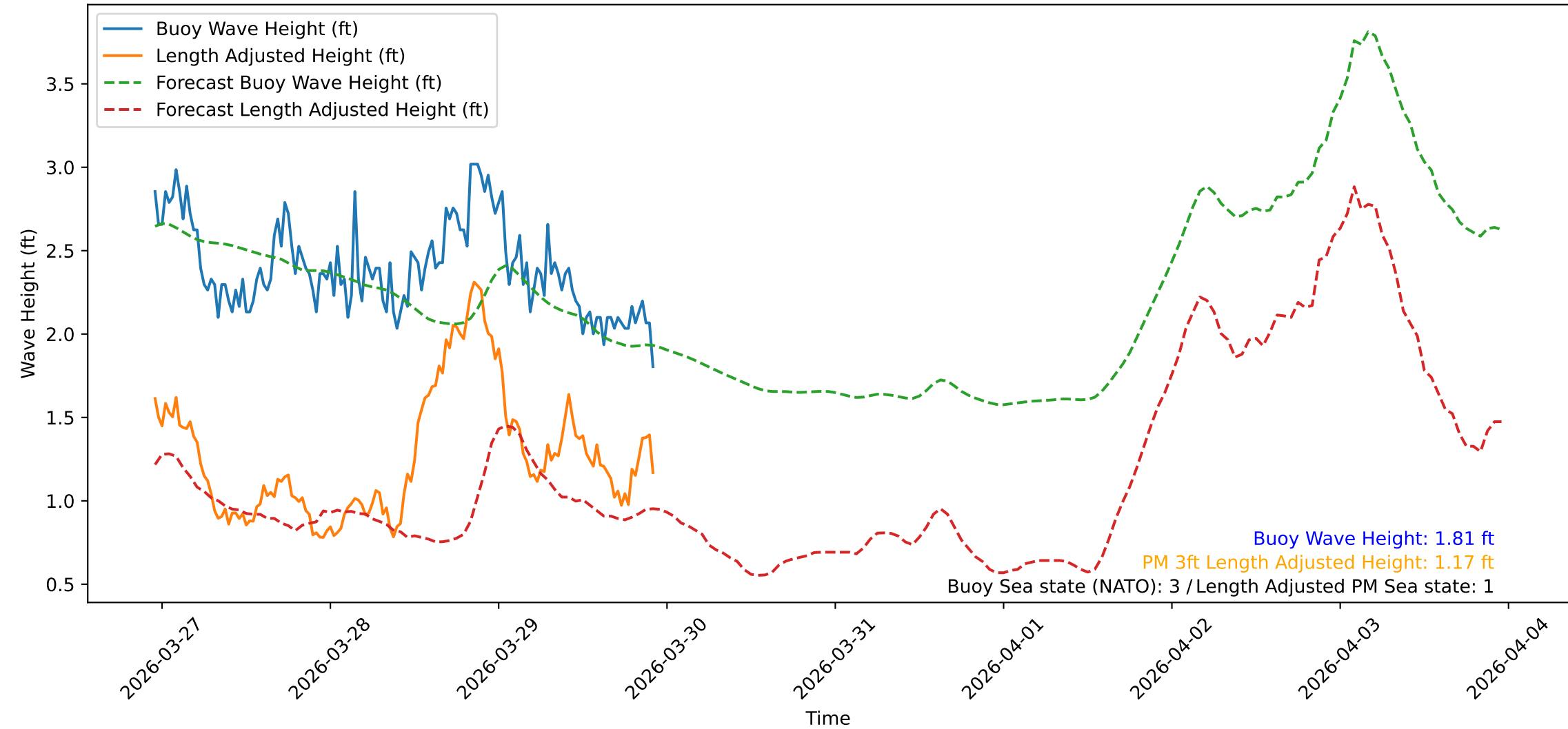
Wave Heights over Time for Red Beach at 2026-03-29 22:40:48
