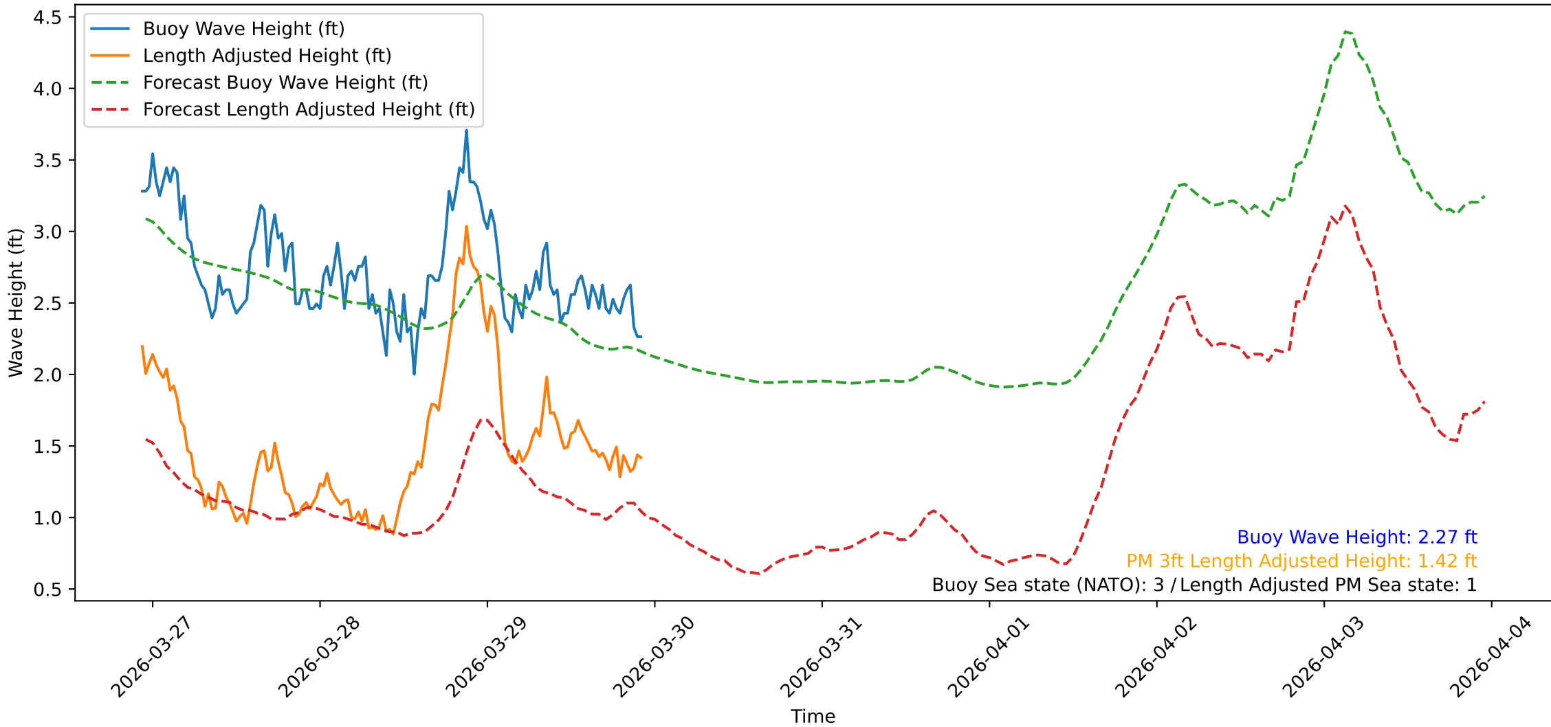
Wave Heights over Time for Green Beach at 2026-03-29 22:41:10
