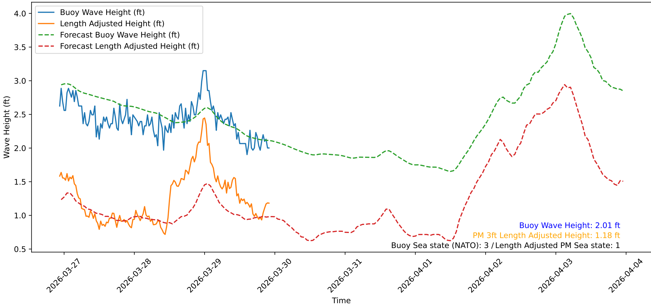
Wave Heights over Time for Oceanside Harbor at 2026-03-29 22:40:31
