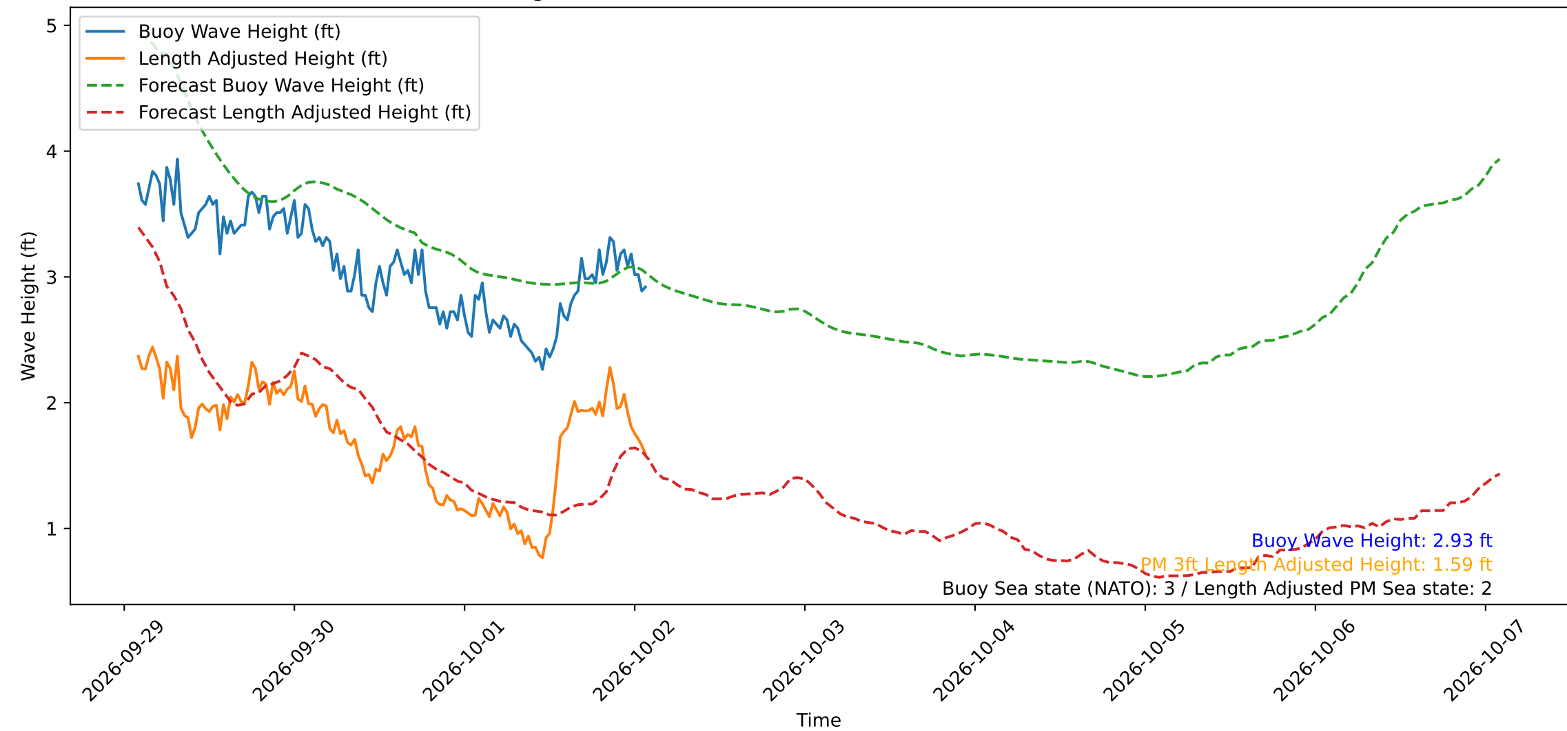
Wave Heights over Time for Oceanside Harbor at 2026-10-02 02:10:29
