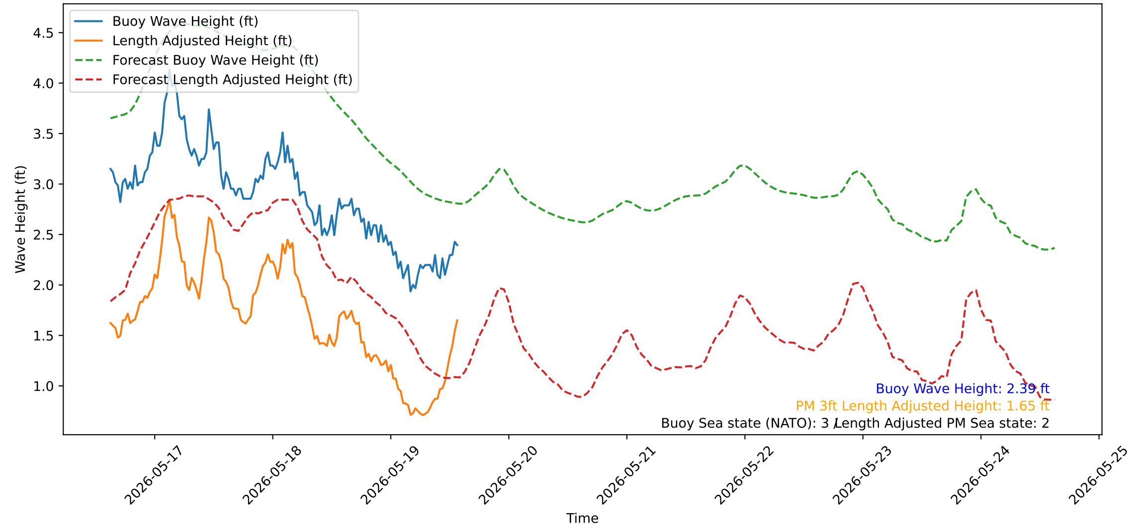
Wave Heights over Time for Red Beach at 2026-05-19 14:50:51
