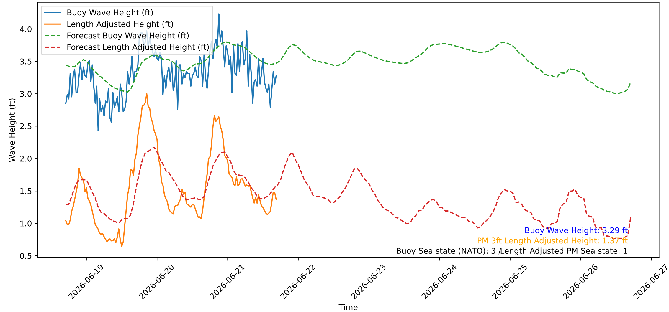
Wave Heights over Time for Green Beach at 2026-06-21 17:11:07
