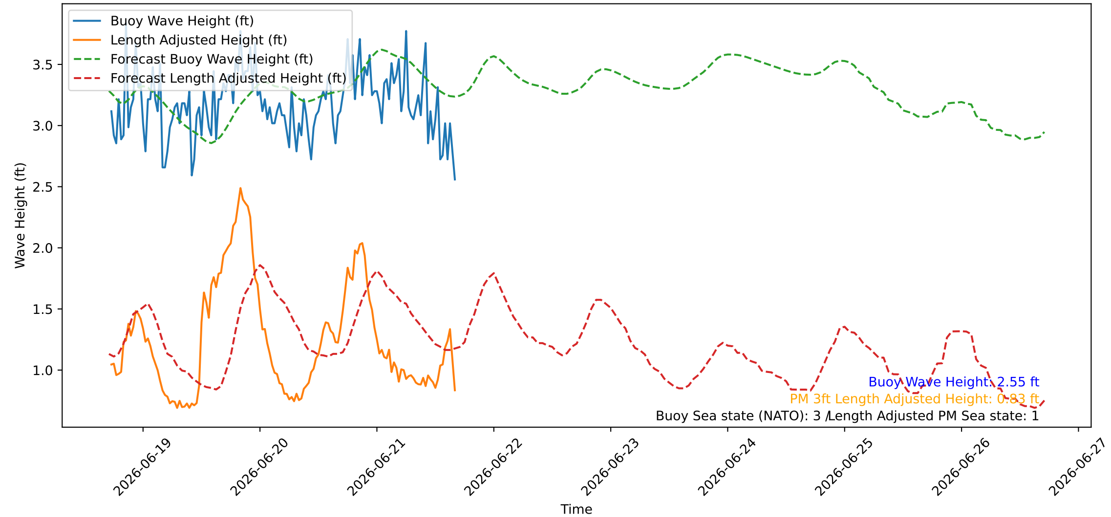
Wave Heights over Time for Red Beach at 2026-06-21 17:10:45
