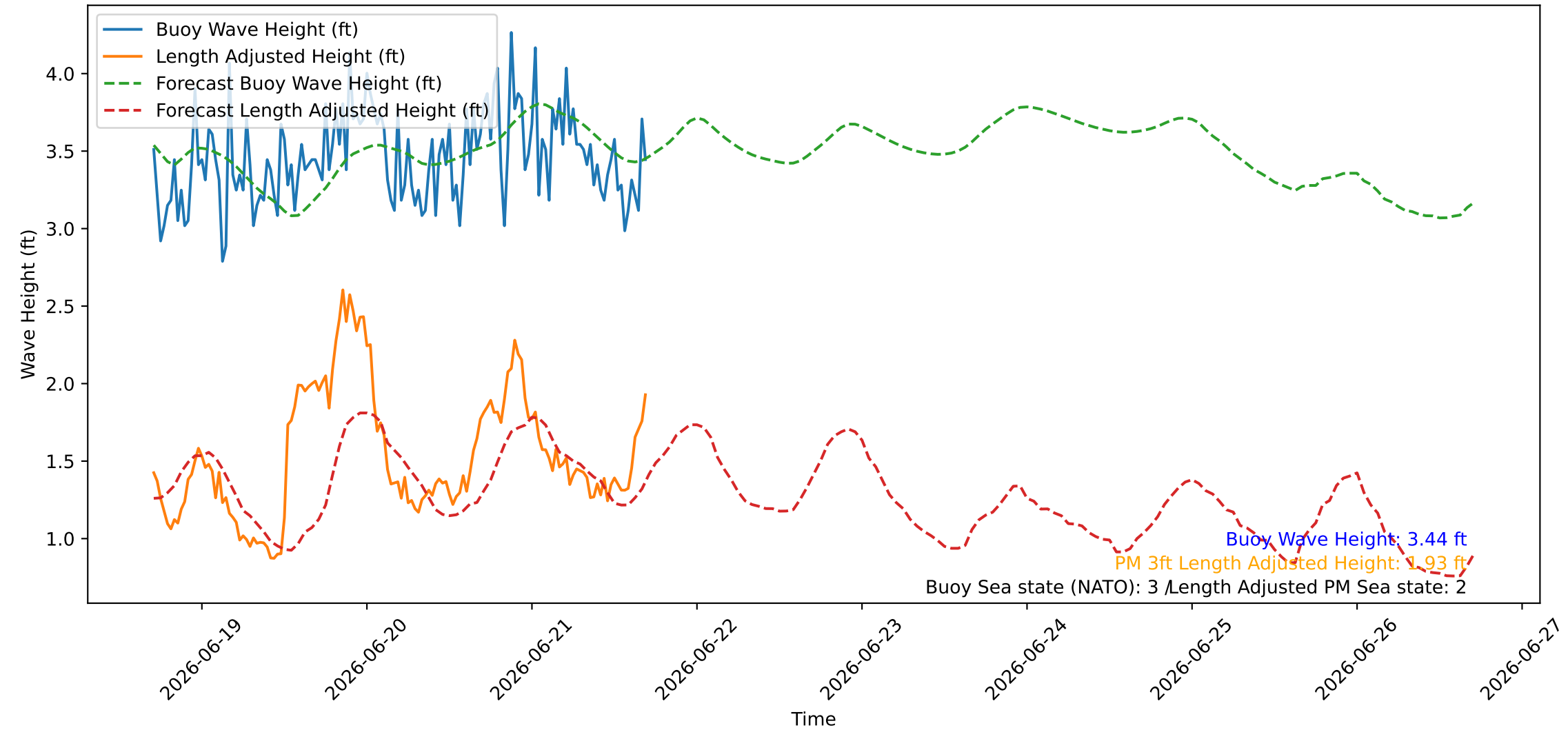
Wave Heights over Time for Oceanside Harbor at 2026-06-21 17:10:25
