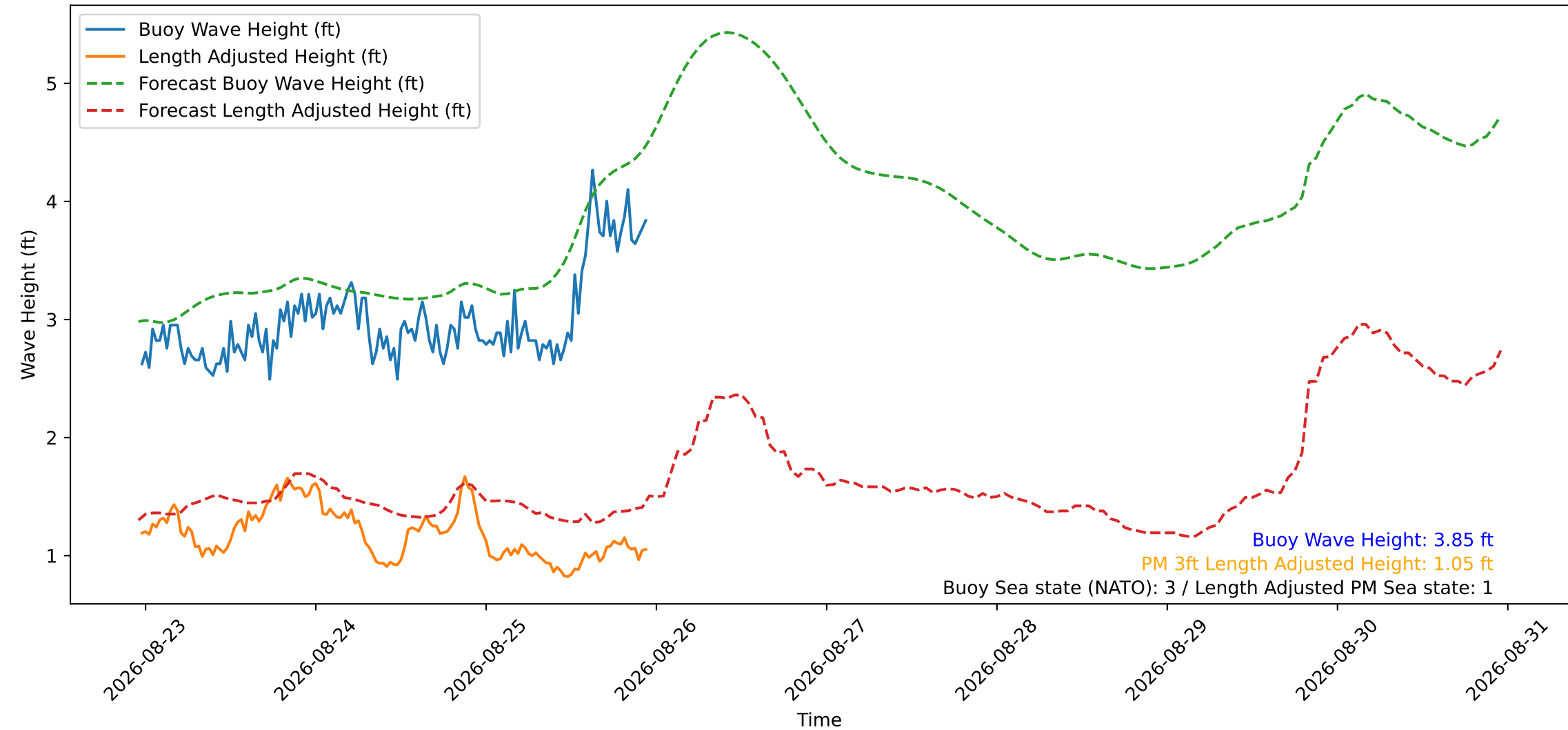
Wave Heights over Time for Green Beach at 2026-08-25 23:11:12
