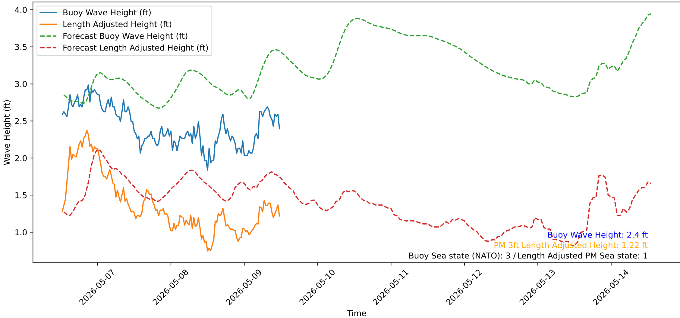
Wave Heights over Time for Green Beach at 2026-05-09 12:31:14
