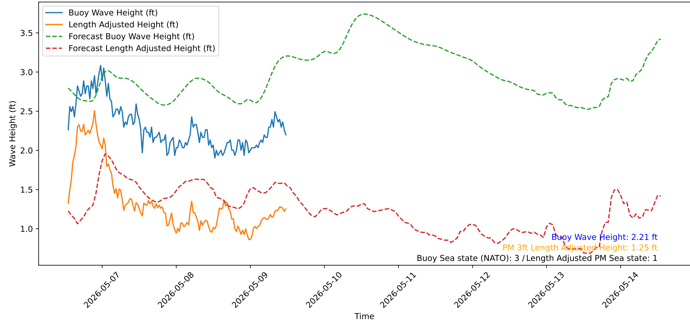
Wave Heights over Time for Red Beach at 2026-05-09 12:30:51
