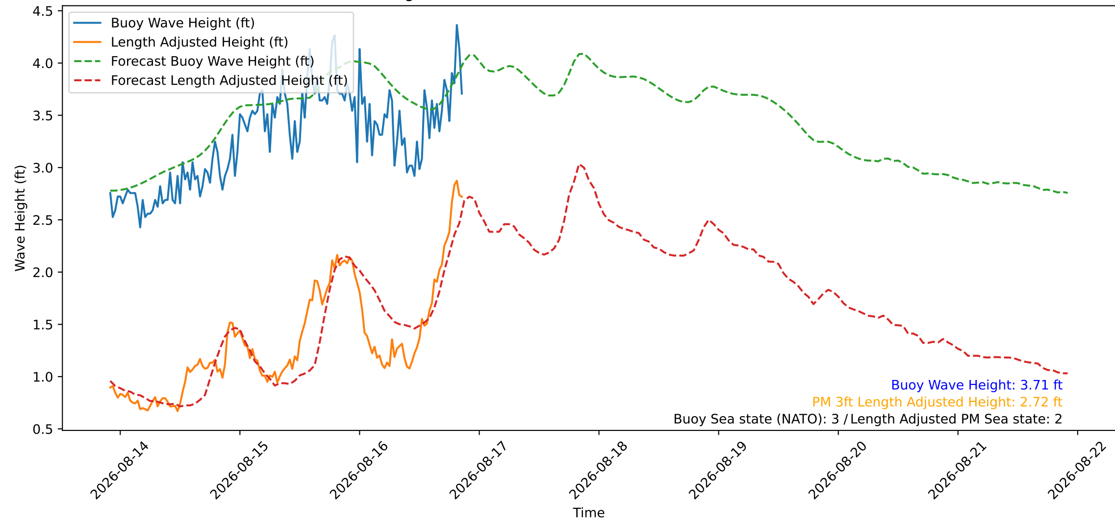
Wave Heights over Time for Green Beach at 2026-08-16 21:31:08
