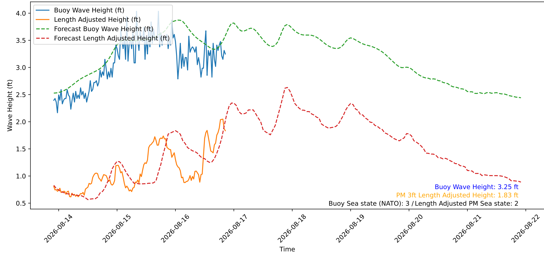
Wave Heights over Time for Red Beach at 2026-08-16 21:30:46
