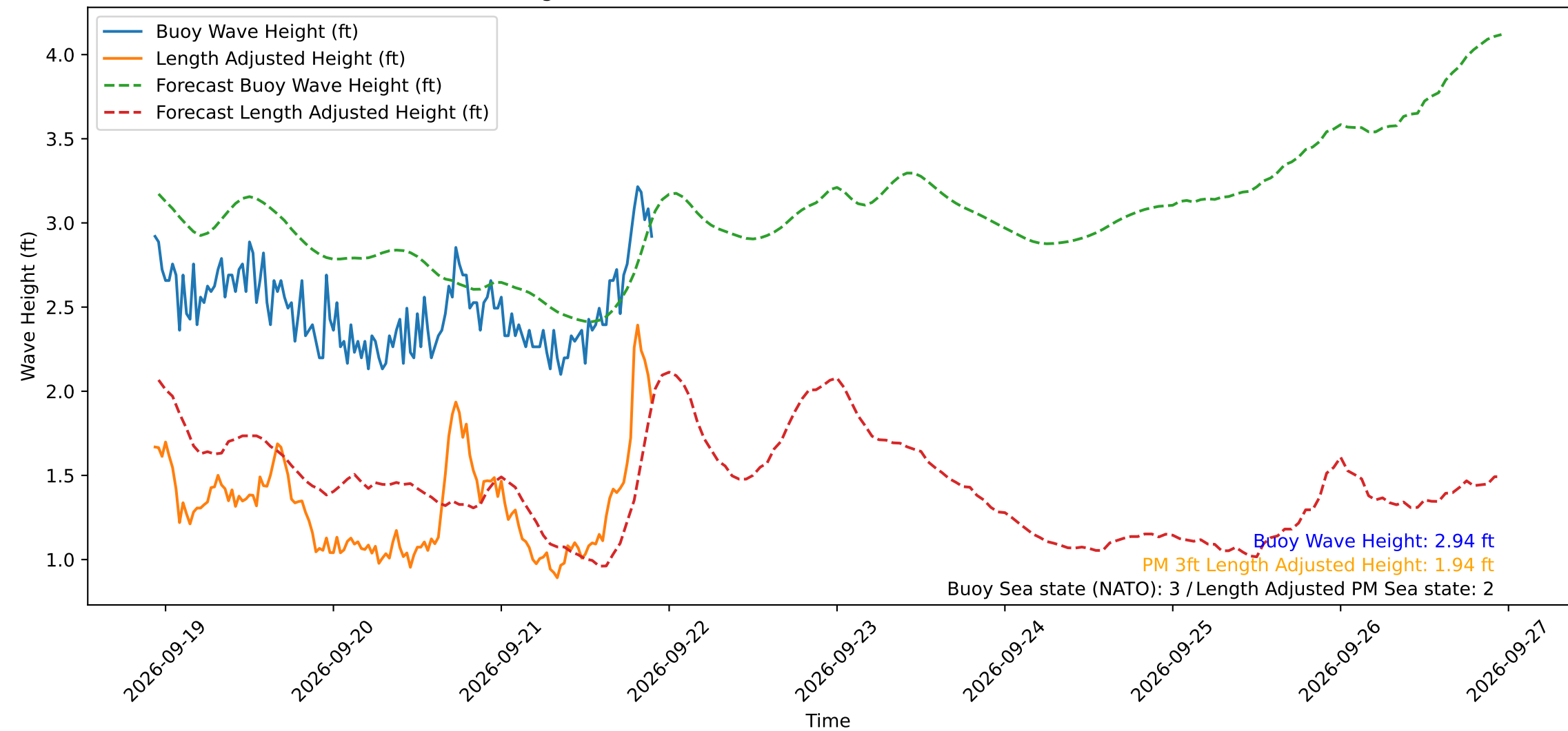
Wave Heights over Time for Oceanside Harbor at 2026-09-21 22:30:31
