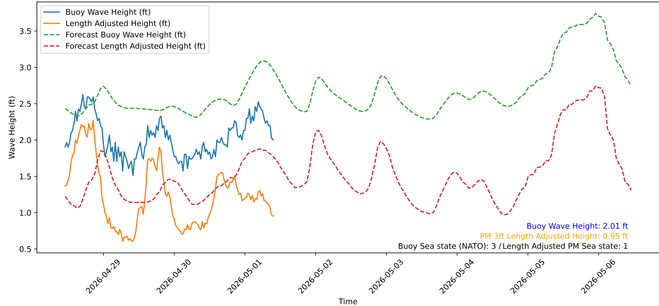
Wave Heights over Time for Red Beach at 2026-05-01 10:30:50
