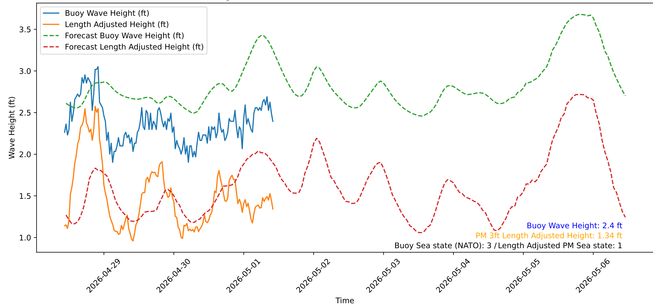
Wave Heights over Time for Oceanside Harbor at 2026-05-01 10:30:31
