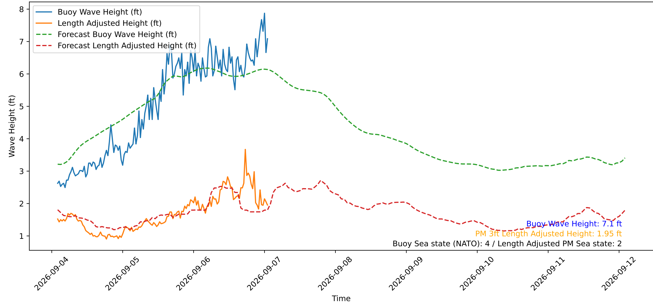
Wave Heights over Time for Green Beach at 2026-09-07 01:41:13
