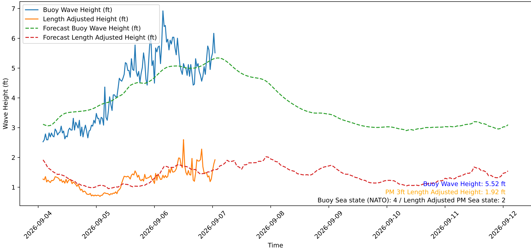
Wave Heights over Time for Red Beach at 2026-09-07 01:40:51
