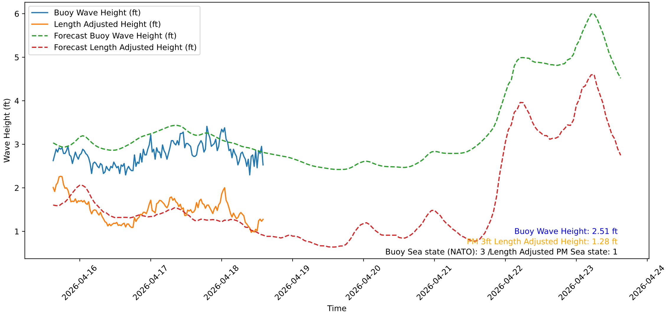
Wave Heights over Time for Oceanside Harbor at 2026-04-18 14:50:31
