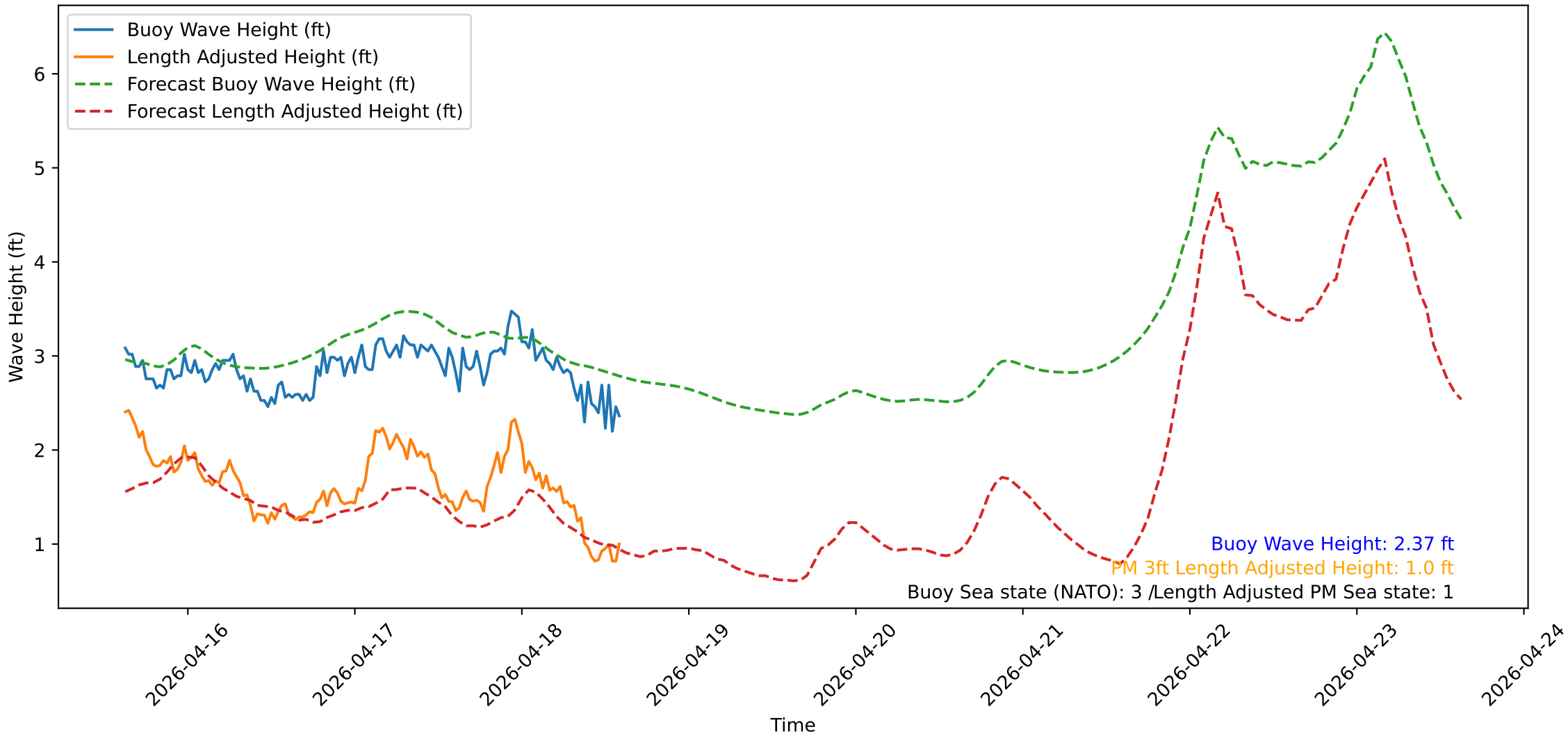
Wave Heights over Time for Green Beach at 2026-04-18 14:51:13
