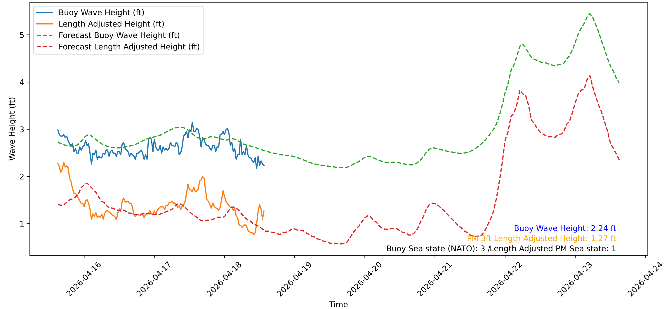
Wave Heights over Time for Red Beach at 2026-04-18 14:50:51
